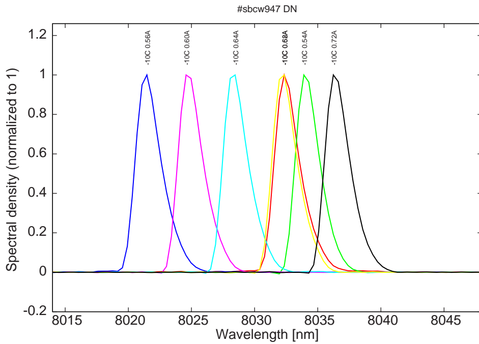
Figure 9: spectra at -10C for various DC currents (monomode range, but with mode jumping for currents higher than 0.54A)
