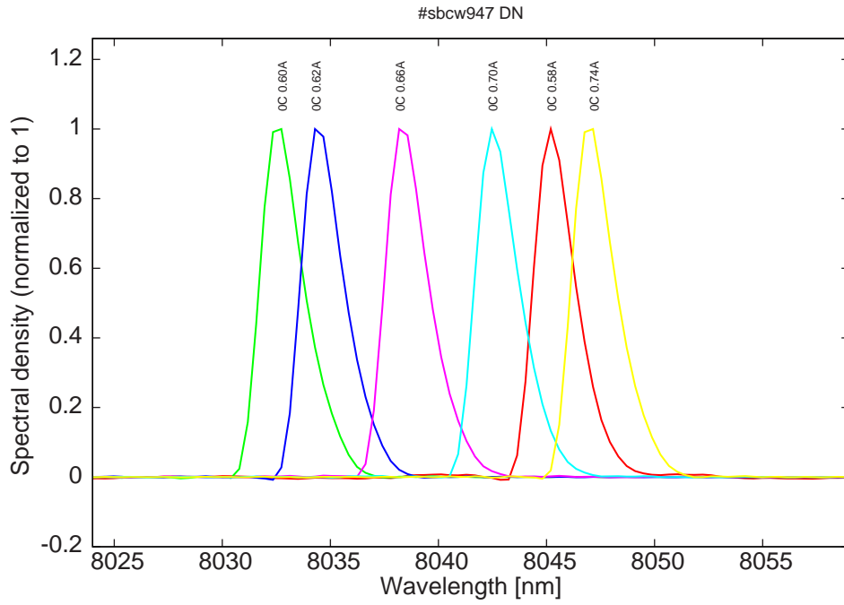
Figure 10: spectra at 0C for various DC currents (monomode range, but with mode jumping for current higher than 0.58A)
