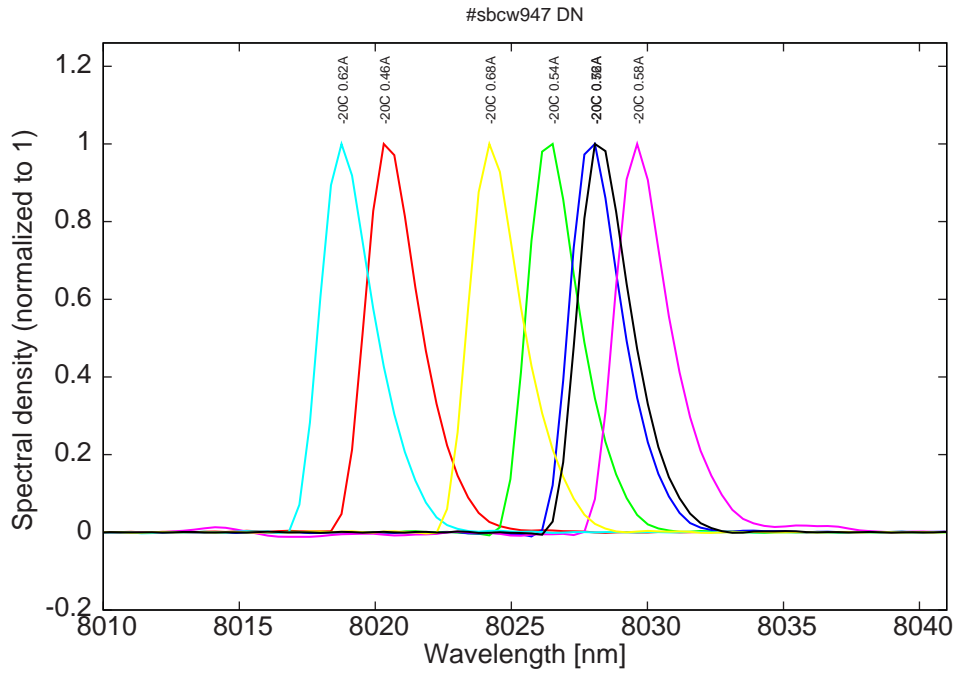
Figure 8: spectra at -20C for various DC currents (monomode range, but with mode jumping for currents higher than 0.58A)
