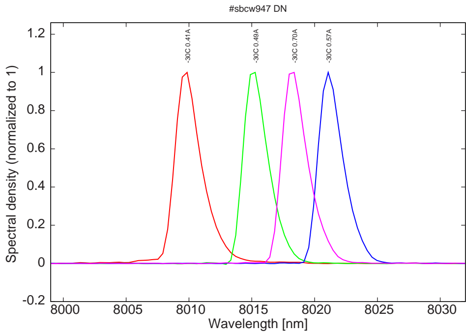
Figure 7: spectra at -30C for various DC currents (monomode range, but with mode jumping for currents higher than 0.61A)
