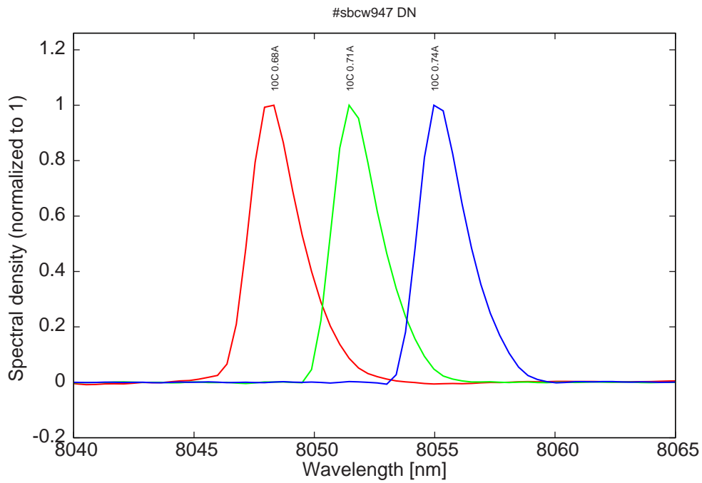
Figure 11: spectra at 10C for various DC currents (same mode compared to high current spectra at 0C)
