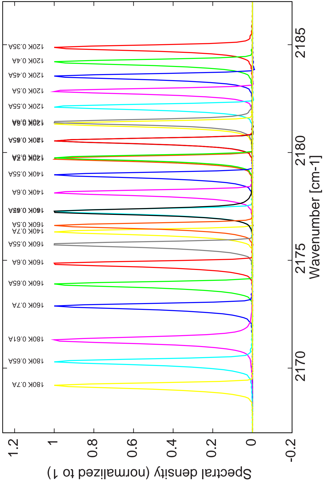
Figure 10: spectra between 120K and 180K (all monomode)
