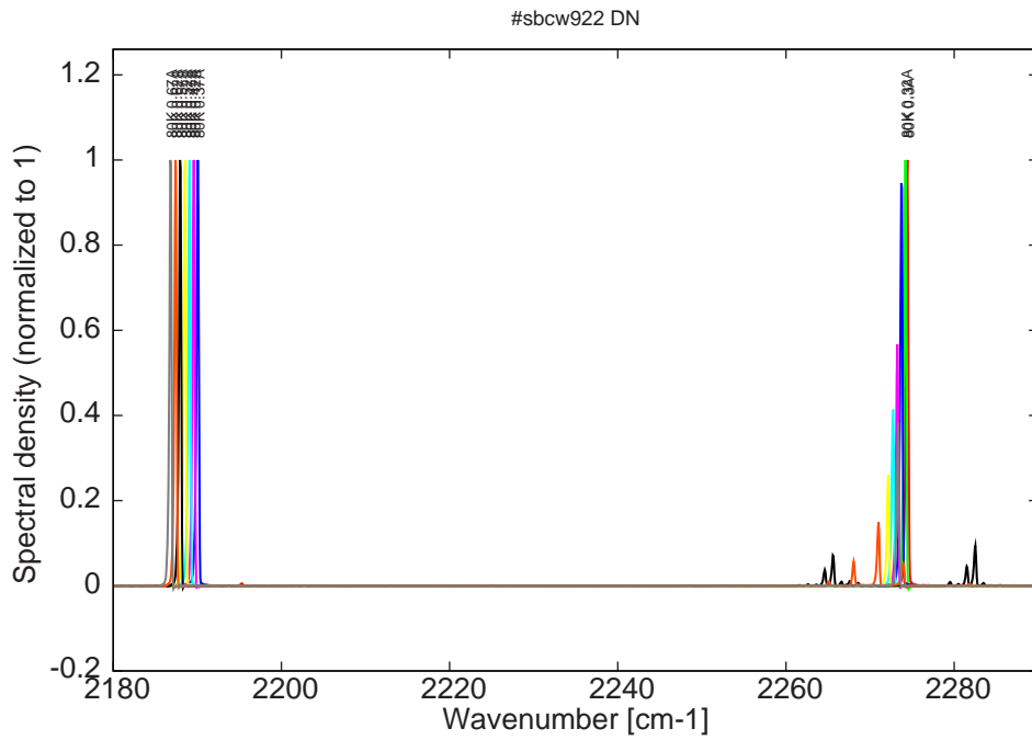
Figure 6: spectra at 80K (monomode up to 0.32A but around 2274cm-1)
