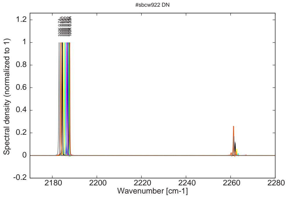
Figure 9: spectra at 100K (monomode up to 0.45Å)
