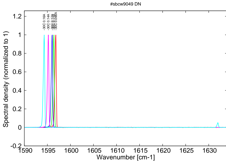
Figure 6: spectra at -30C for various DC currents (monomode up to 0.14A, then becomes bimode)
