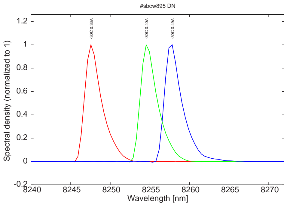
Figure 7: spectra at -30C for various DC currents (monomode range, but with mode jumping for spectrum at 0.49A)
