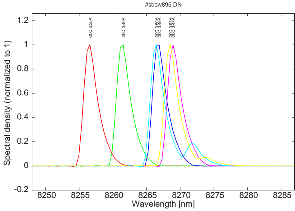
Figure 8: spectra at -20C for various DC currents
