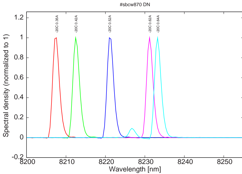
Figure 9: spectra at -20C for various DC currents
