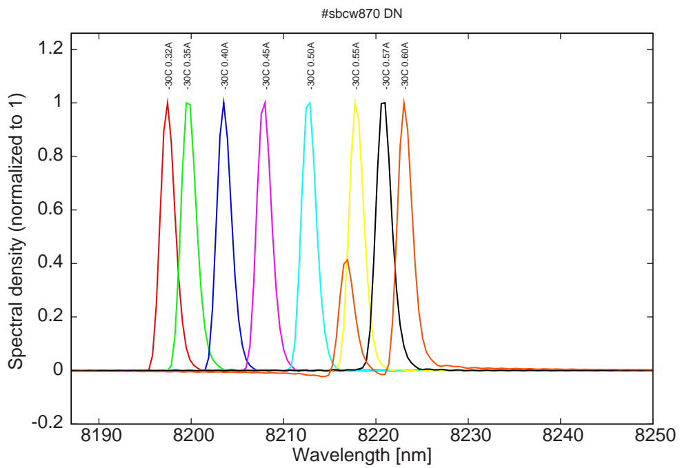
Figure 7: spectra at -30C for various DC currents
