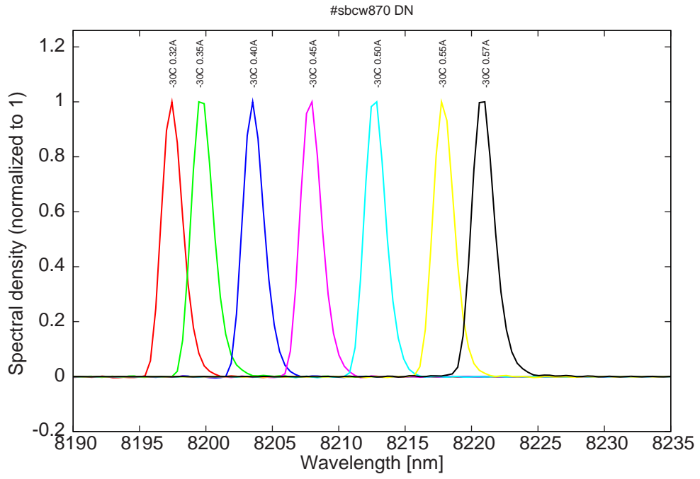
Figure 8: spectra at -30C for various DC currents (monomode range)
