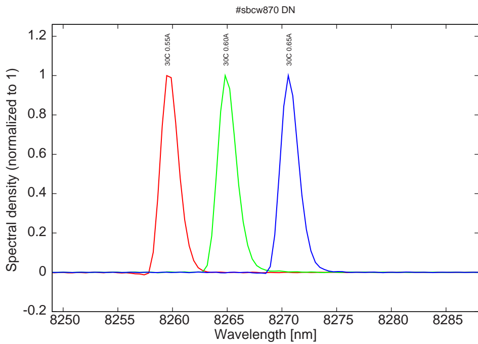
Figure 15: spectra at 30C for various DC currents
