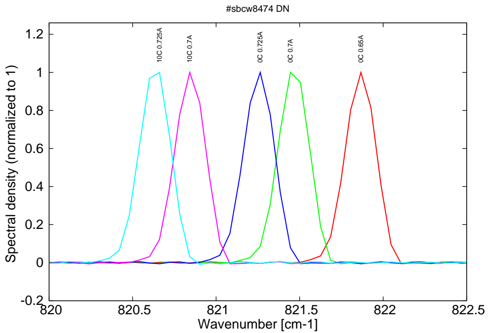
Figure 6: spectra between 0C and 10C for various DC currents (all monomode on mode 2, see Fig. 2 & 3)
