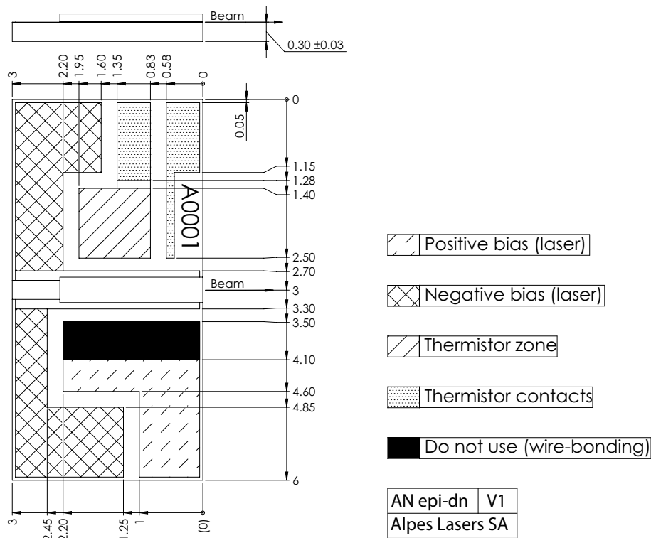
Figure 1: Support mounting for #sbcw8474 DN (please note that AlN submount numbering is A02KL)
