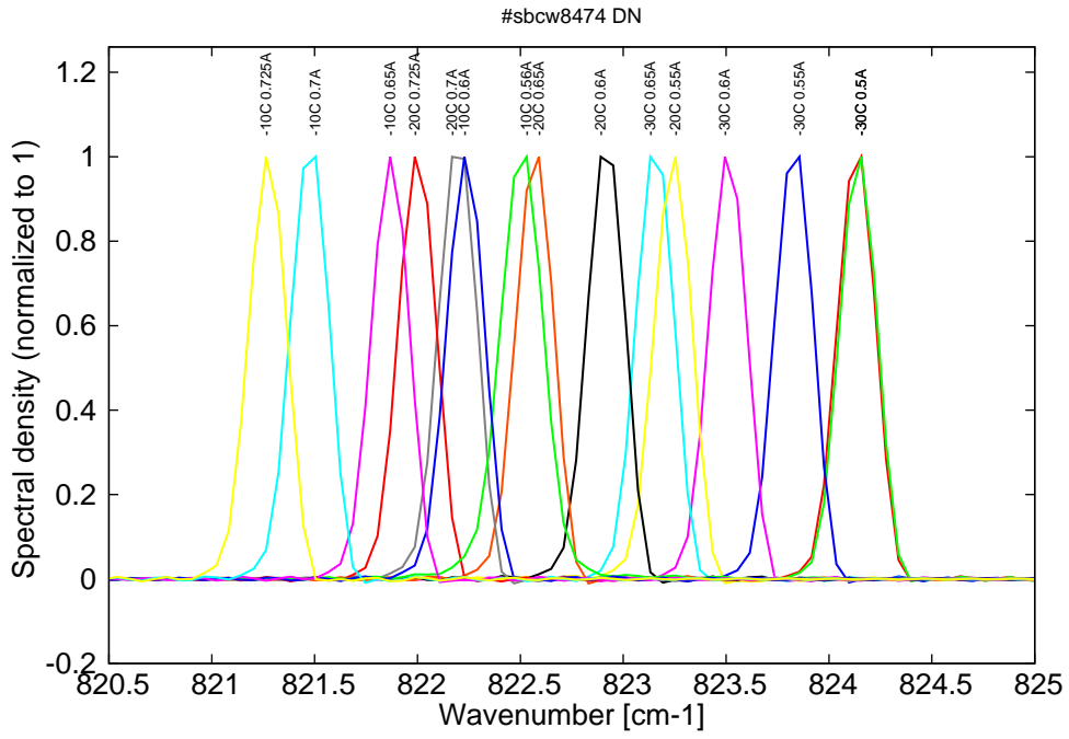
Figure 5: spectra between -30C and -10C for various DC currents (all monomode on mode 1, see Fig. 2 & 3)
