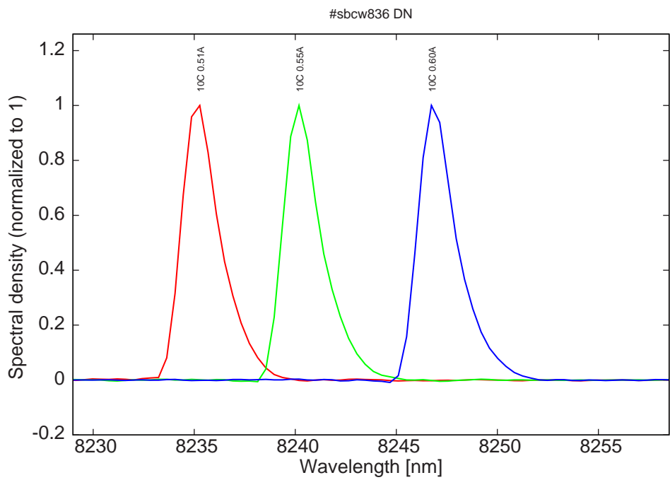
Figure 14: spectra at 10C for various DC currents
