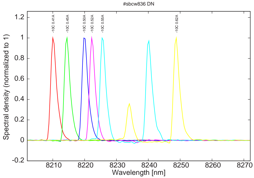
Figure 11: spectra at -10C for various DC currents (monomode up to 0.52A)
