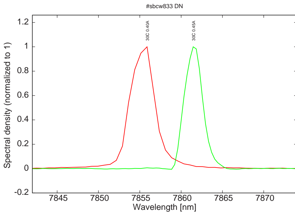
Figure 20: spectra at 30C for various DC currents
