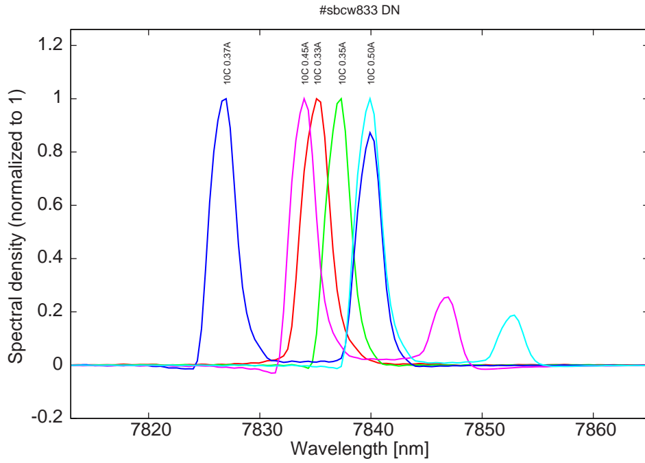
Figure 15: spectra at 10C for various DC currents
