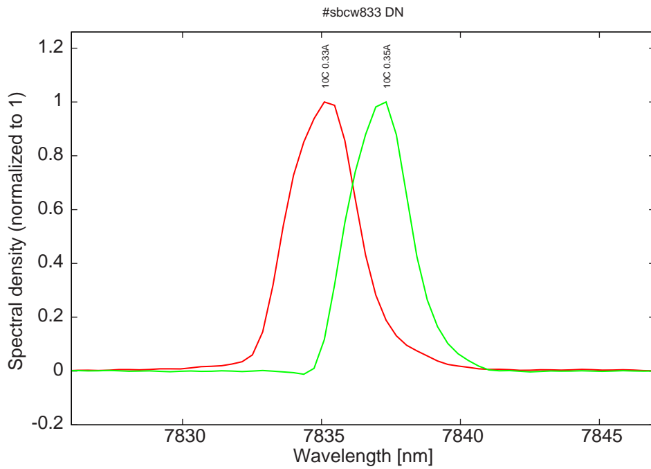
Figure 16: spectra at 10C for various DC currents
