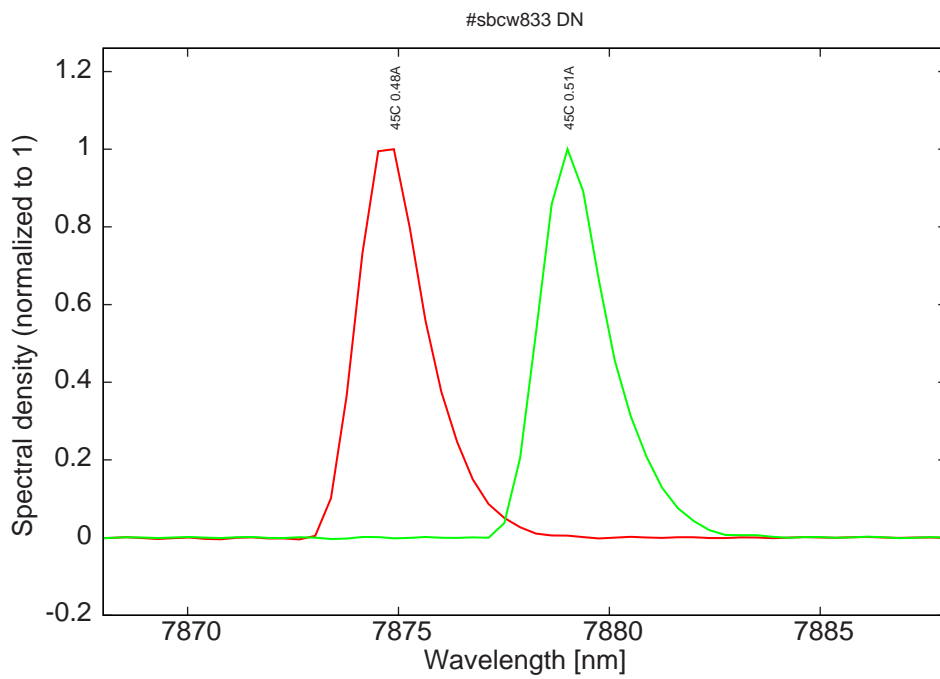
Figure 22: spectra at 45C for various DC currents
