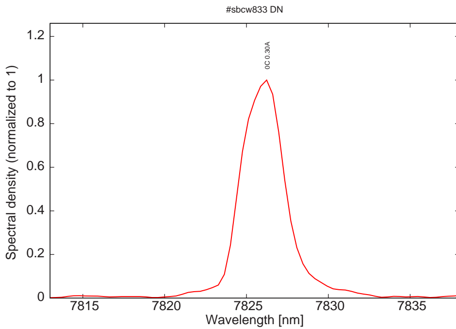
Figure 14: monomode spectrum at 0C and 0.30A on ILX
