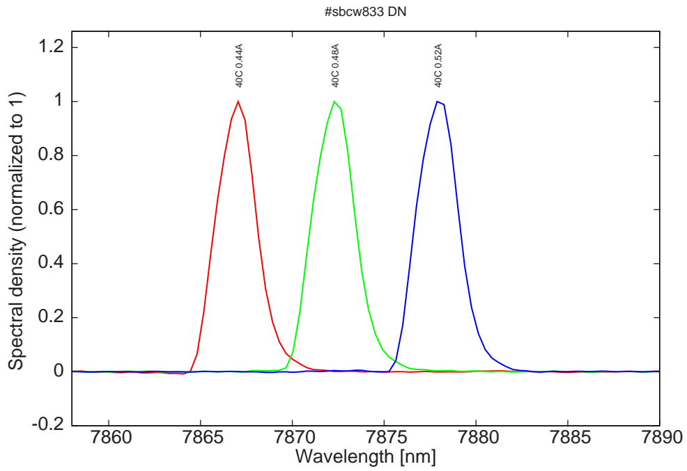
Figure 21: spectra at 40C for various DC currents
