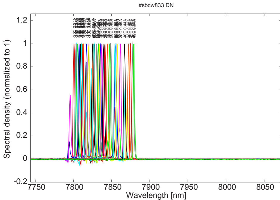
Figure 6: spectra at -30C, -20C, -10C, 0C, 10C, 20C, 30C, 40C and 45C for various DC currents
