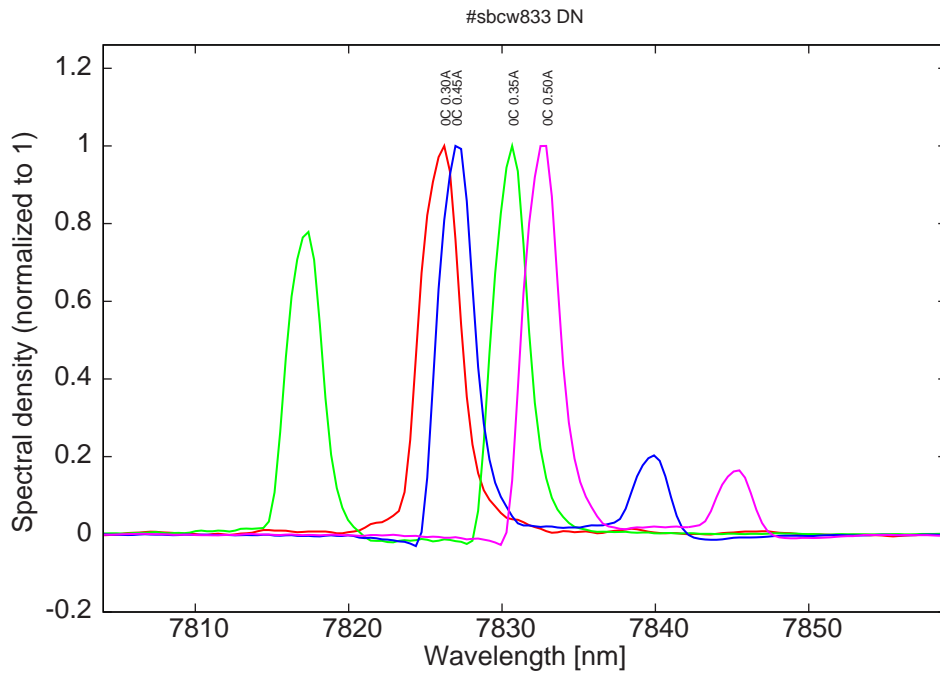
Figure 13: spectra at 0C for various DC currents
