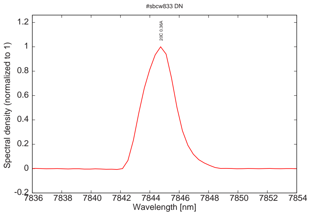
Figure 18: monomode spectrum at 20C and 0.36A on ILX
