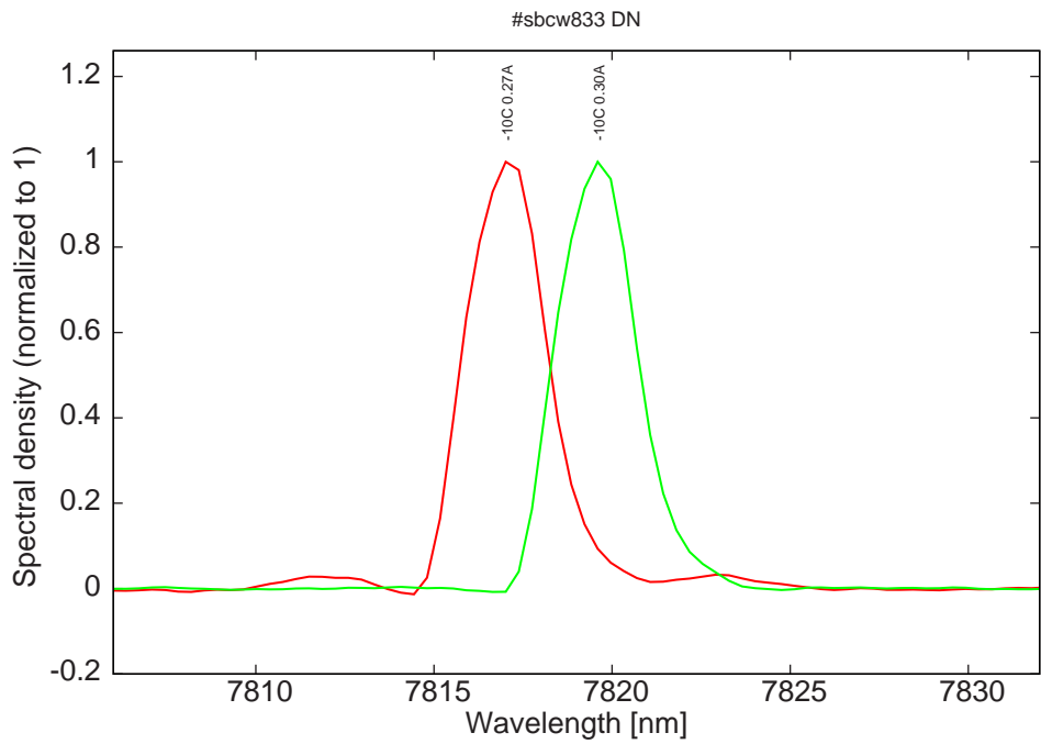
Figure 12: spectra at -10C for various DC currents (monomode range)
