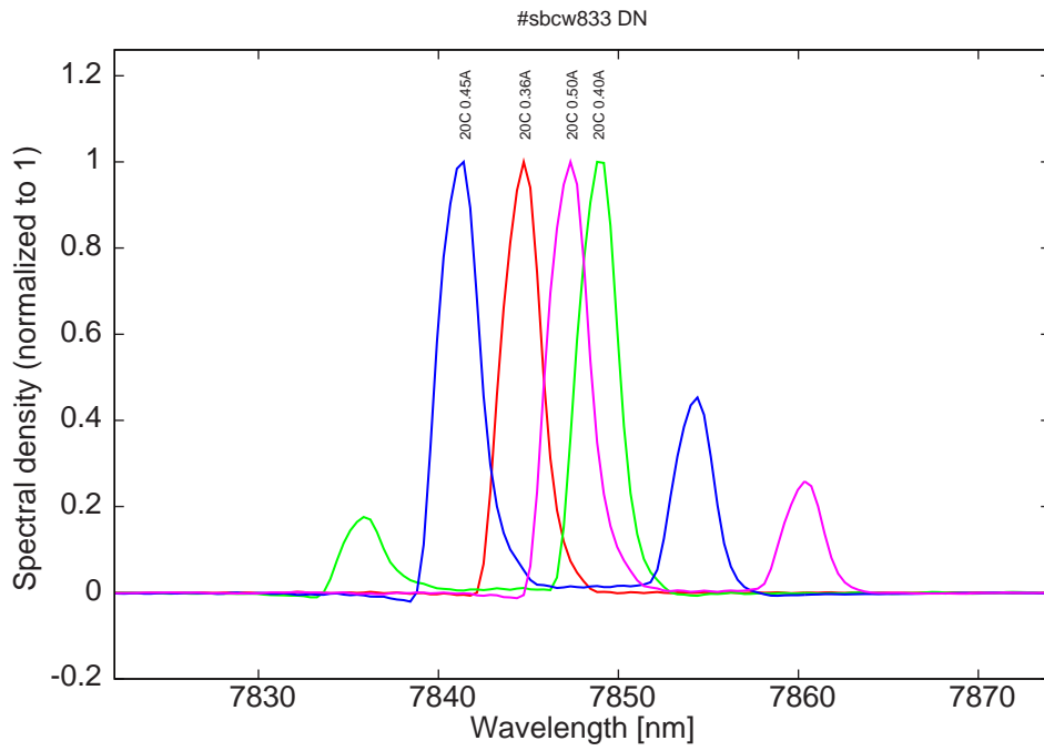
Figure 17: spectra at 20C for various DC currents
