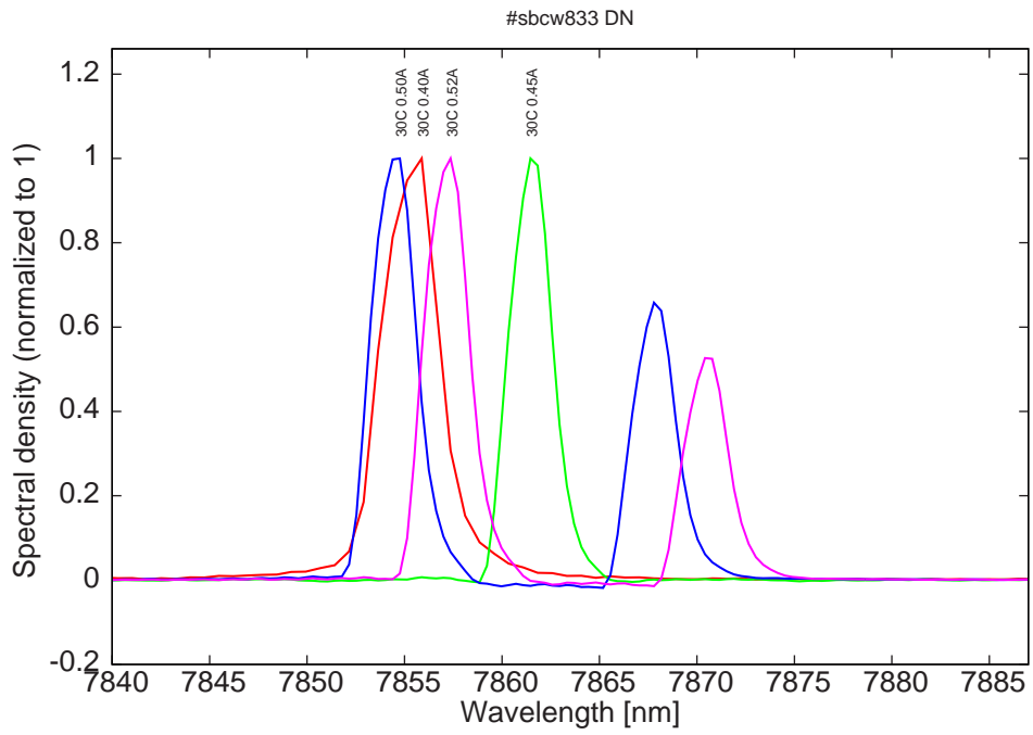
Figure 19: spectra at 30C for various DC currents
