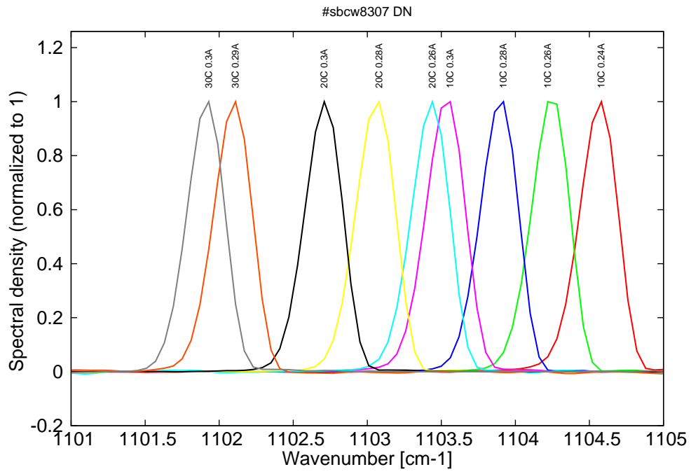
Figure 14: spectra between 10C and 30C for various DC currents (all monomode on mode 2)
