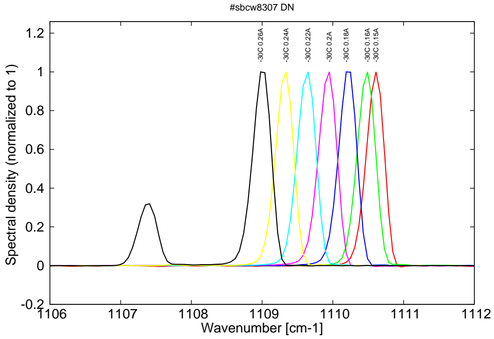
Figure 6: spectra at -30C for various DC currents (monomode on mode 1 up to 0.24A, then becomes bimode)
