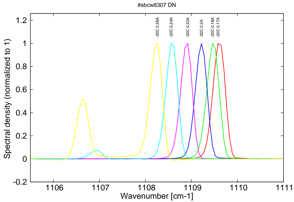
Figure 8: spectra at -20C for various DC currents (monomode on mode 1 up to 0.22A, then becomes bimode)
