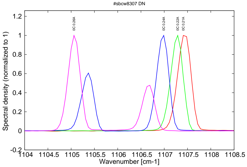
Figure 12: spectra at 0C for various DC currents (monomode on mode 1 up to 0.22A, then becomes bimode)
