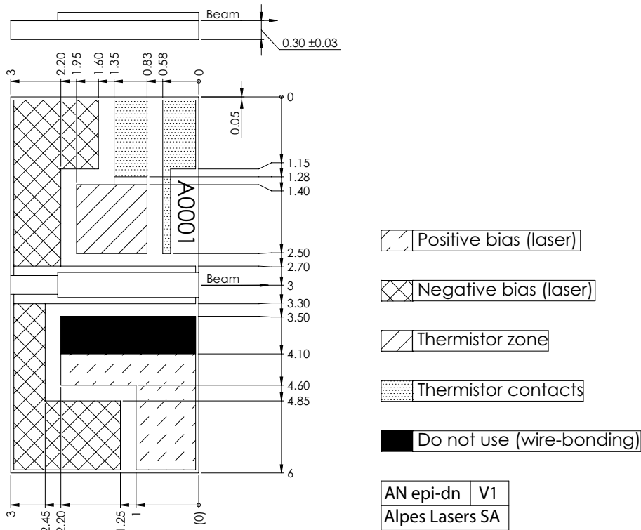
Figure 1: Support mounting for #sbcw8307 DN (please note that AlN submount numbering is A02AL)
