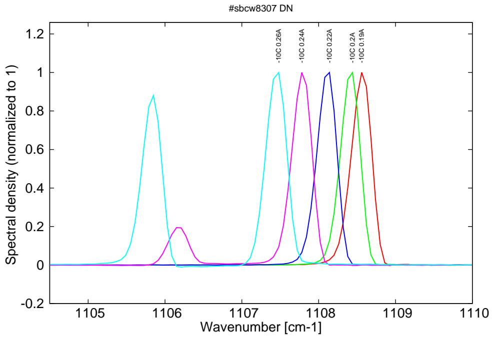
Figure 10: spectra at -10C for various DC currents (monomode on mode 1 up to 0.22A, then becomes bimode)
