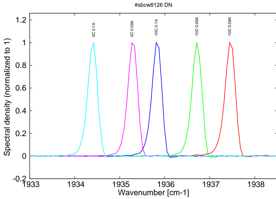
Figure 10: spectra -10C and 0C for various DC currents (all monomode)
