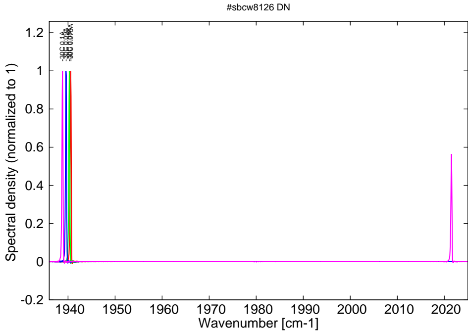
Figure 6: spectra at -30C for various DC currents (monomode up to 0.09A, then becomes bimode)
