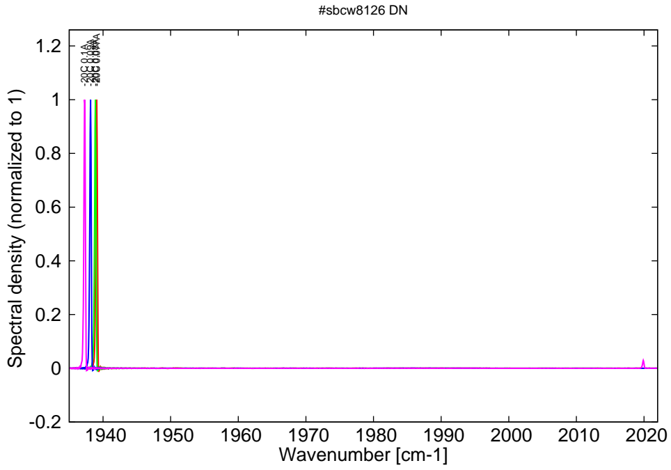
Figure 8: spectra at -20C for various DC currents (monomode up to 0.09A, then becomes bimode)
