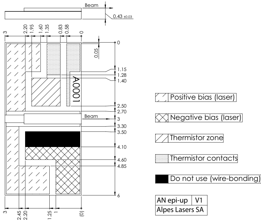
Figure 1: Support mounting for #sbcw7736 DN (please note that AlN submount numbering is A006J)
