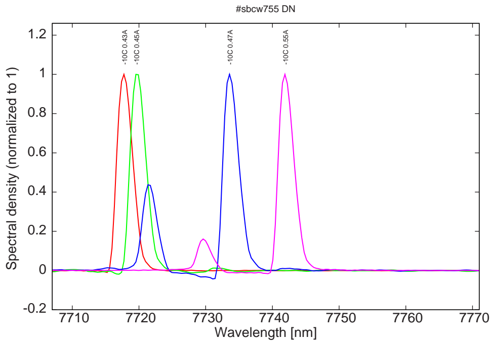
Figure 10: spectra at -10C for various DC currents (monomode just at threshold)
