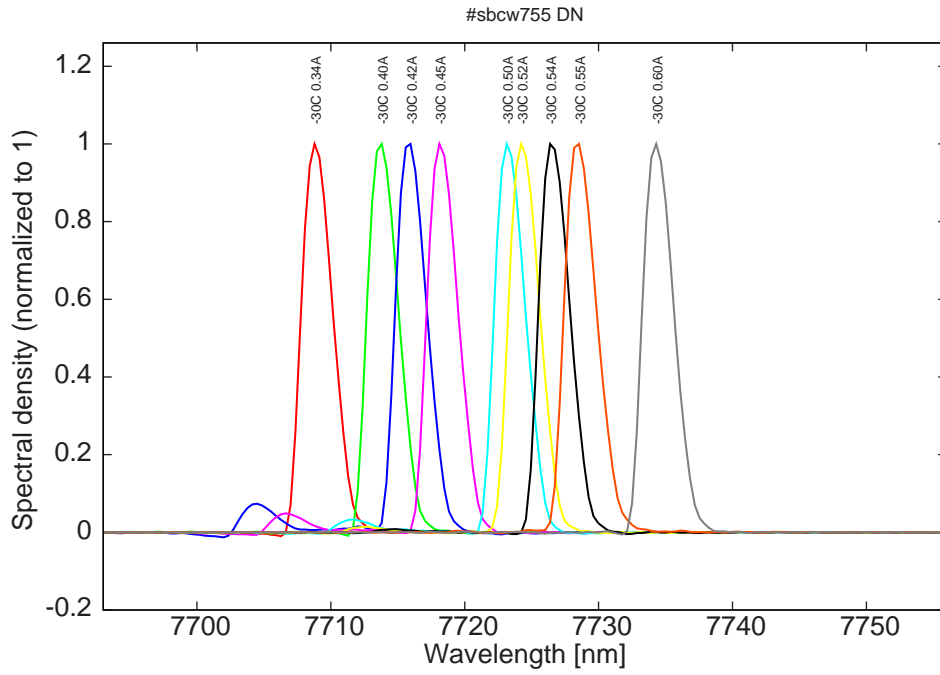
Figure 7: spectra at -30C for various DC currents (mode jumping compared to monomode spectra at -20C, -10C, 0C and 10C)
