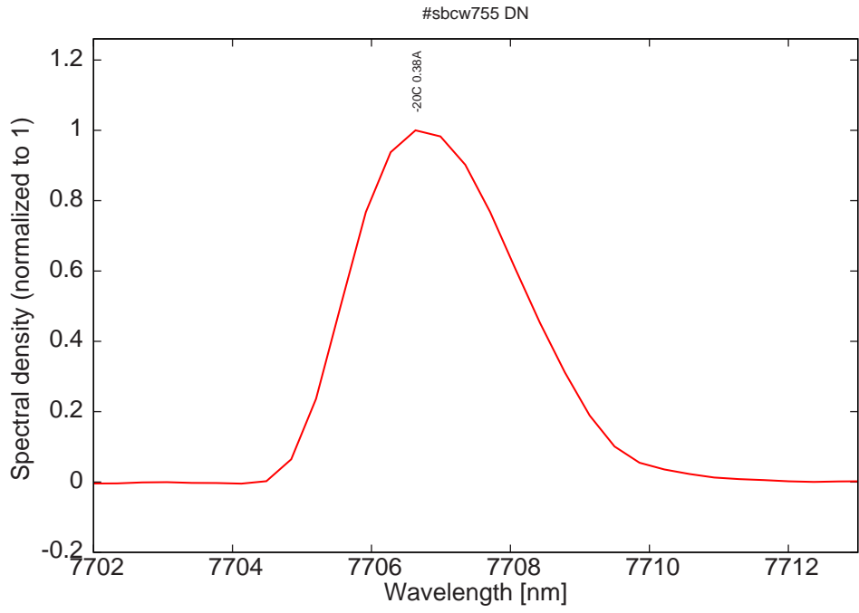
Figure 9: monomode spectrum at -20C and 0.38A
