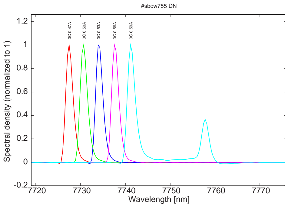
Figure 12: spectra at 0C for various DC currents (monomode up to 0.56A)
