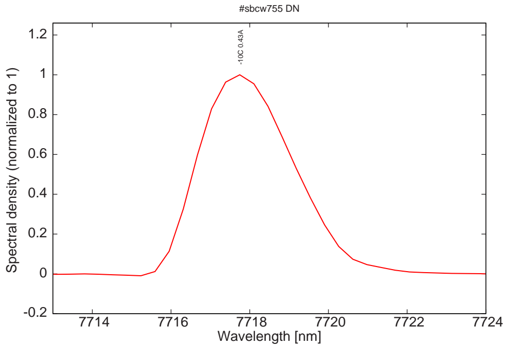
Figure 11: monomode spectrum at -10C and 0.43A
