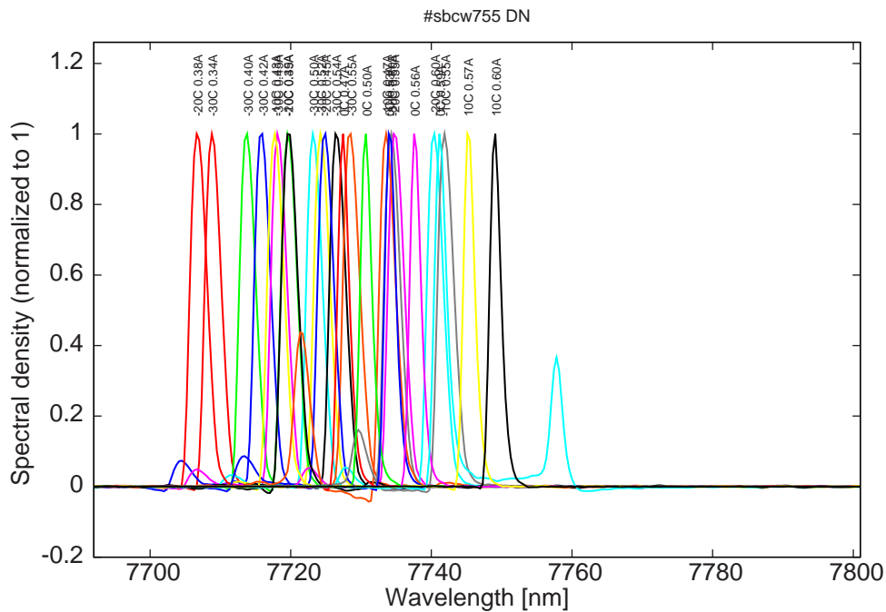
Figure 6: spectra at -30C, -20C, -10C, 0C and 10C for various DC currents
