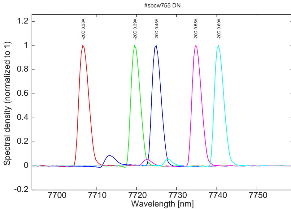
Figure 8: spectra at -20C for various DC currents (monomode just at threshold, mode jumping when current is greater than 0.38A )
