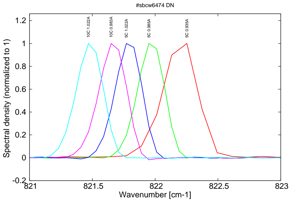
Figure 6: spectra between 5C and 10C for various DC currents (all monomode on mode 2, see Fig. 2 & 3)
