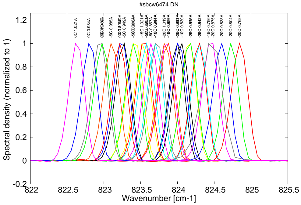
Figure 5: spectra between -20C and 0C for various DC currents (all monomode on mode 1, see Fig. 2 & 3)
