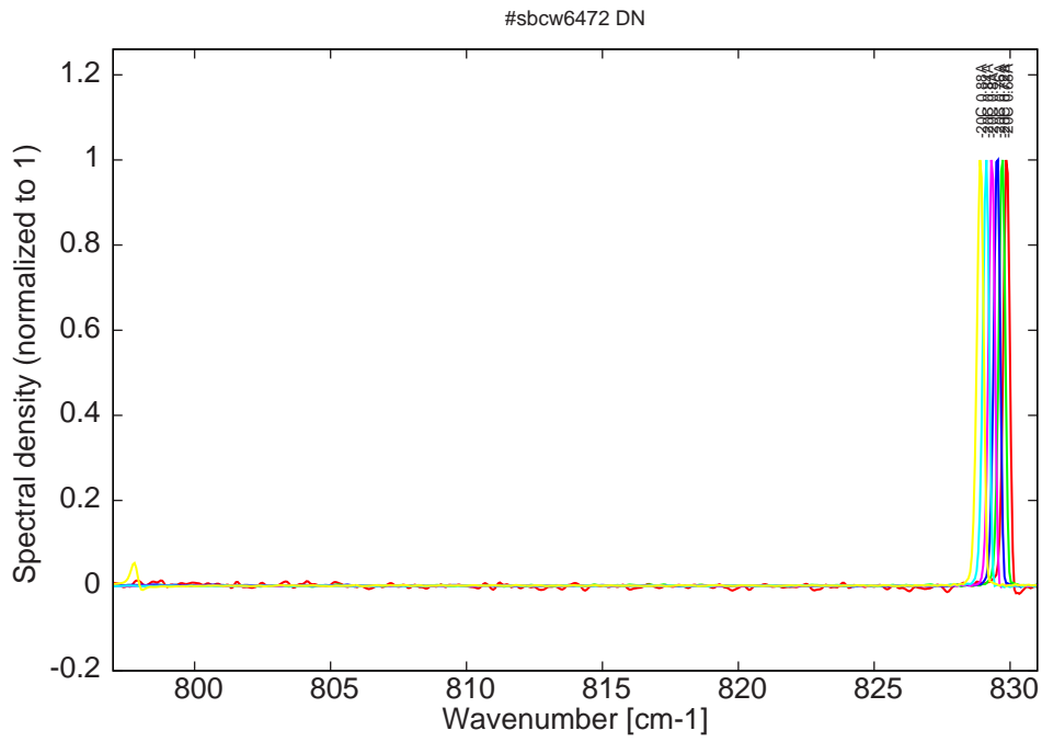
Figure 8: spectra at -20C for various DC currents (monomode up to 0.84A, then becomes bimode)
