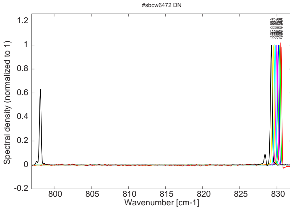
Figure 6: spectra at -30C for various DC currents (monomode up to 0.84A, then becomes bimode)
