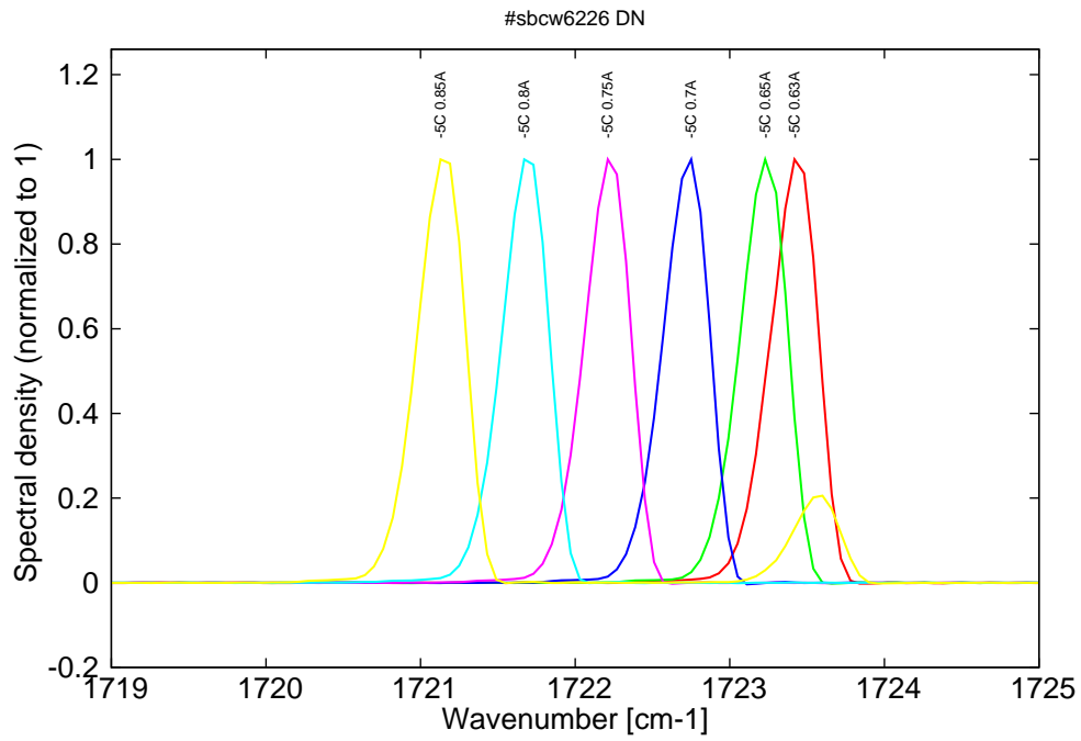
Figure 12: spectra at -5C for various DC currents (monomode up to 0.80A, then becomes bimode)
