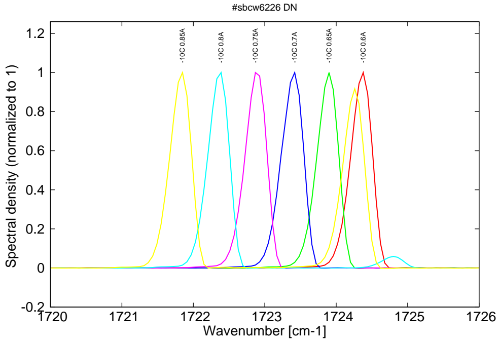
Figure 10: spectra at -10C for various DC currents (monomode up to 0.75A, then becomes bimode)
