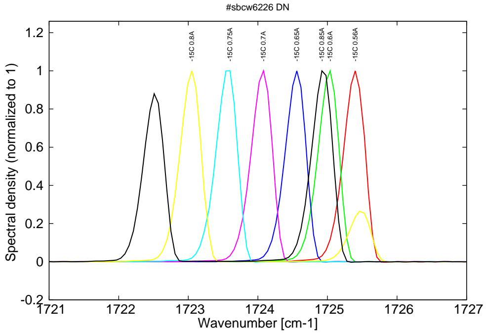
Figure 8: spectra at -15C for various DC currents (monomode up to 0.75A, then becomes bimode)
