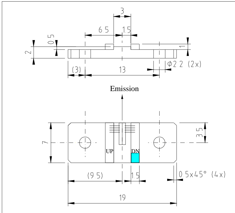
Figure 1: Support mounting for #sbcw6226 DN (please note that the laser is connected to the DN pad drawn in blue)
