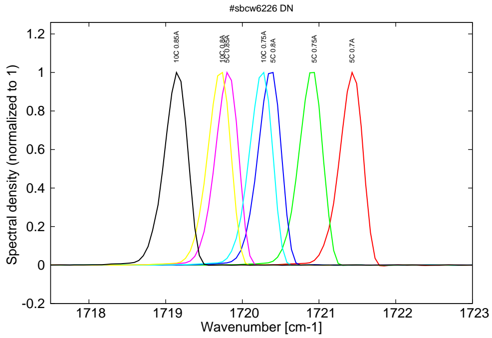
Figure 14: spectra between 0C and 10C for various DC currents (all monomode)
