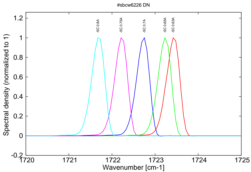
Figure 13: spectra at -5C for various DC currents (monomode range)
