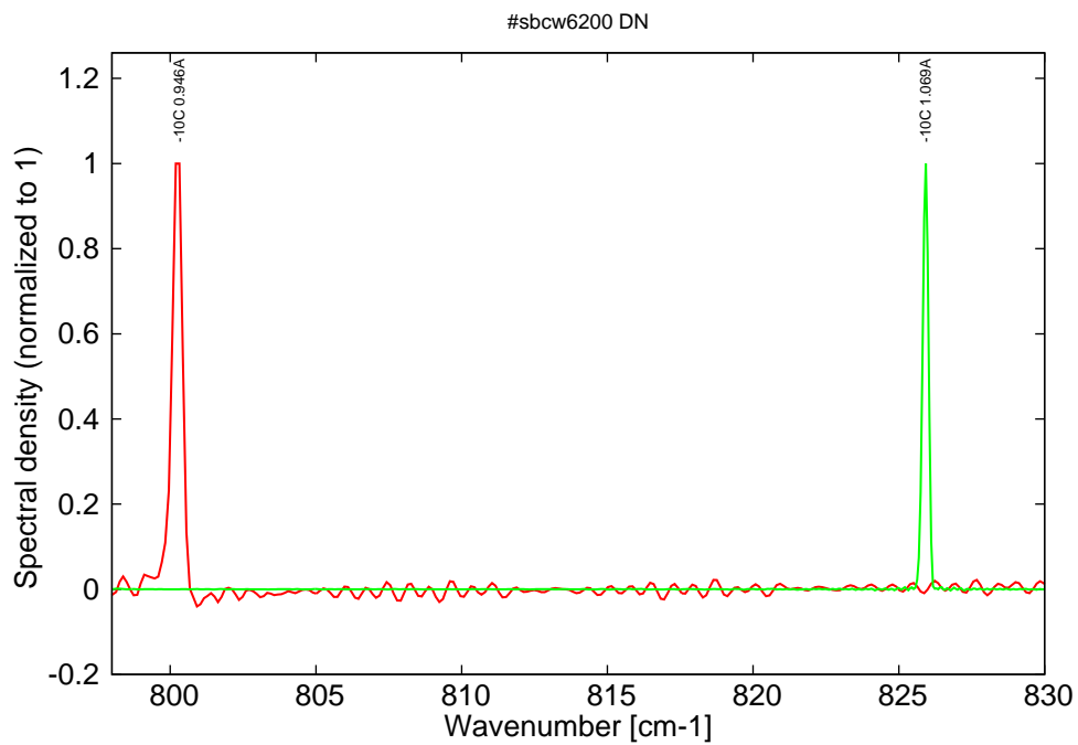
Figure 7: spectra at -10C for various DC currents (monomode on mode 1 up to 0.95A, then becomes monomode on mode 2)
