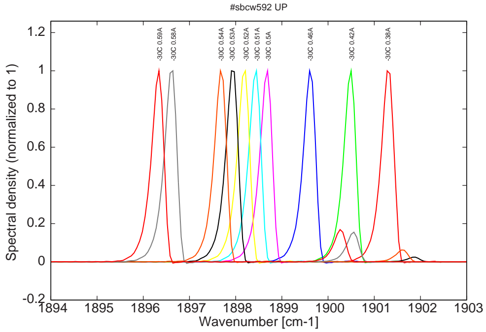
Figure 6: spectra at -30C for various DC currents (become bimode for I > 0.52A )
