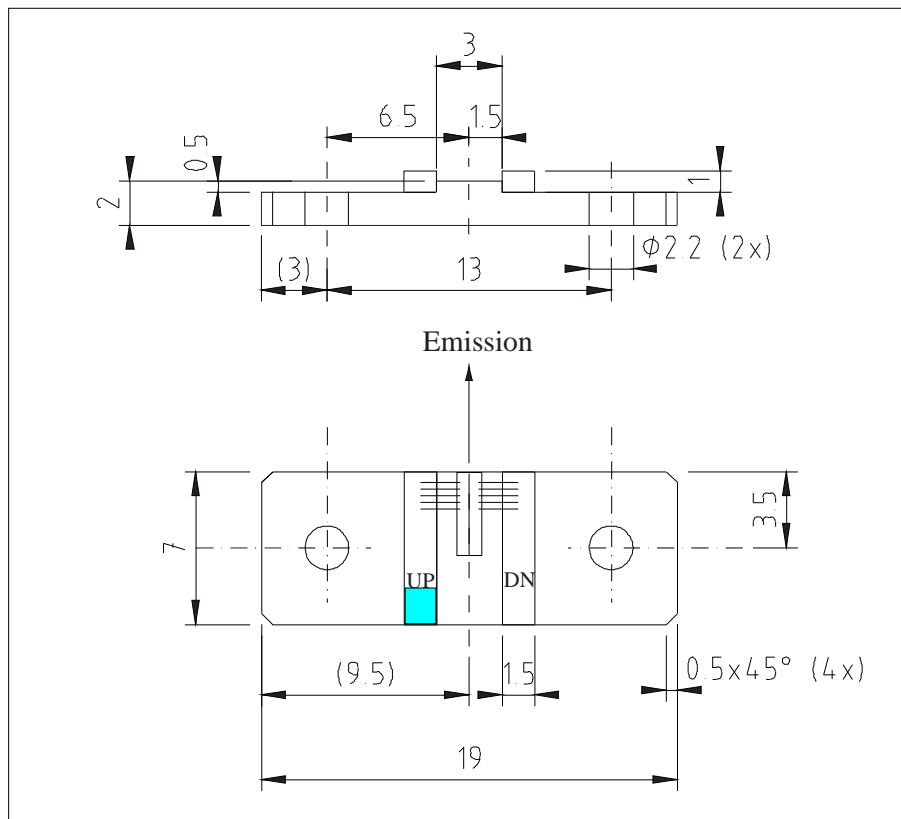
Figure 1: Support mounting for #sbcw564 UP (please note that the laser is connected to the UP pad drawn in blue)
