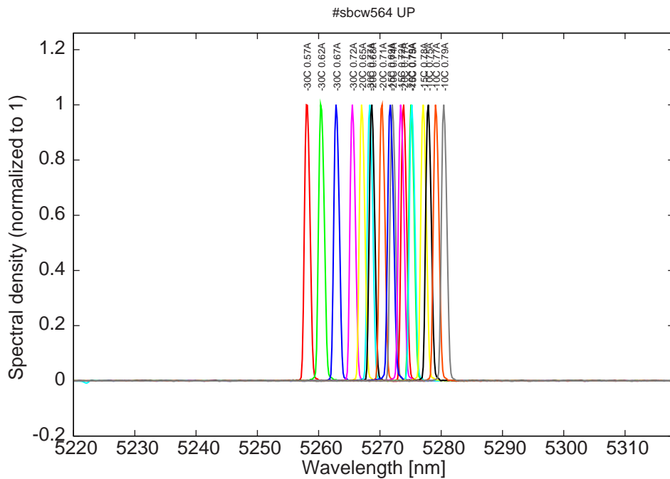
Figure 6: spectra at -30C, -20C, -15C and -10C for various DC currents
