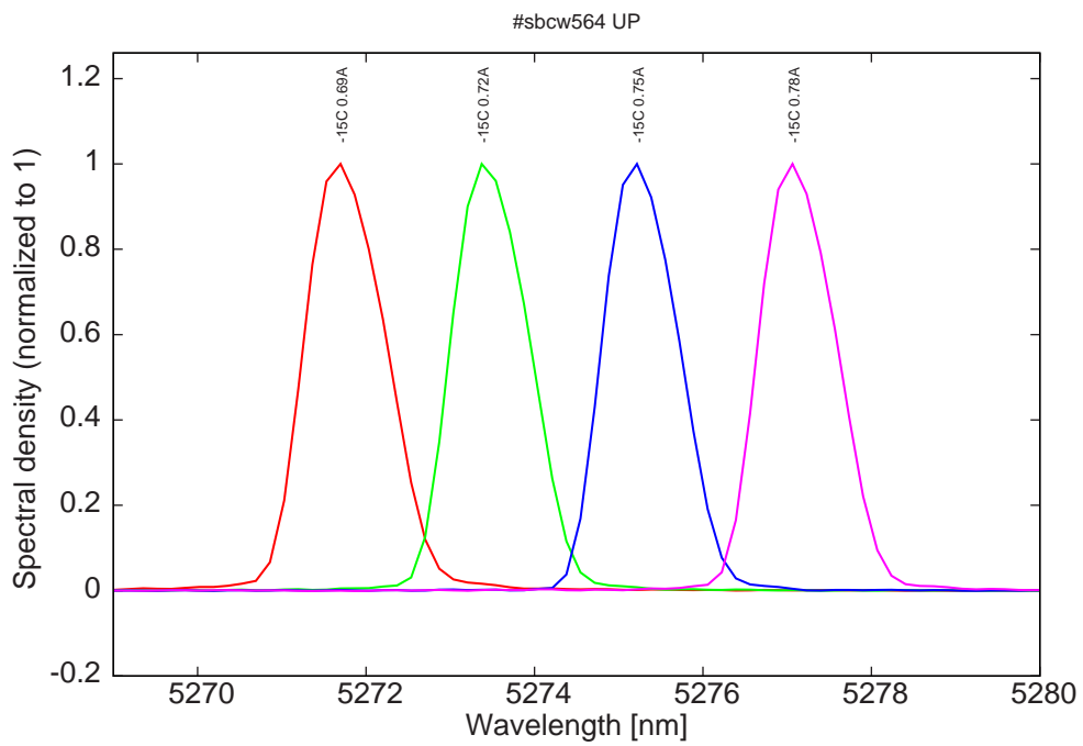
Figure 10: spectra at -15C for various DC currents
