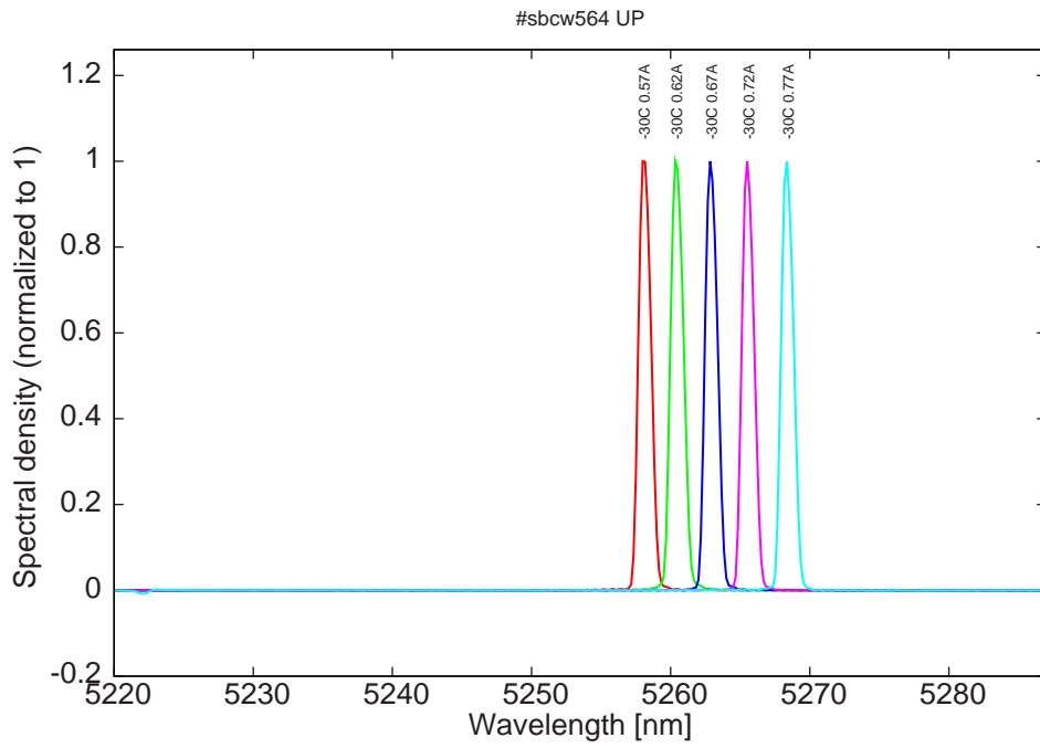
Figure 7: spectra at -30C for various DC currents (monomode up to 0.72A)
