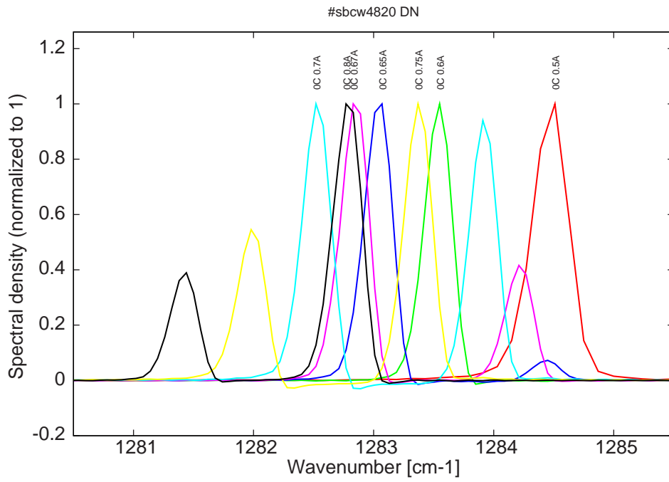
Figure 12: spectra at 0C for various DC currents (monomode up to 0.6A, then becomes bimode)
