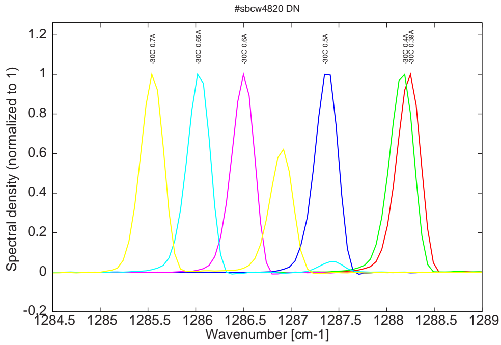
Figure 6: spectra at -30C for various DC currents (monomode up to 0.6A, then becomes bimode)
