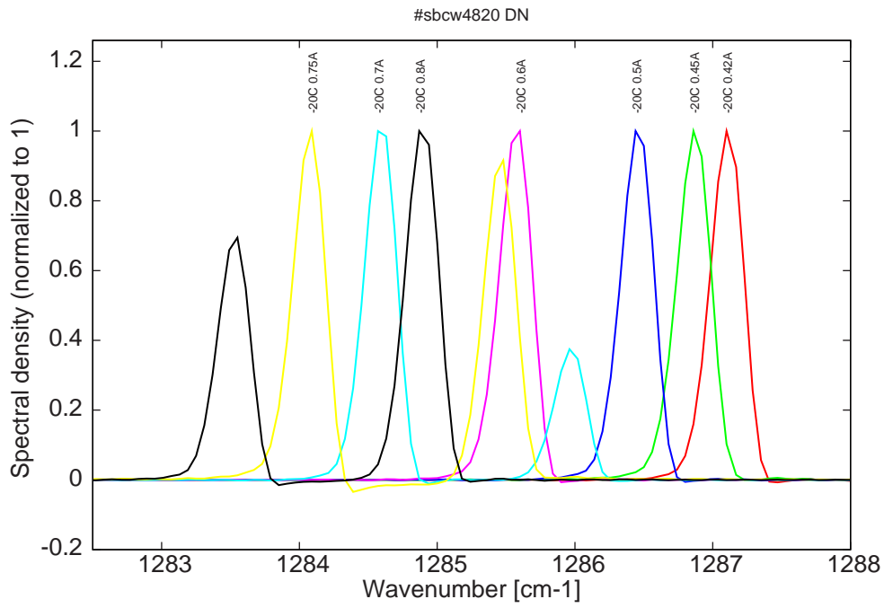
Figure 8: spectra at -20C for various DC currents (monomode up to 0.6A, then becomes bimode)
