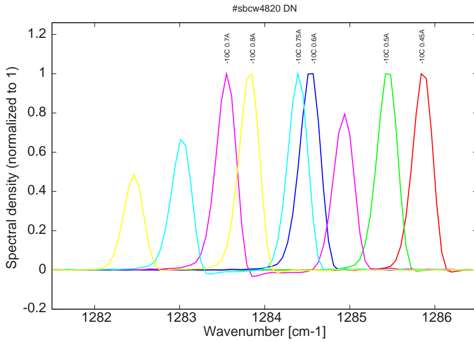
Figure 10: spectra at -10C for various DC currents (monomode up to 0.6A, then becomes bimode)
