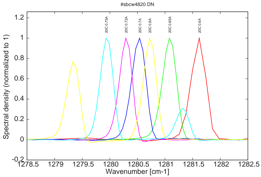
Figure 16: spectra at 20C for various DC currents (monomode up to 0.72A, then becomes bimode)
