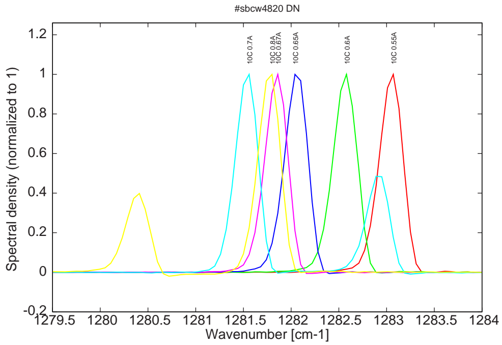
Figure 14: spectra at 10C for various DC currents (monomode up to 0.67A, then becomes bimode)
