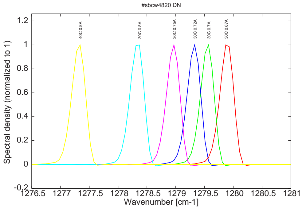
Figure 18: spectra between 30C and 40C for various DC currents (all monomode)
