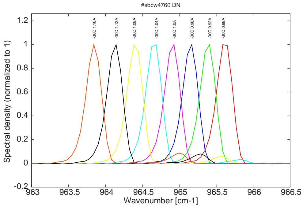
Figure 6: spectra at -30C for various DC currents (monomode up to 1A, then bimode, see Fig. 3)
