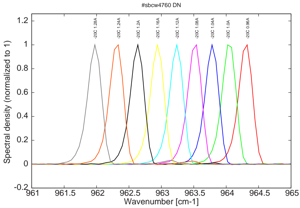
Figure 8: spectra at -20C for various DC currents (monomode up to 1.16A, then bimode, see Fig. 3)
