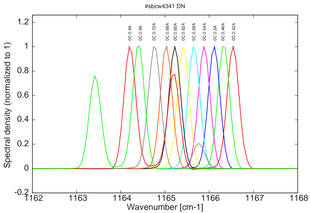
Figure 9: spectra at 0C for various DC currents (monomode up to 0.68A)
