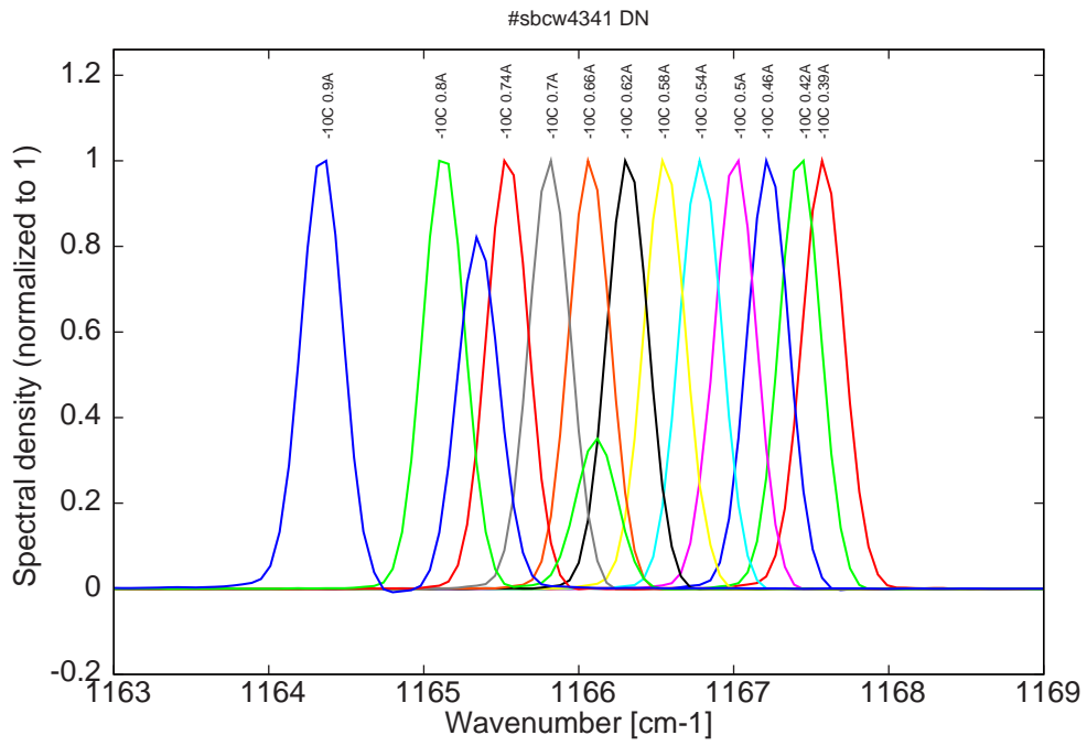
Figure 8: spectra at -10C for various DC currents (monomode up to 0.74A)
