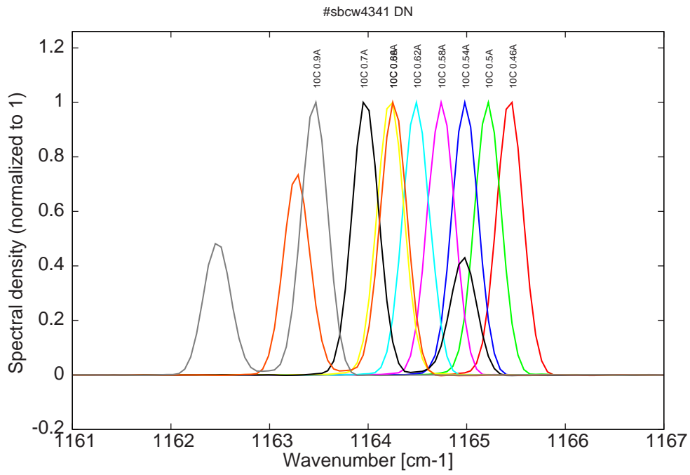
Figure 10: spectra at 10C for various DC currents (monomode up to 0.66A)
