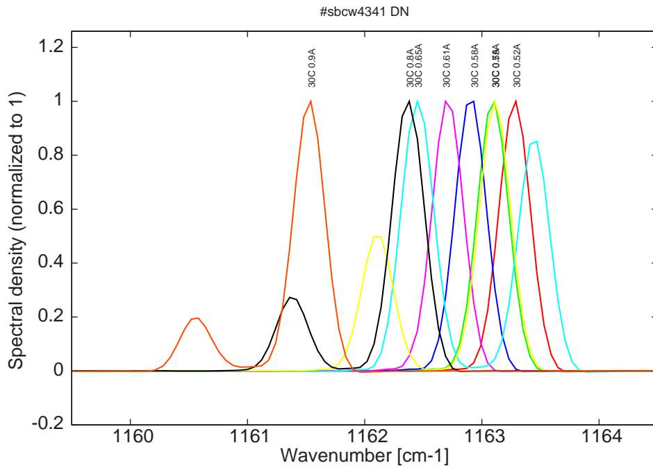
Figure 12: spectra at 30C for various DC currents (monomode up to 0.61A)
