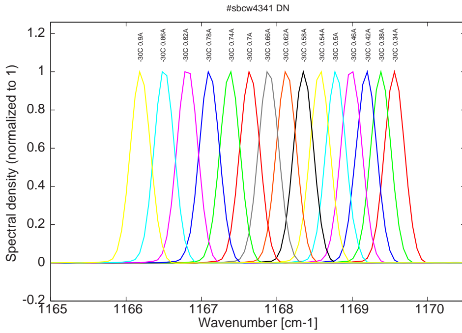
Figure 6: spectra at -30C for various DC currents (all monomode up to 0.9A)
