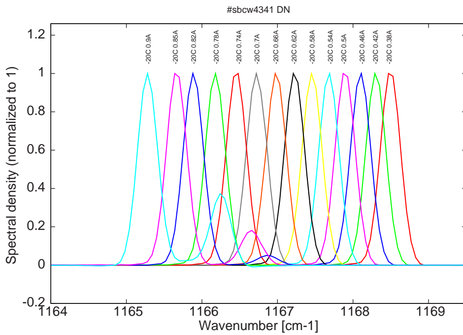
Figure 7: spectra at -20C for various DC currents (monomode up to 0.78A)
