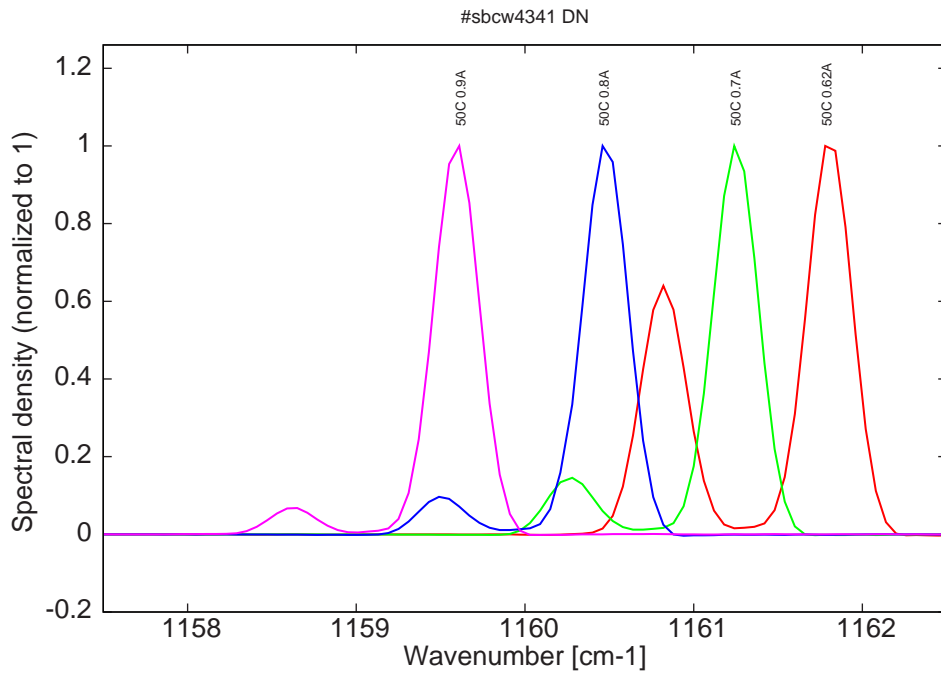
Figure 14: spectra at 50C for various DC currents (bimode)
