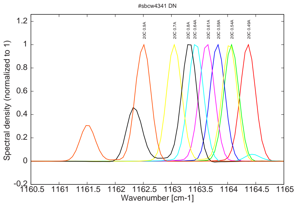
Figure 11: spectra at 20C for various DC currents (monomode up to 0.61A)
