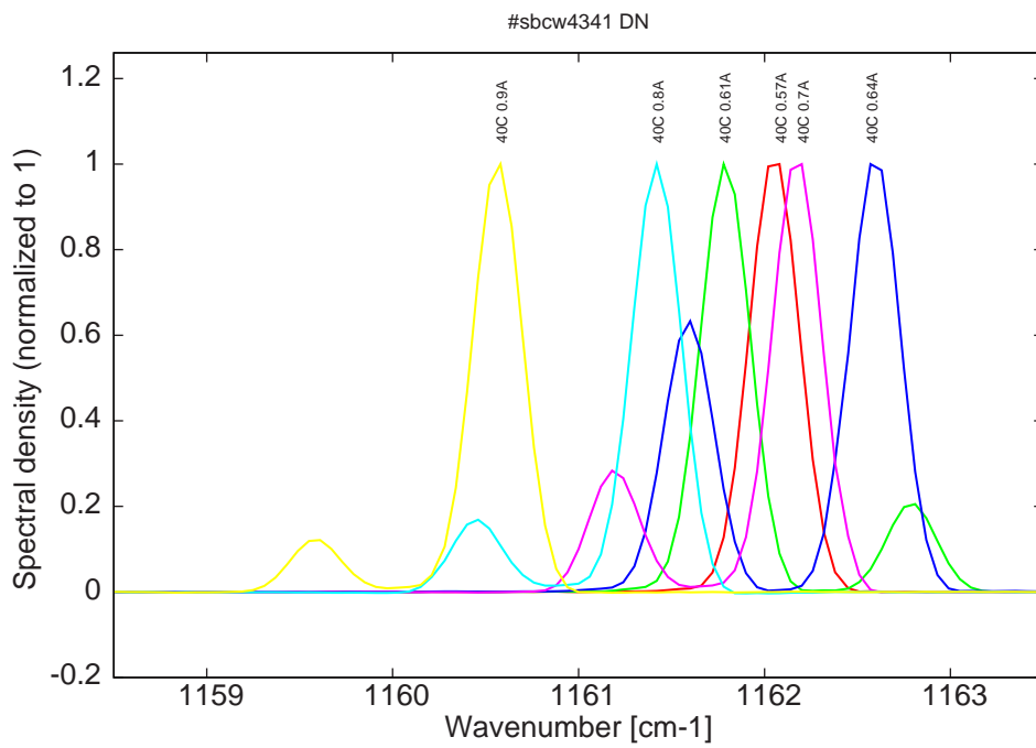
Figure 13: spectra at 40C for various DC currents (monomode only at threshold)
