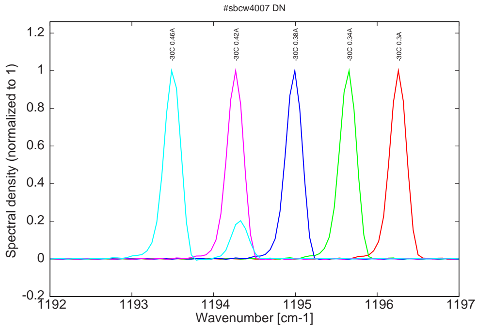
Figure 6: spectra at -30C for various DC currents (monomode up to 0.42A)
