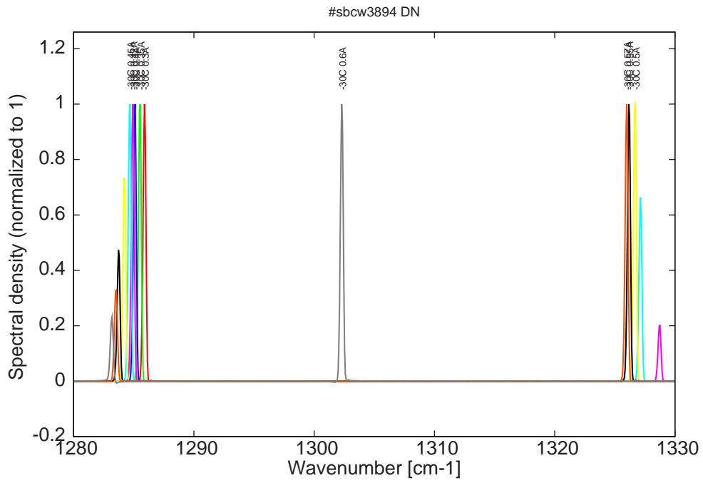
Figure 6: spectra at -30C for various DC currents (monomode up to 0.4A, then bimode)
