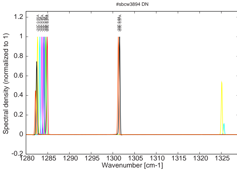
Figure 8: spectra at -20C for various DC currents (monomode up to 0.45A, then bimode)
