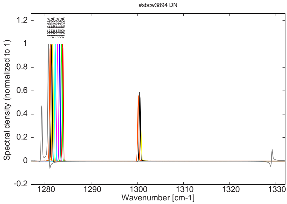
Figure 10: spectra at -10C for various DC currents (monomode up to 0.5A, then bimode)
