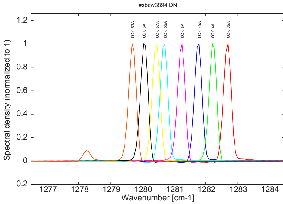
Figure 12: spectra at 0C for various DC currents (monomode up to 0.6A, then bimode)
