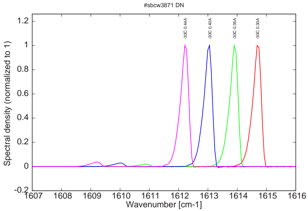
Figure 6: spectra at -30C for various DC currents (monomode only at threshold, then bimode)
