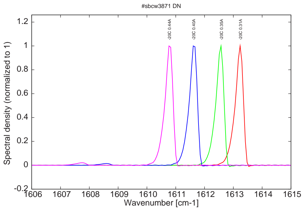
Figure 7: spectra at -20C for various DC currents (monomode up to 0.35A, then bimode)
