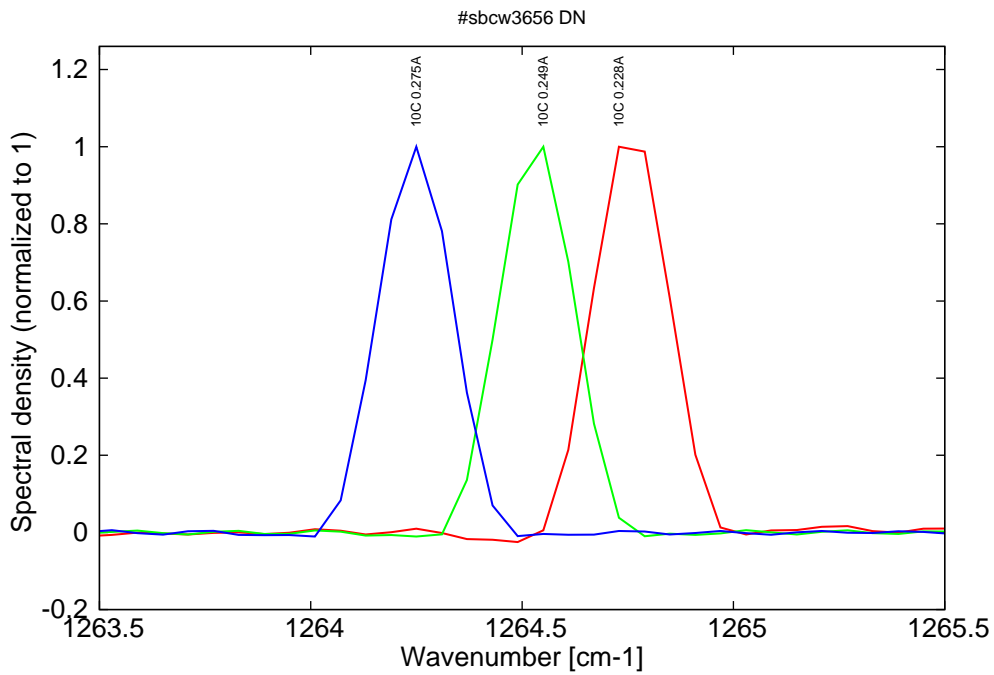
Figure 11: spectra at 10C for various DC currents (monomode on mode 2 range)
