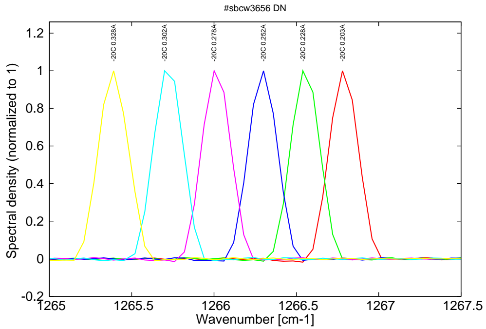
Figure 6: spectra at -20C for various DC currents (monomode on mode 1)
