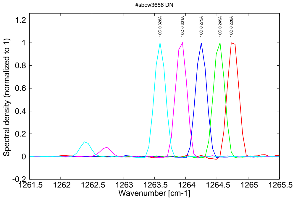
Figure 10: spectra at 10C for various DC currents (monomode on mode 2 up to 0.275A, then becomes bimode)
