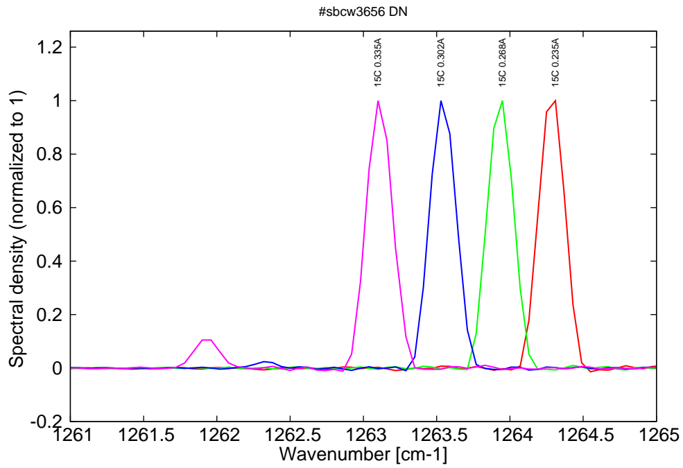
Figure 12: spectra at 15C for various DC currents (monomode on mode 2 up to 0.275A, then becomes bimode)
