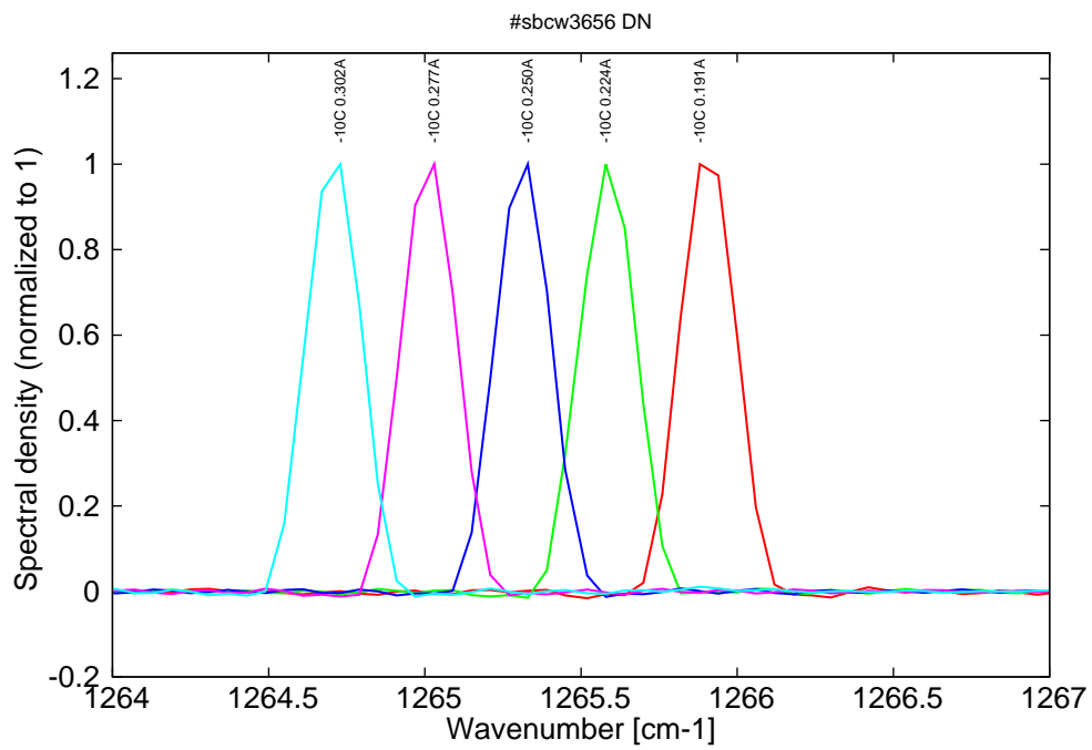
Figure 7: spectra at -10C for various DC currents (monomode on mode 1)
