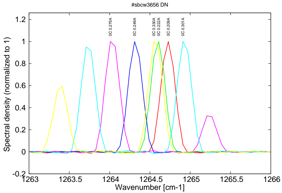
Figure 8: spectra at 0C for various DC currents (monomode on mode 1 up to 0.25A, then becomes bimode)
