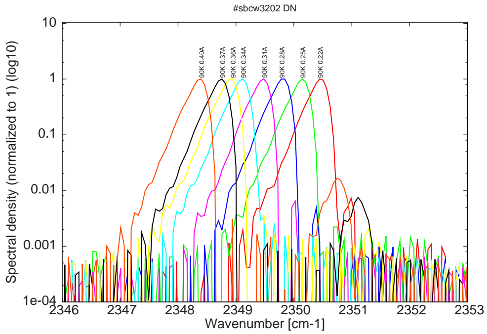
Figure 8: spectra at 90K for various DC currents
