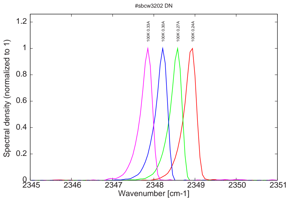
Figure 11: spectra at 100K for various DC currents (monomode range)
