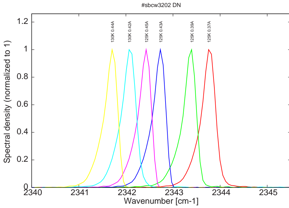
Figure 16: spectra between 125K and 130K for various DC currents (all monomode)
