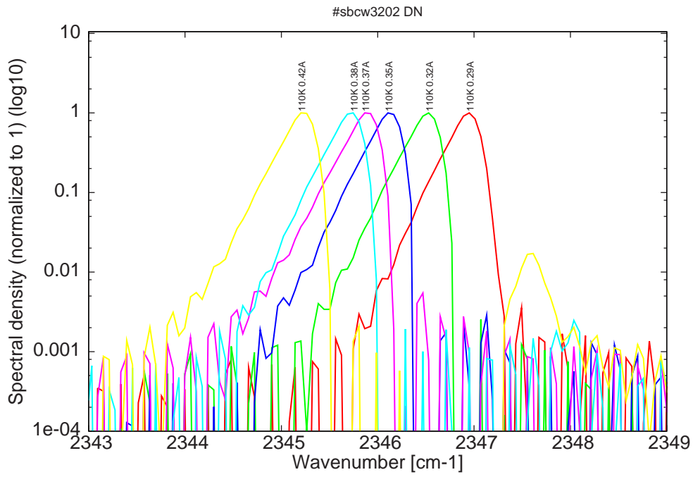
Figure 12: spectra at 110K for various DC currents
