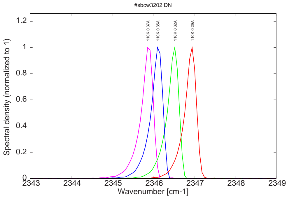
Figure 13: spectra at 110K for various DC currents (monomode range)
