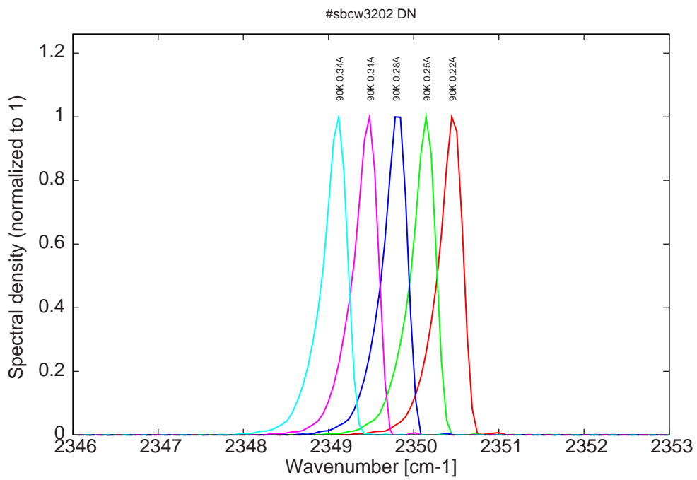
Figure 9: spectra at 90K for various DC currents (monomode range)
