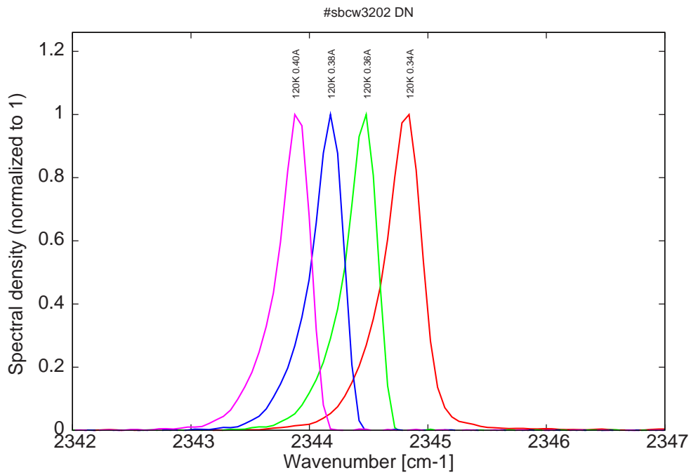
Figure 15: spectra at 120K for various DC currents (monomode range)
