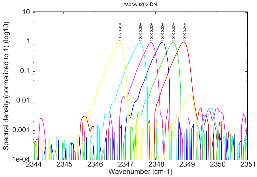
Figure 10: spectra at 100K for various DC currents
