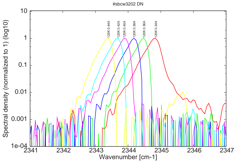
Figure 14: spectra at 120K for various DC currents
