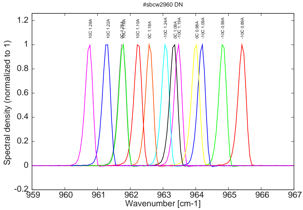
Figure 8: spectra from -10C to 10C for various DC currents (all monomode, with mode jumping compared to spectra at -30C and -20C, see Fig. 3)
