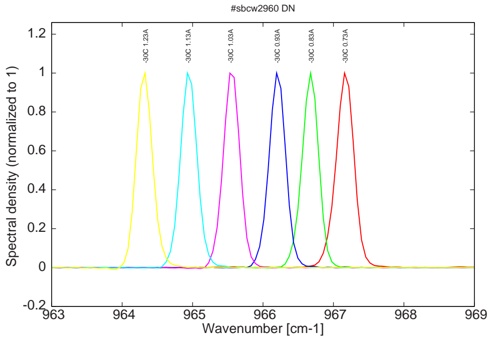
Figure 6: spectra at -30C for various DC currents (all monomode)
