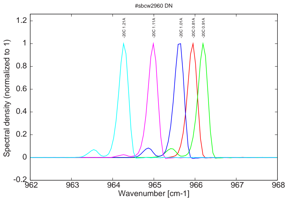
Figure 7: spectra at -20C for various DC currents (monomode only at threshold)
