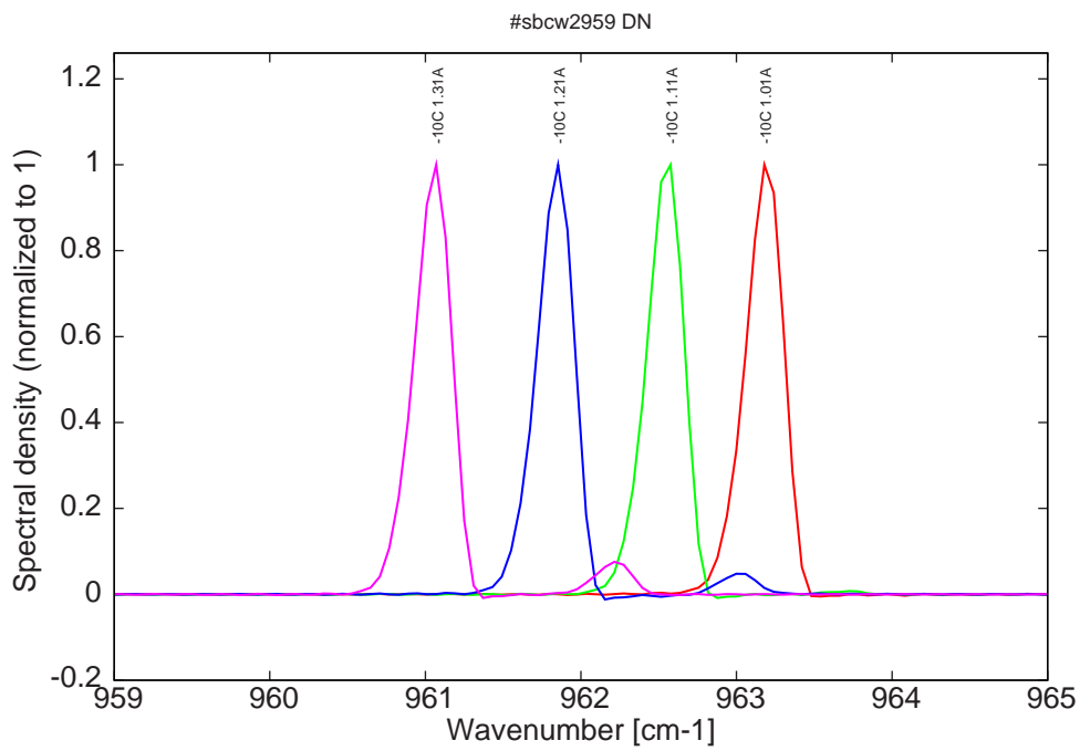
Figure 7: spectra at -10C for various DC currents (monomode only at threshold, see Fig. 3)
