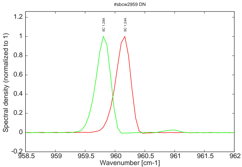
Figure 9: spectra at 5C for various DC currents (monomode only at threshold, mode jumping compared to spectra at -30C and -20C, see Fig. 3)
