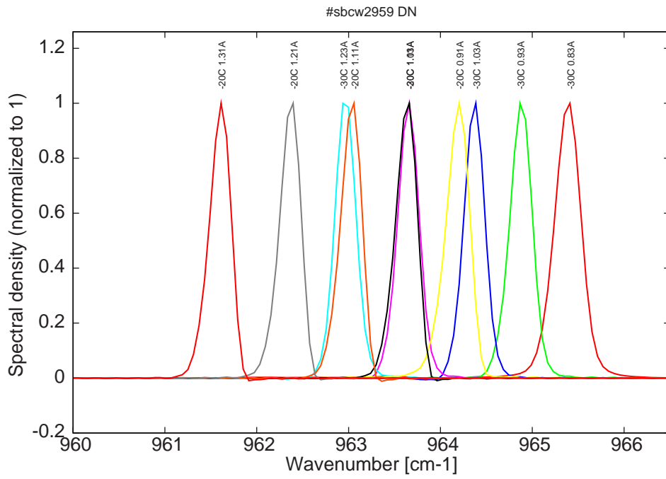
Figure 6: spectra at -30C and -20C for various DC currents (all monomode)
