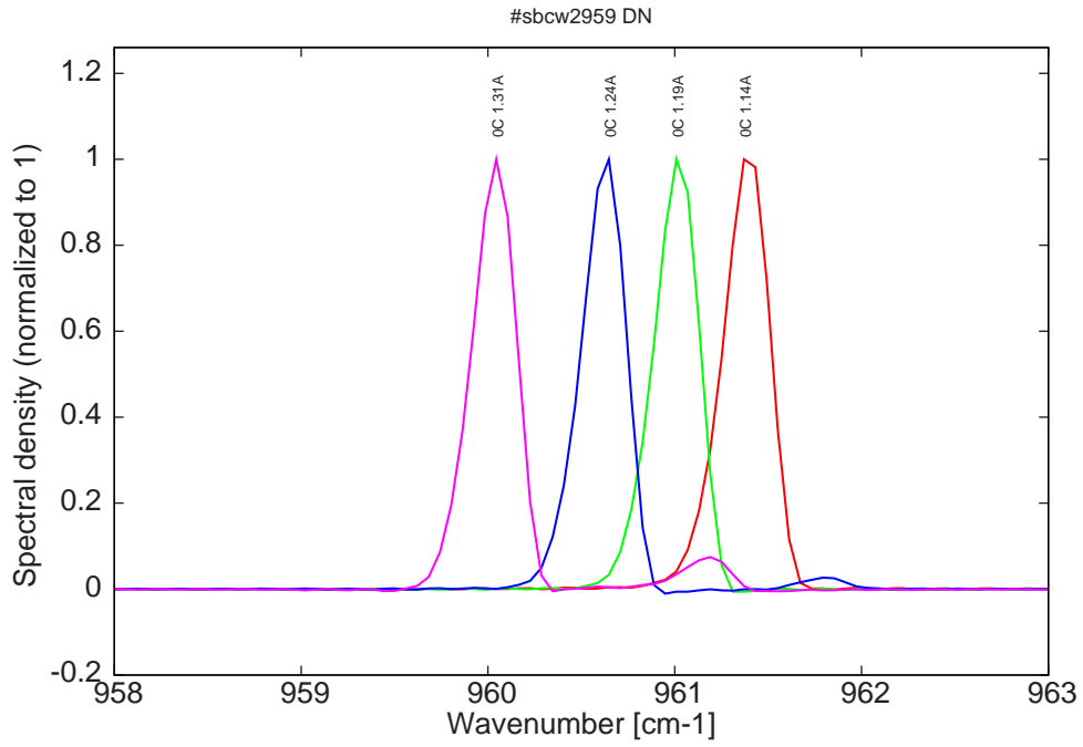
Figure 8: spectra at 0C for various DC currents (monomode up to 1.19A, mode jumping compared to spectra at -30C and -20C, see Fig. 3)
