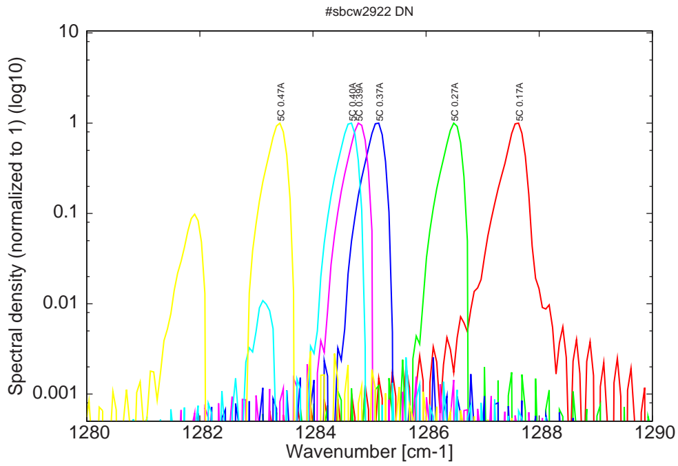
Figure 10: spectra at 5C for various DC currents (bimode for I \geq 0.40A )
