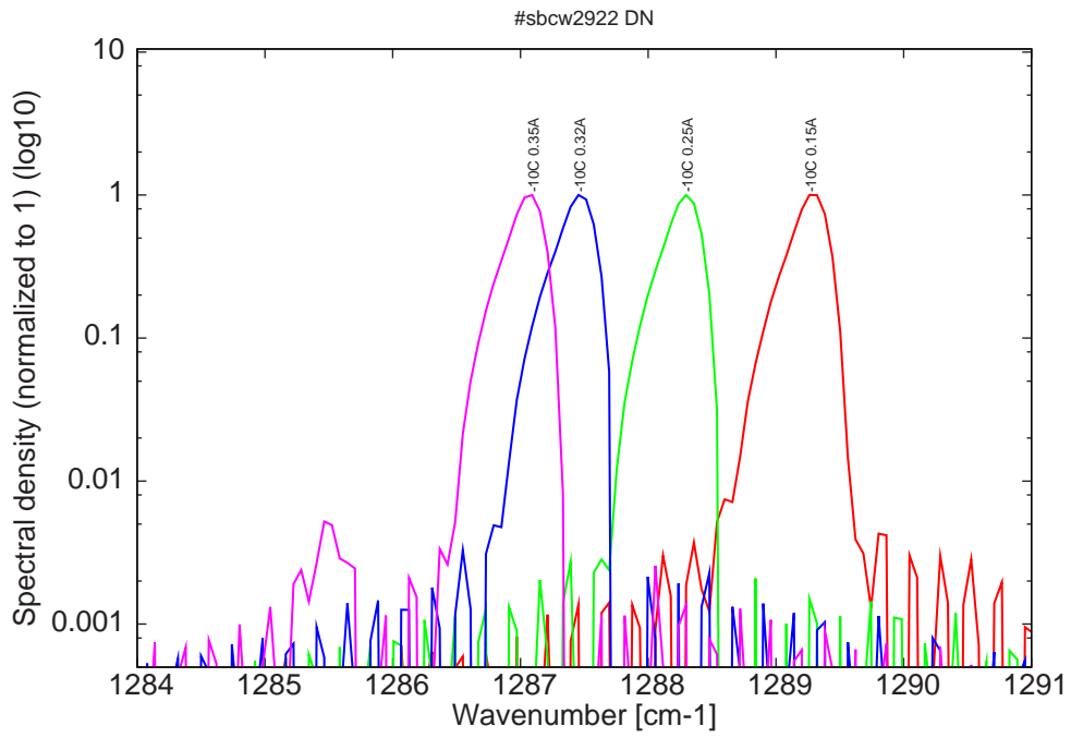
Figure 8: spectra at -10C for various DC currents (bimode for I \geq 0.35A )
