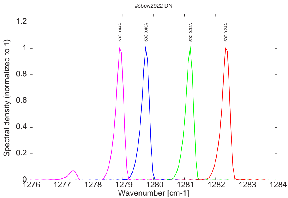
Figure 15: spectra at 50C for various DC currents (bimode for I \geq 0.44A )
