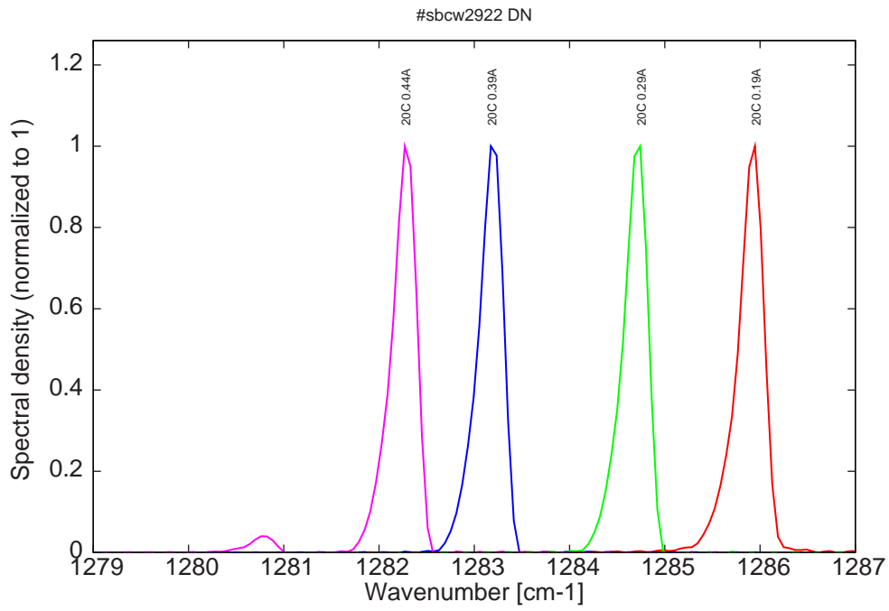
Figure 12: spectra at 20C for various DC currents (bimode for I \geq 0.44A )
