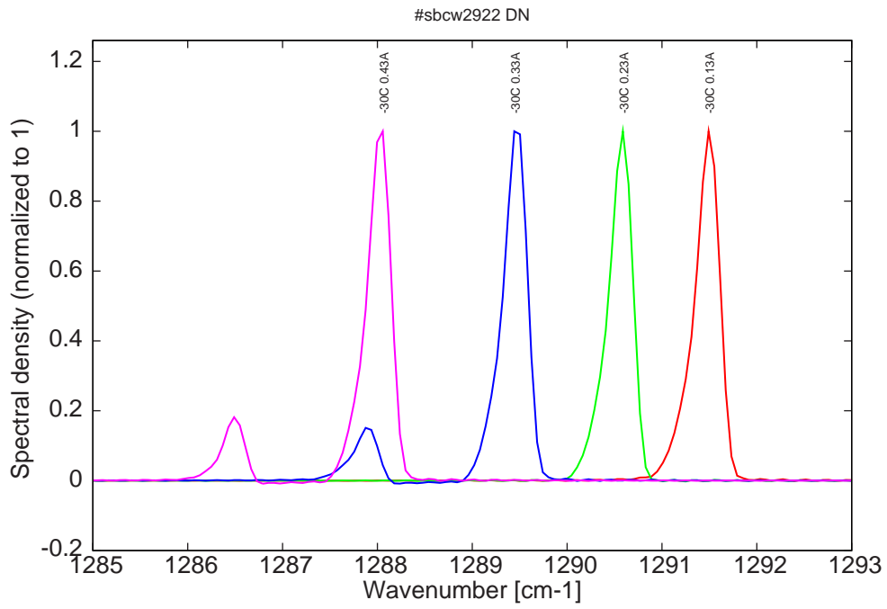
Figure 6: spectra at -30C for various DC currents (bimode for I \geq 0.33A )
