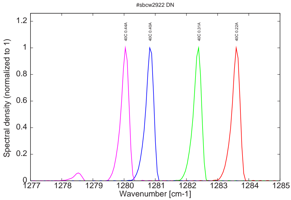
Figure 14: spectra at 40C for various DC currents (bimode for I \geq 0.44A )
