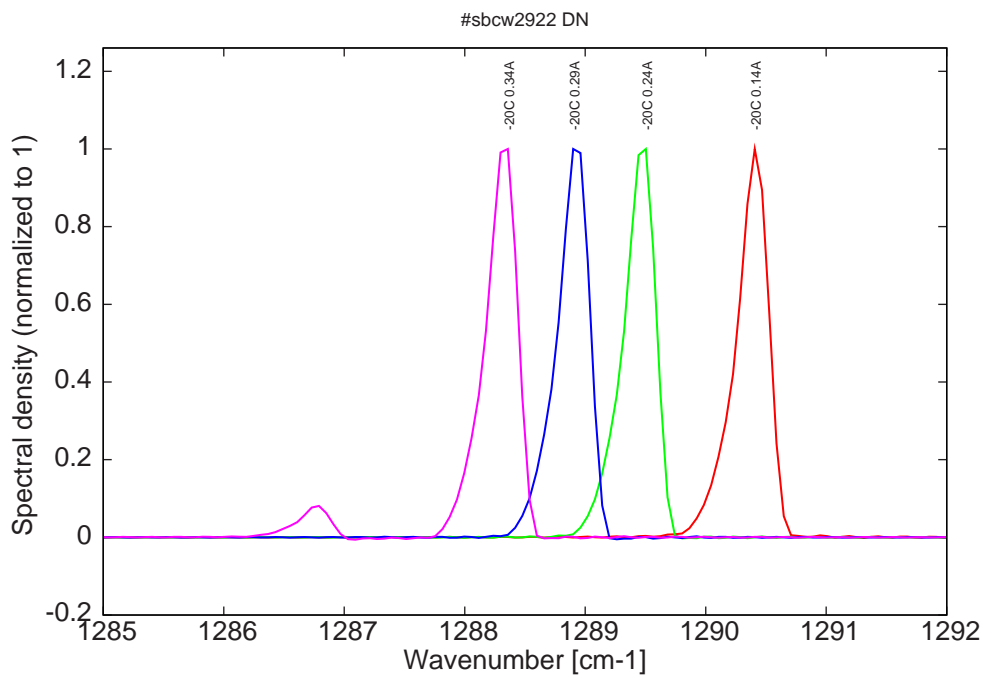
Figure 7: spectra at -20C for various DC currents (bimode for I \geq 0.34A )
