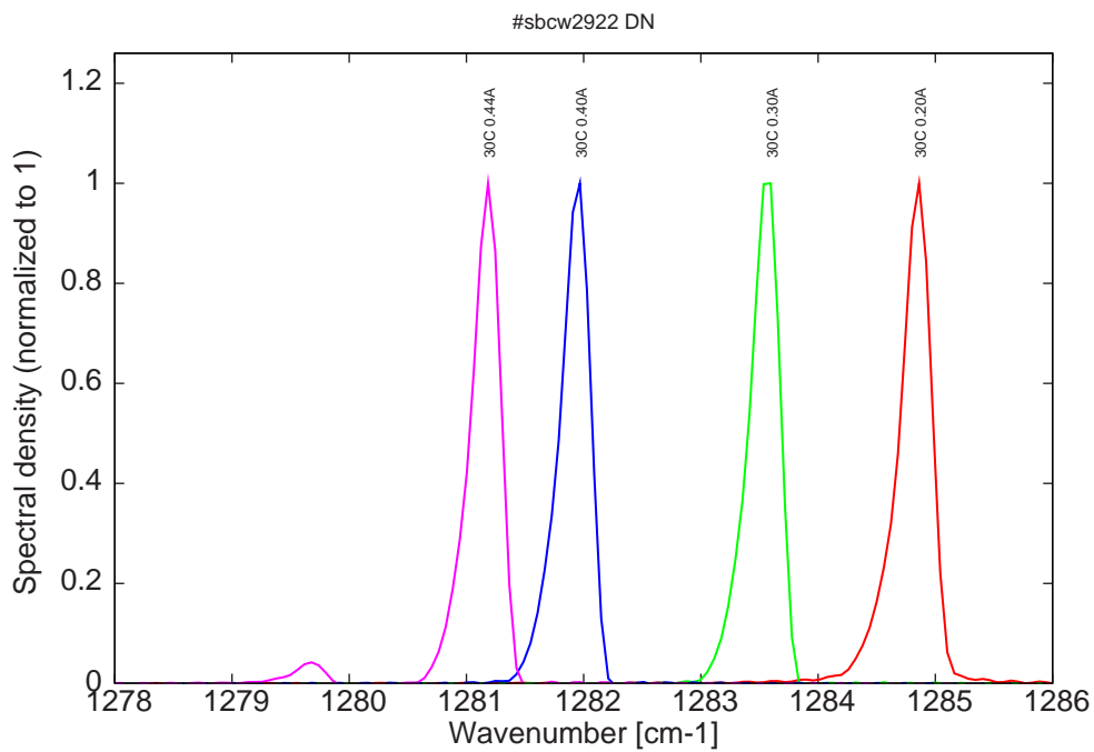
Figure 13: spectra at 30C for various DC currents (bimode for I \geq 0.44A )
