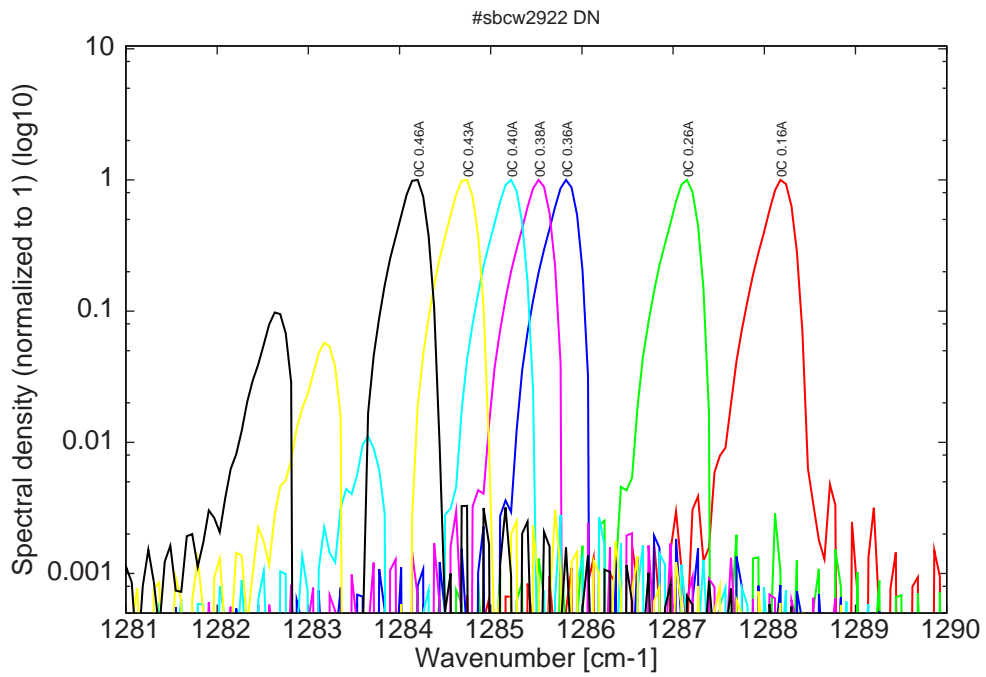
Figure 9: spectra at 0C for various DC currents (bimode for I \geq 0.40A )
