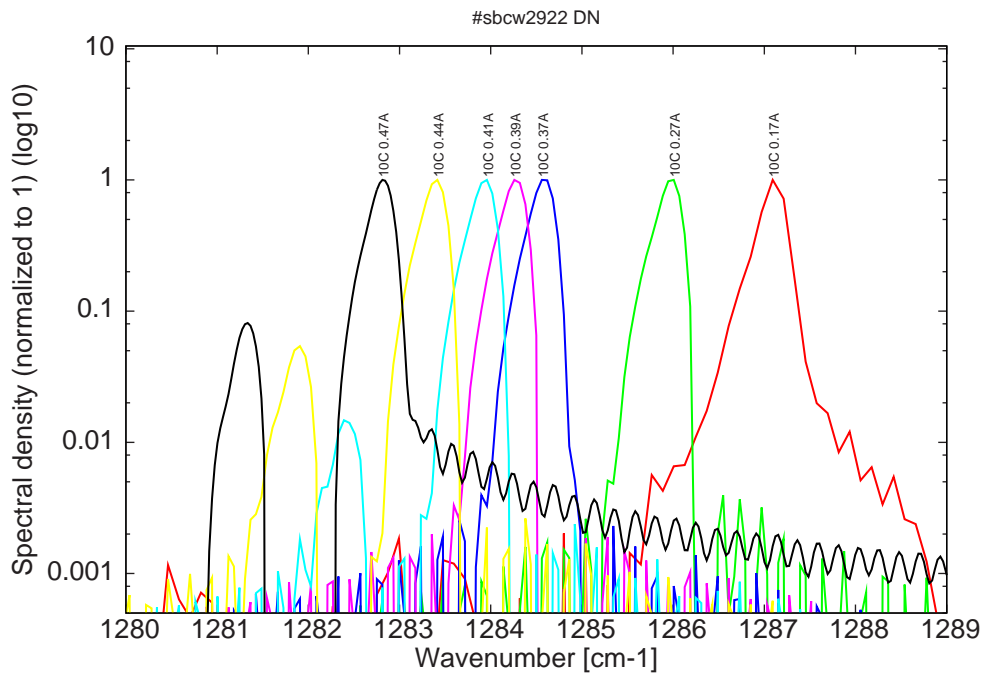
Figure 11: spectra at 10C for various DC currents (bimode for I \geq 0.41A )
