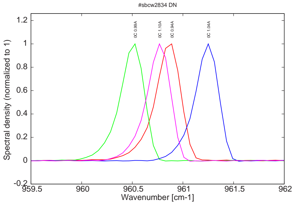
Figure 12: spectra at 0C for various DC currents (monomode range with mode jumping between 0.99A and 1.04A, see Fig. 3)
