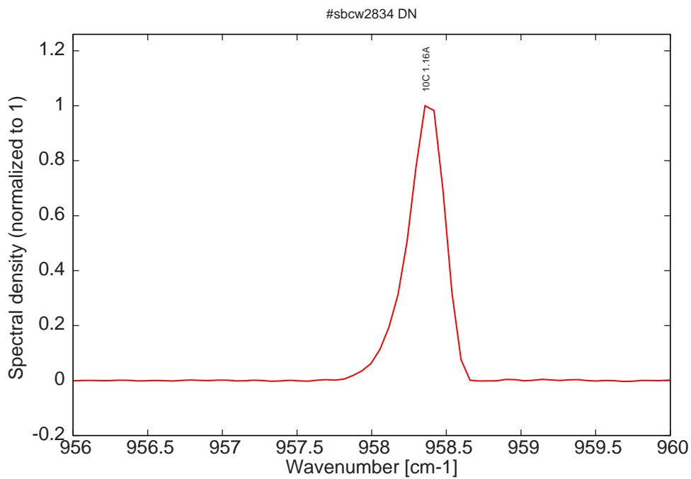
Figure 13: spectrum at 10C at 1.16A (monomode but on a different mode compared the other temperatures, see Fig. 3)
