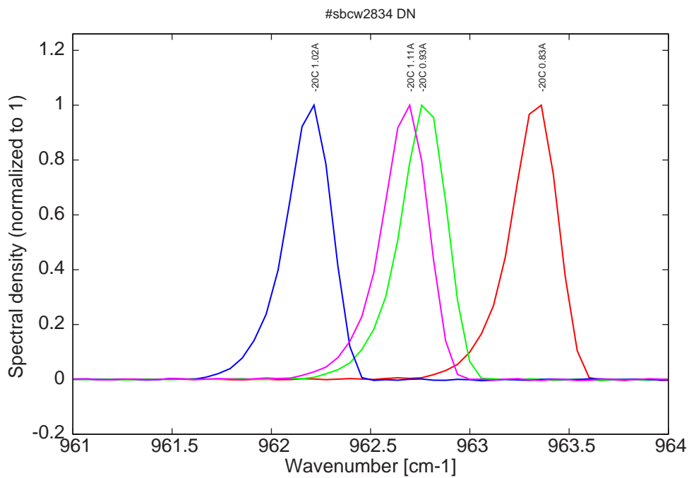
Figure 9: spectra at -20C for various DC currents (monomode range with mode jumping between 1.02A and 1.11A, see Fig. 3)
