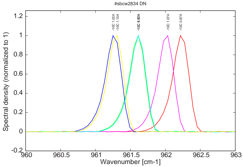
Figure 10: spectra at -10C for various DC currents (all monomode but with mode jumping between 1.02A and 1.07A, see Fig. 3)
