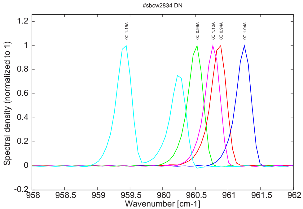
Figure 11: spectra at 0C for various DC currents (monomode up to 1.10A)
