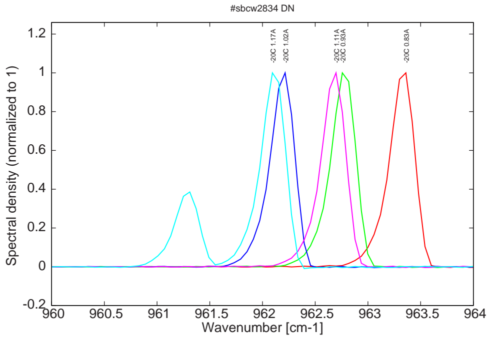
Figure 8: spectra at -20C for various DC currents (monomode up to 1.11A)
