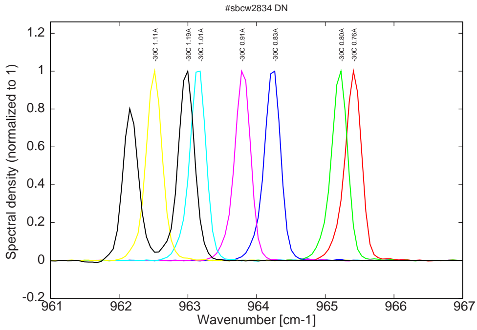
Figure 6: spectra at -30C for various DC currents (monomode up to 1.11A)
