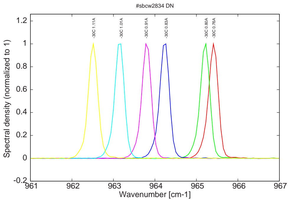
Figure 7: spectra at -30C for various DC currents (monomode range with mode jumping between 0.80A and 0.83A, see Fig. 3)
