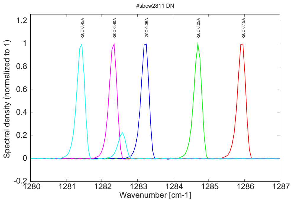
Figure 7: spectra at -20C for various DC currents (monomode up to 0.40A)
