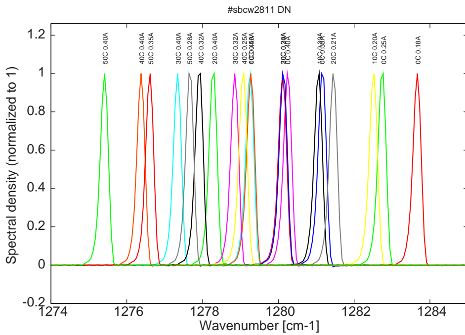
Figure 9: spectra between 0C and 50C for various DC currents (all monomode)
