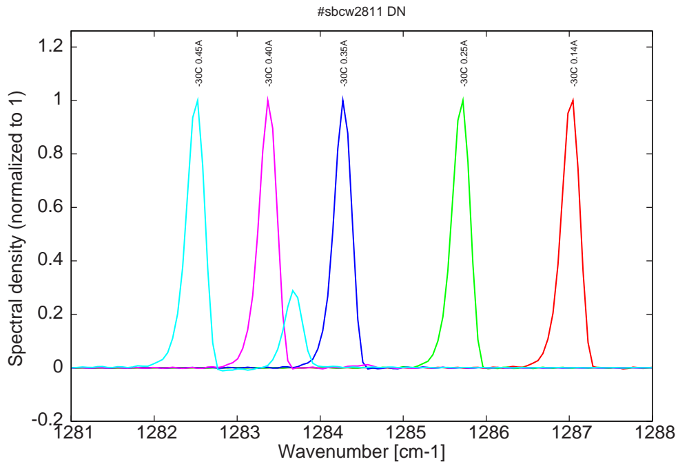
Figure 6: spectra at -30C for various DC currents (monomode up to 0.40A)
