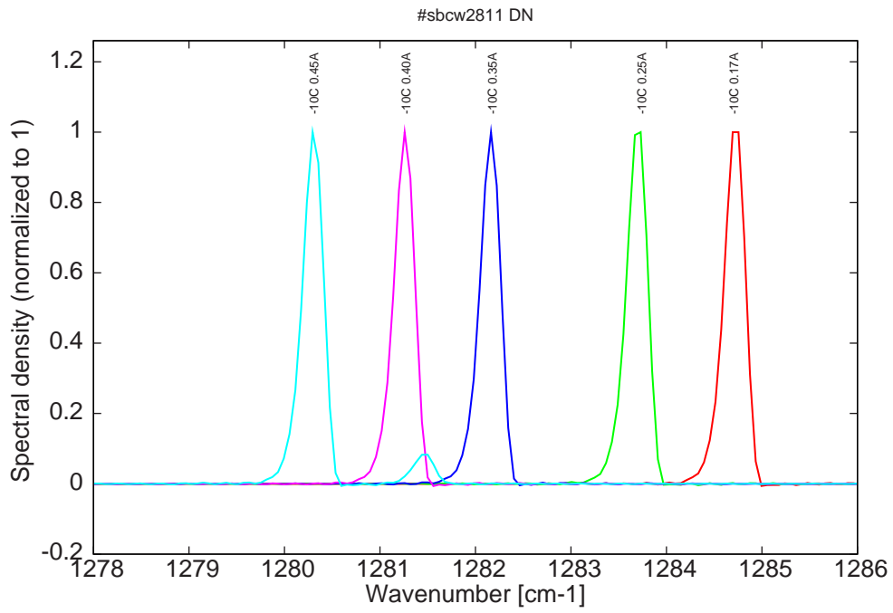
Figure 8: spectra at -10C for various DC currents (monomode up to 0.40A)
