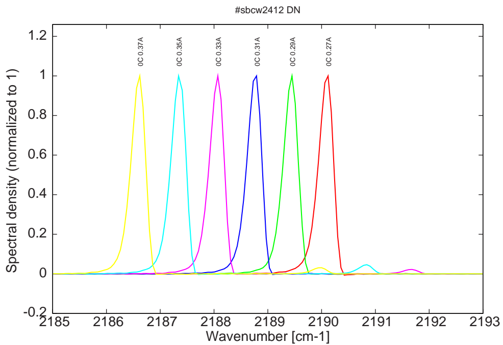
Figure 9: spectra at 0C for various DC currents (become bimode for I > 0.31A )
