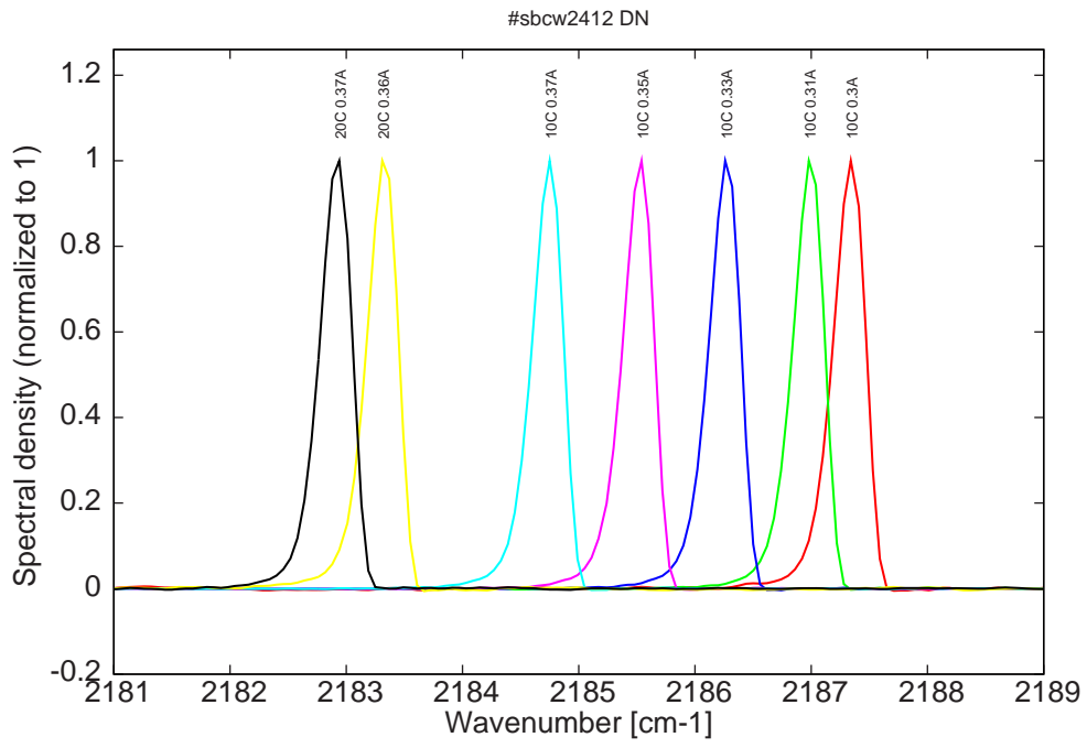
Figure 10: spectra at 10C and 20C for various DC currents (all monomode)
