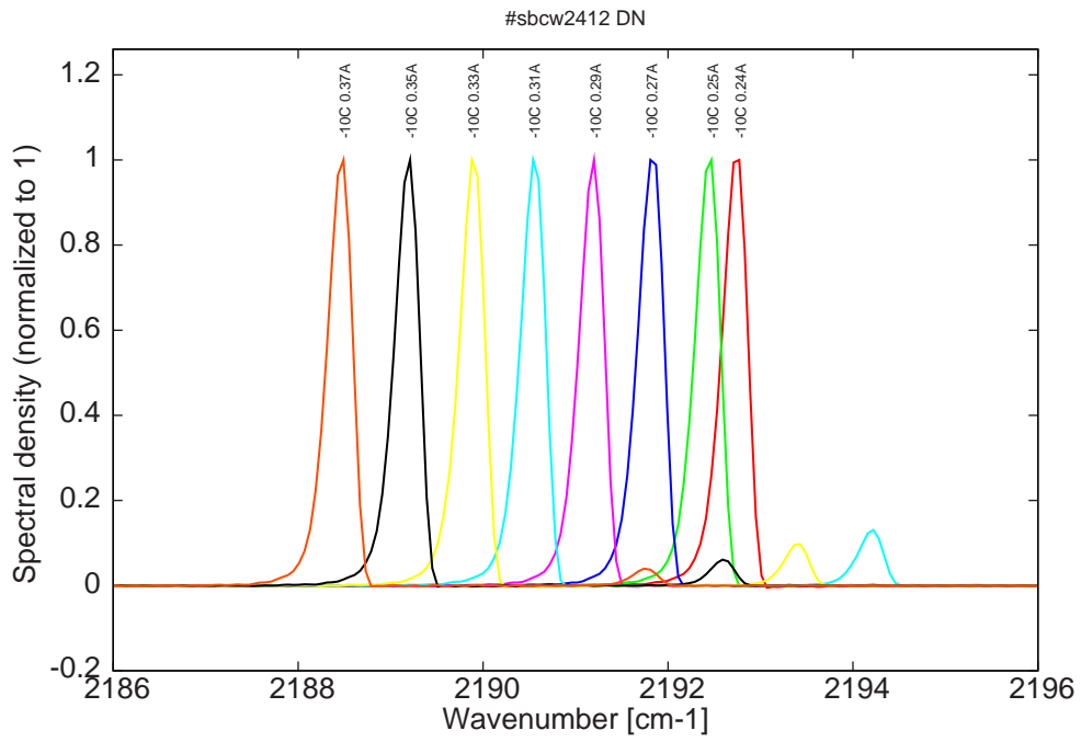
Figure 8: spectra at -10C for various DC currents (become bimode for I > 0.29A )
