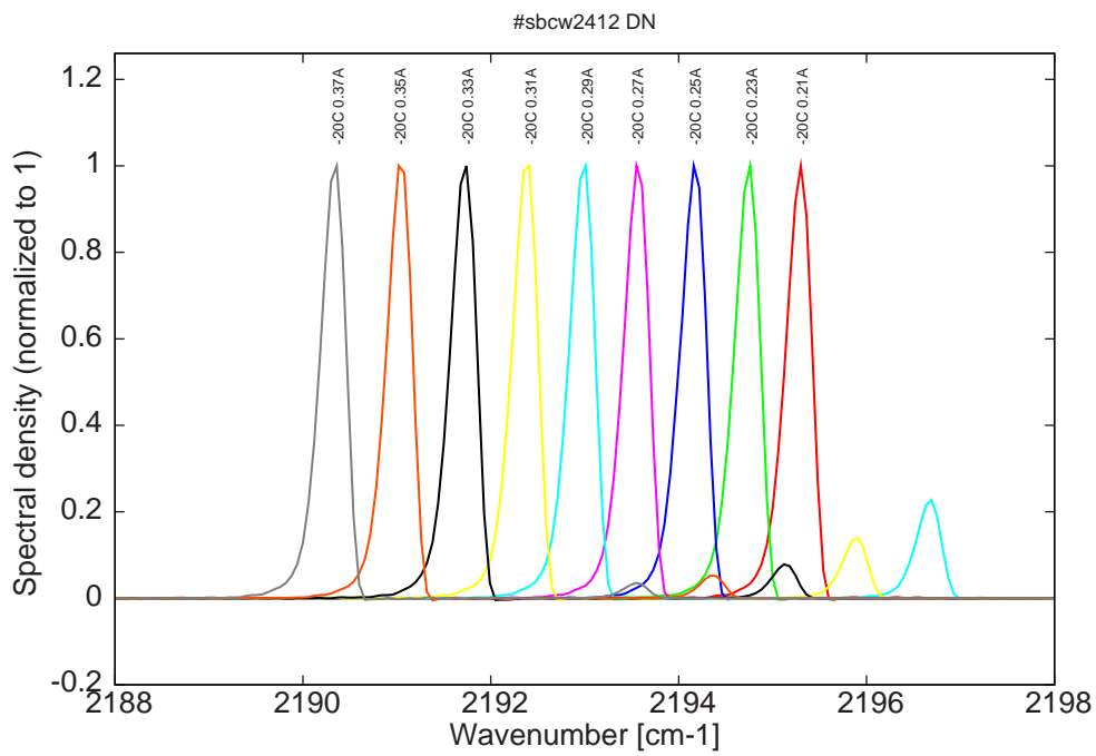
Figure 7: spectra at -20C for various DC currents (become bimode for I > 0.27A )
