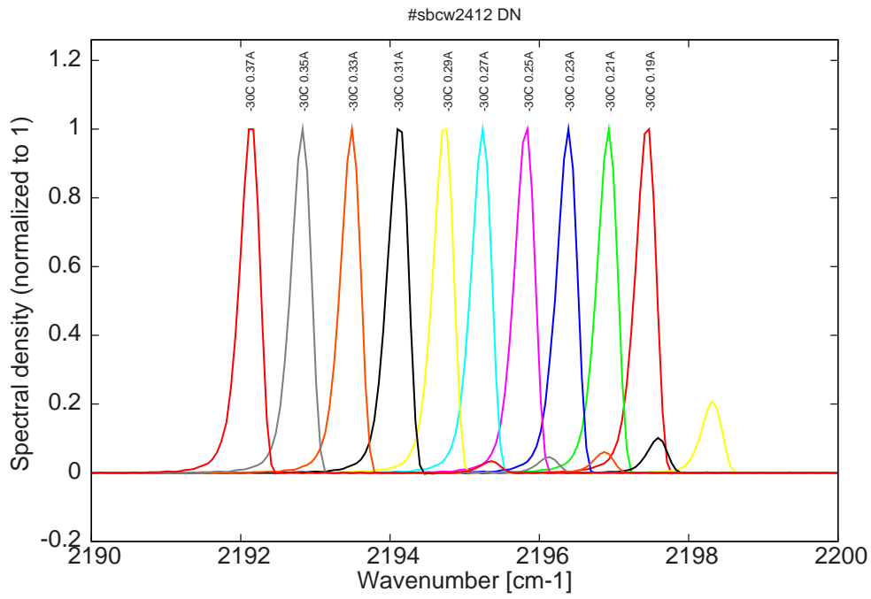
Figure 6: spectra at -30C for various DC currents (become bimode for I > 0.27A )
