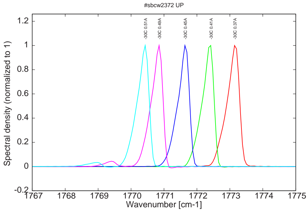
Figure 6: spectra at -30C for various DC currents (monomode up to 0.45A)
