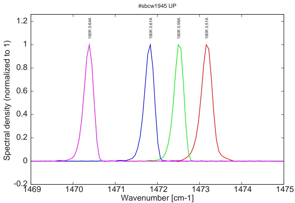
Figure 9: spectra at 160K for various DC currents (all monomode, but with mode jumping for I > 0.61A , see Fig. 1)
