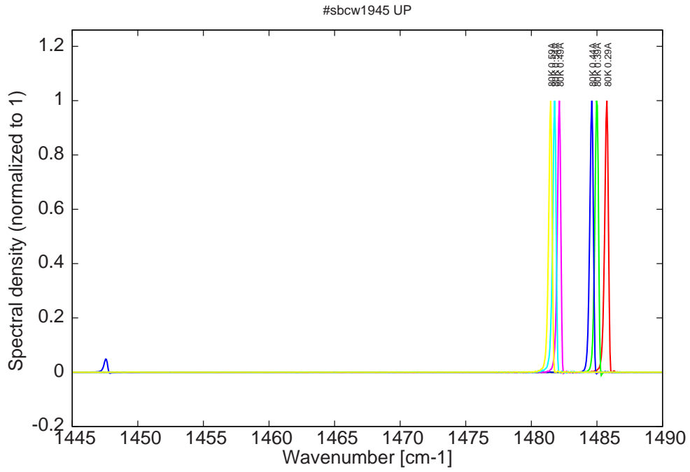
Figure 6: spectra at 80K for various DC currents (bimode around 0.44A)
