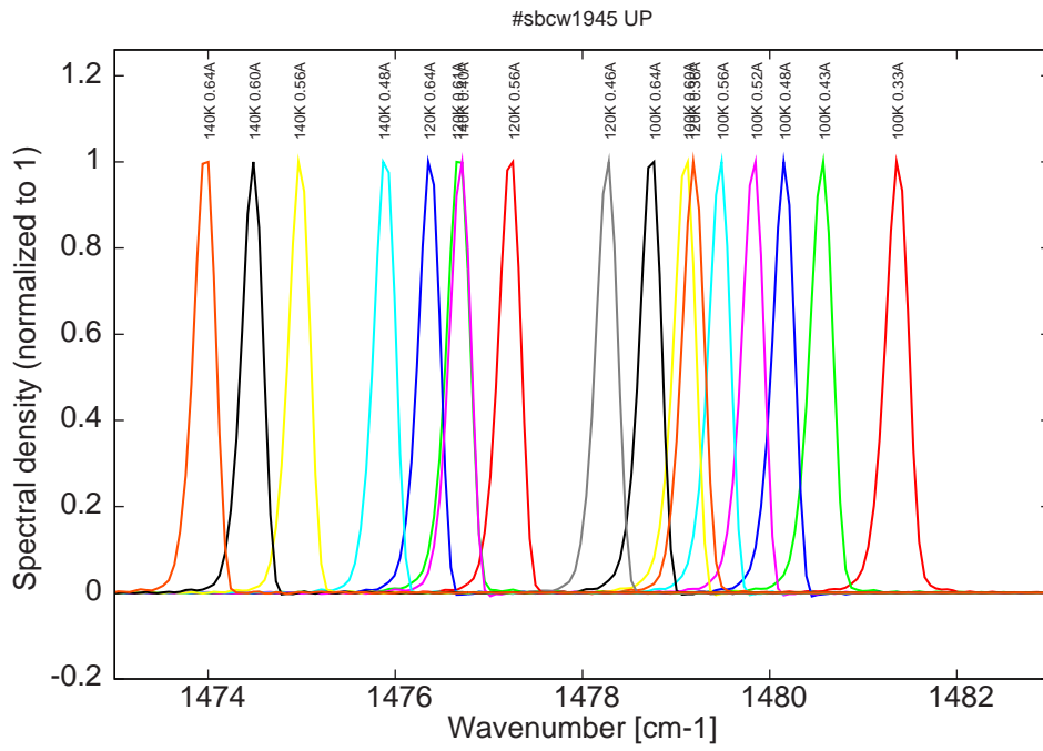
Figure 8: spectra between 100K and 140K for various DC currents (all monomode)
