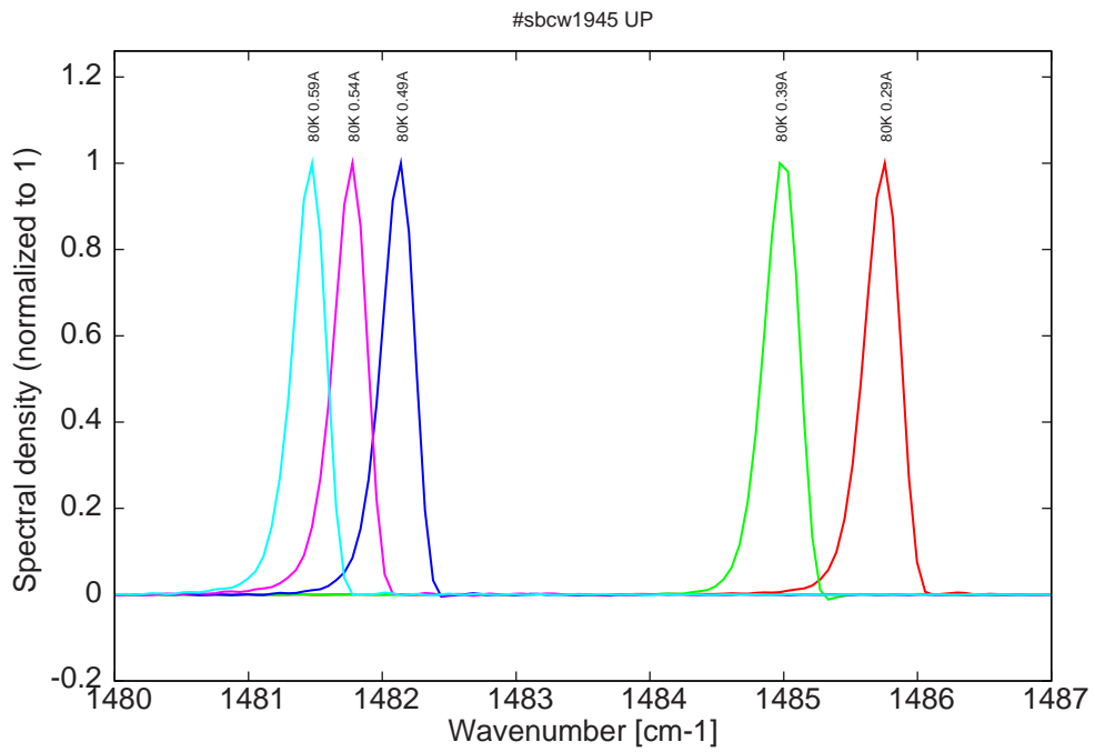
Figure 7: spectra at 80K for various DC currents (monomode range, but lower currents spectra on another mode compared to higher temperatures, see Fig. 1)
