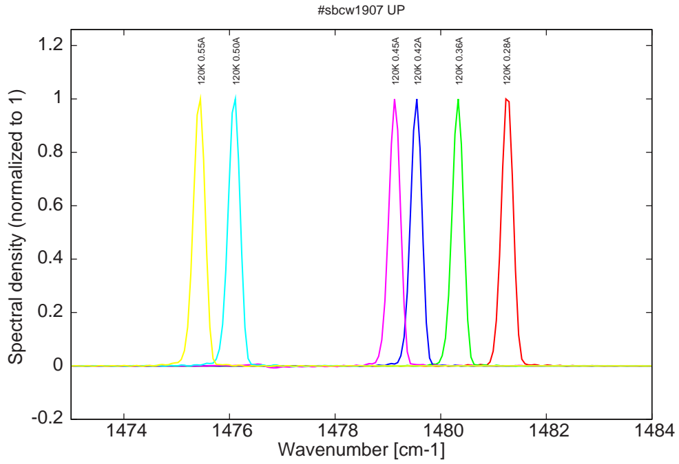
Figure 8: spectra at 120K for various DC currents (monomode up to 0.42A, then bimode and again monomode from 0.50A to 0.55A but on another mode, see Fig.1)
