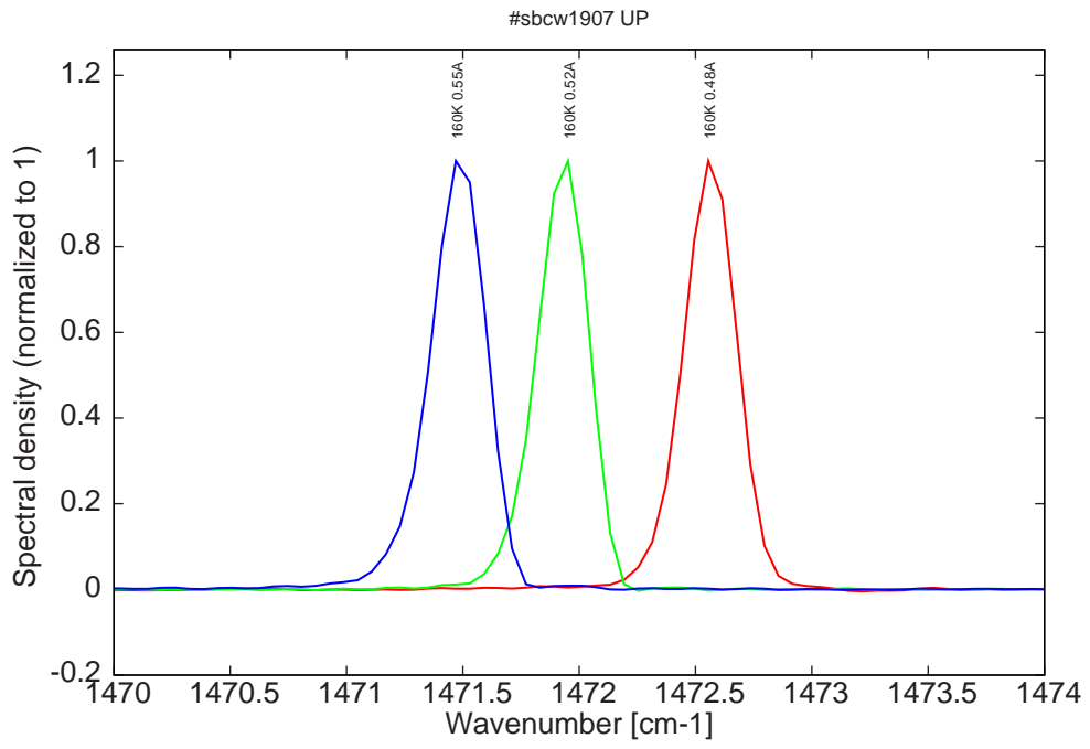
Figure 10: spectra at 160K for various DC currents (all monomode but on another mode, see Fig.1)
