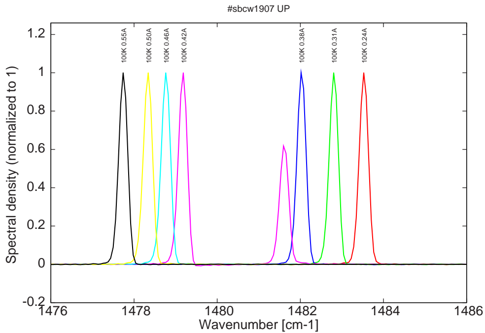
Figure 7: spectra at 100K for various DC currents (monomode up to 0.38A, then bimode and again monomode from 0.46A to 0.55A but on another mode, see Fig.1)
