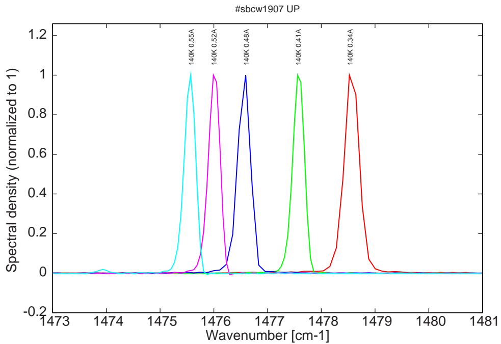
Figure 9: spectra at 140K for various DC currents (monomode up to 0.52A, then bimode, see Fig.1)
