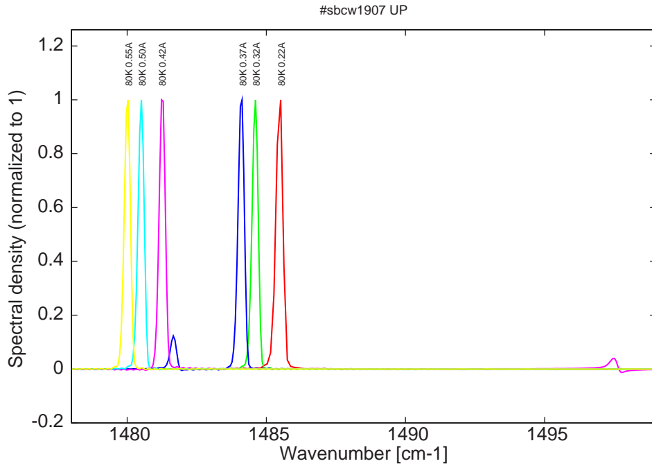
Figure 6: spectra at 80K for various DC currents (monomode up to 0.32A, then bimode and again monomode from 0.50A to 0.55A but on another mode, see Fig.1)
