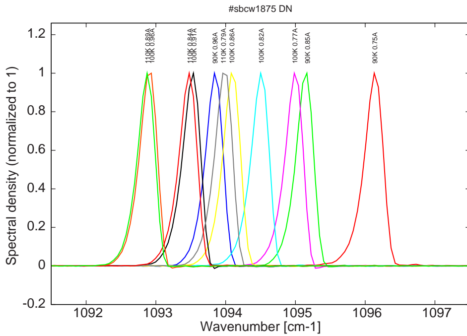
Figure 6: spectra at 90K, 100K and 110K for various DC currents (all monomode on the same mode, see Fig. 1)
