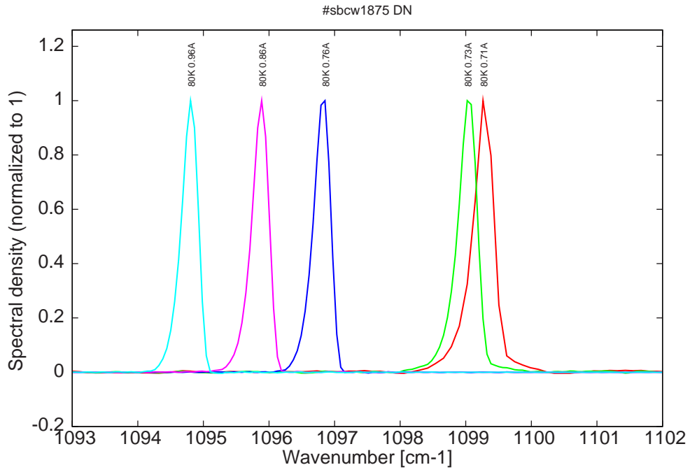
Figure 5: spectra at 80K for various DC currents (mode jumping for I > 0.73A , same mode as at higher temperature, see Fig. 1)
