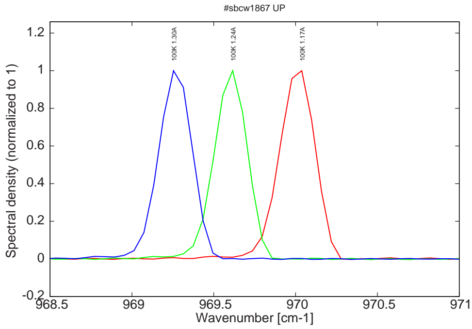
Figure 8: spectra at 100K for various DC currents (all monomode)
