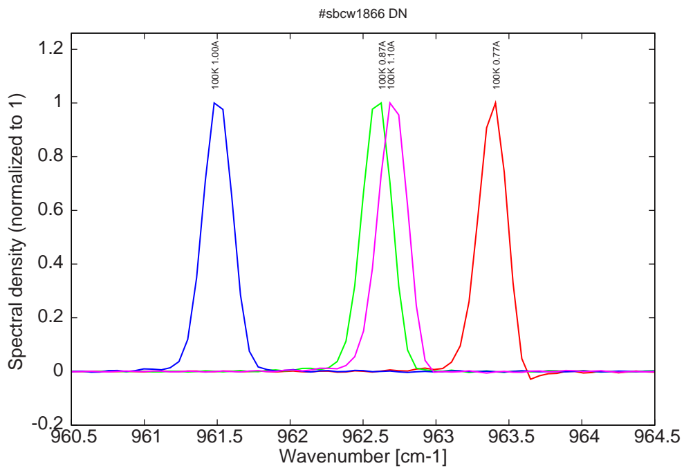
Figure 6: spectra at 100K for various DC currents (mode jumping for I > 1.00\text{A} , see Fig. 1)
