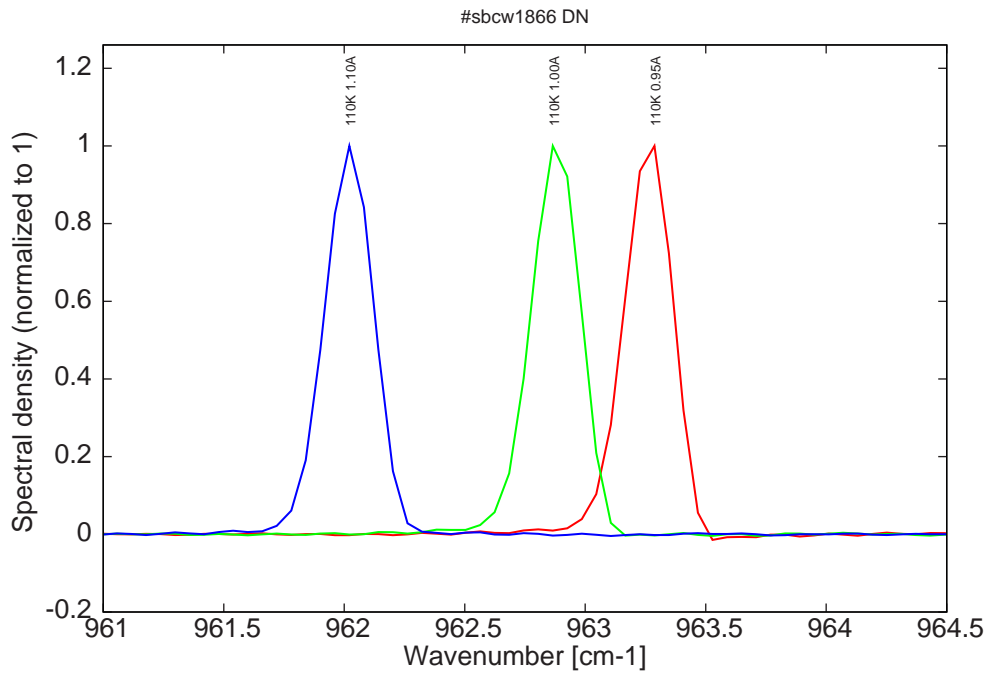
Figure 7: spectra at 110K for various DC currents (all monomode, but on the same mode as higher currents at 100K, see Fig. 1)
