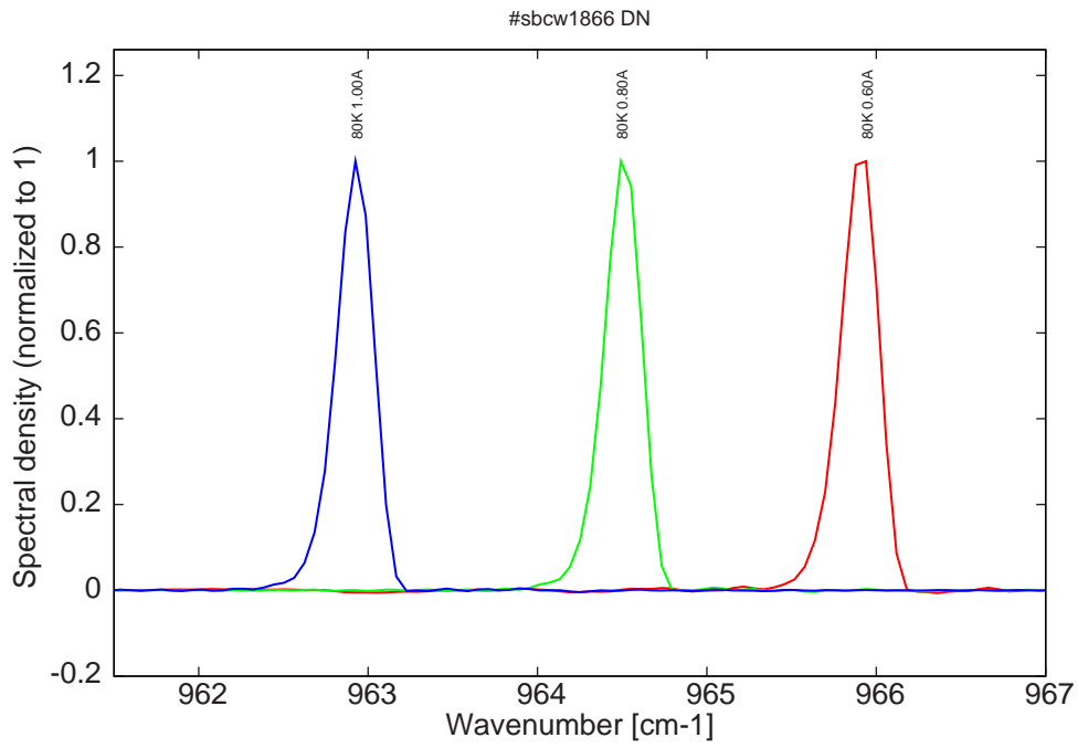
Figure 5: spectra at 80K for various DC currents (all monomode)
