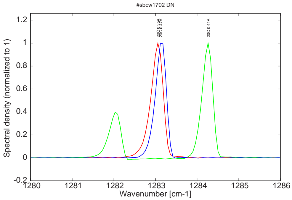
Figure 12: spectra at 20C for various DC currents
