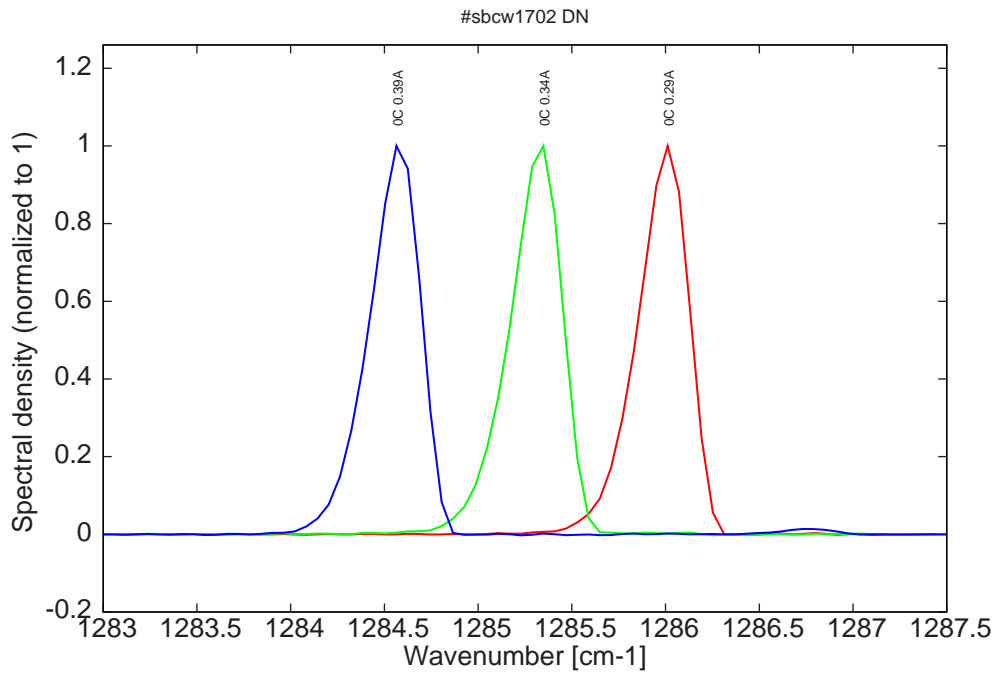
Figure 10: spectra at 0C for various DC currents
