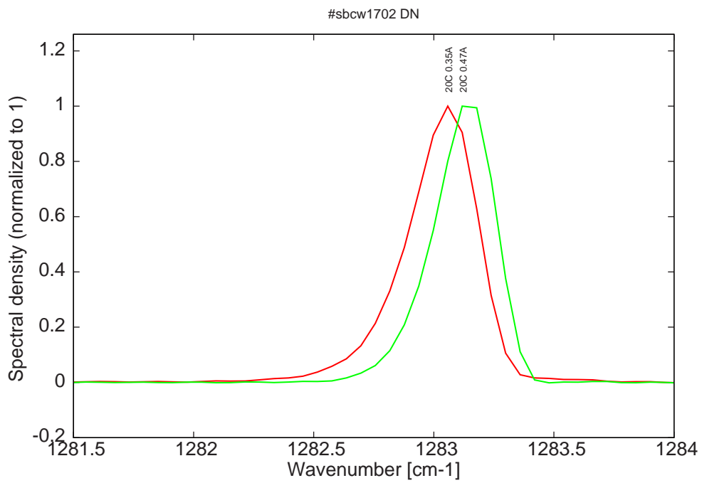
Figure 13: monomode spectra at 20C for various DC currents (with mode jumping for high currents)
