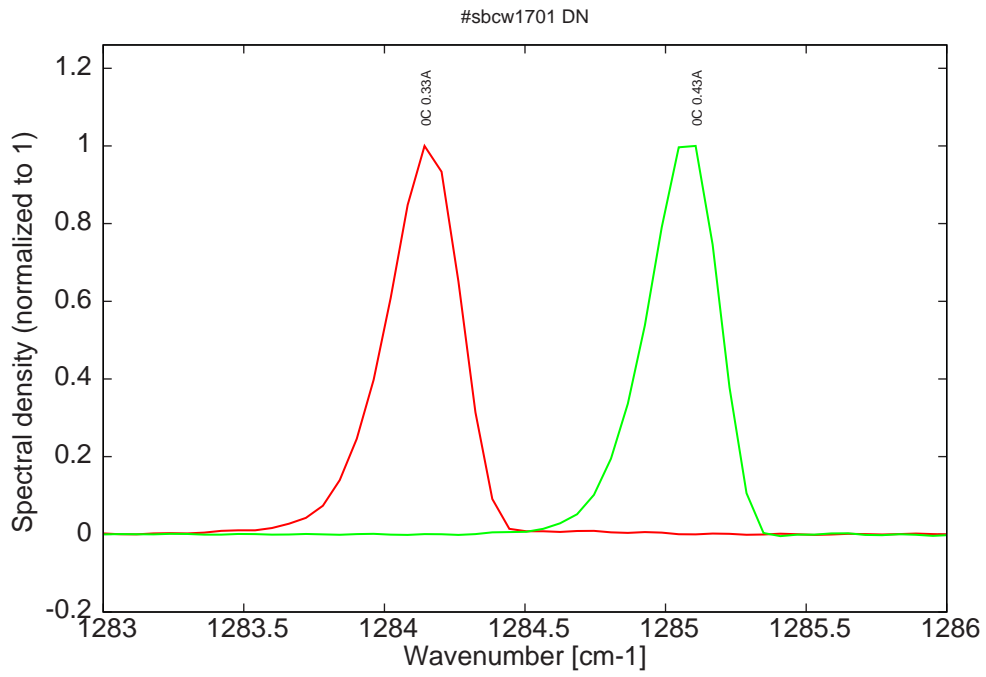
Figure 10: spectra at 0C for various DC currents (monomode range, but with mode jumping for current higher than 0.33A)
