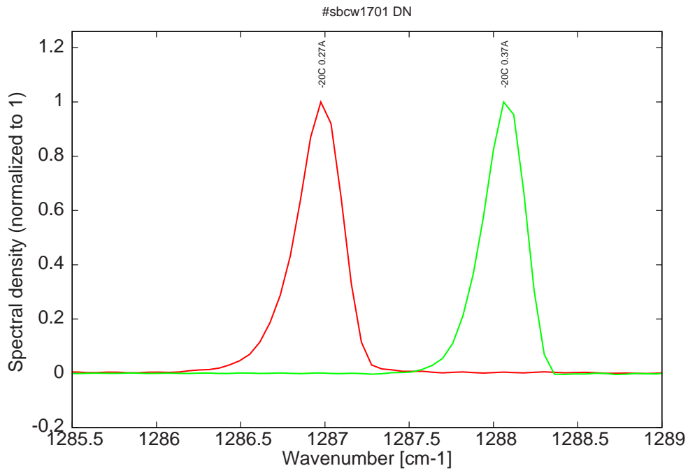
Figure 8: spectra at -20C for various DC currents (monomode range, but with mode jumping for current higher than 0.27A)
