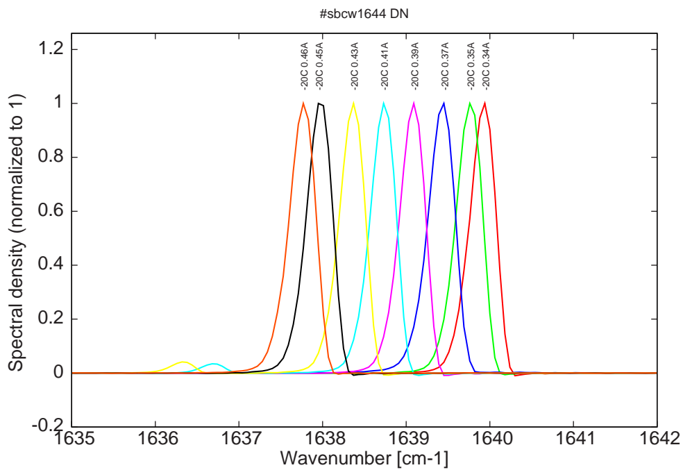
Figure 7: spectra at -20C for various DC currents (monomode up to 0.39A, then bimode, and again monomode for I > 0.43A )
