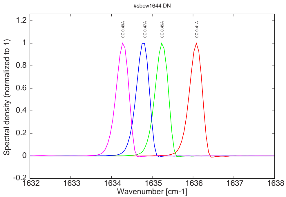
Figure 9: spectra at 0C for various DC currents (monomode up to 0.45A, then bimode)
