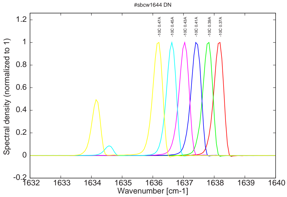
Figure 8: spectra at -10C for various DC currents (monomode up to 0.43A, then bimode)
