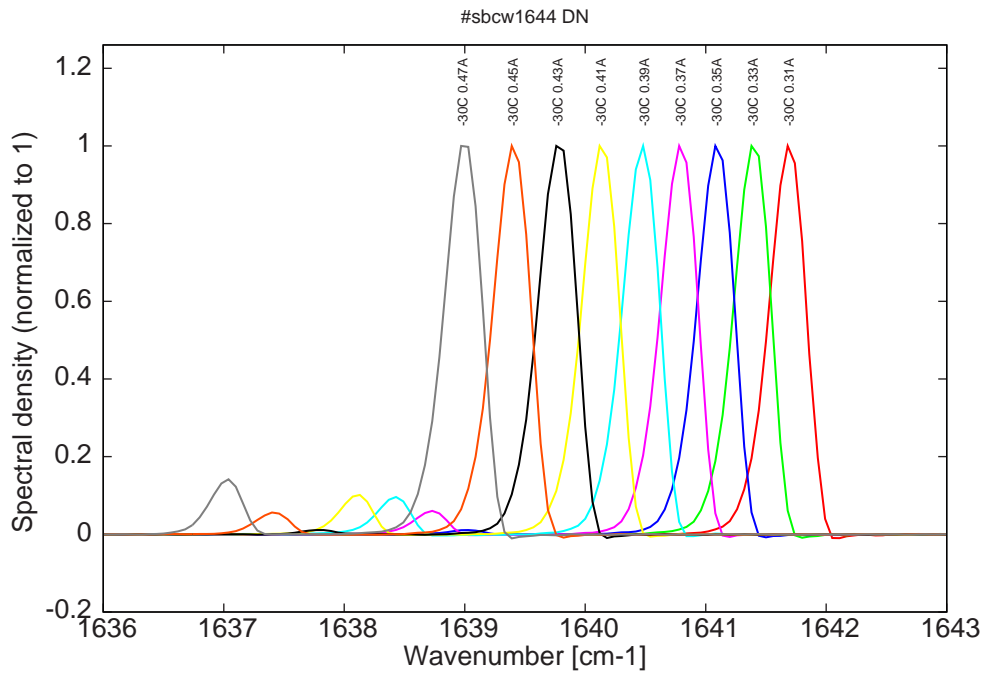
Figure 6: spectra at -30C for various DC currents (monomode up to 0.33A, then bimode)
