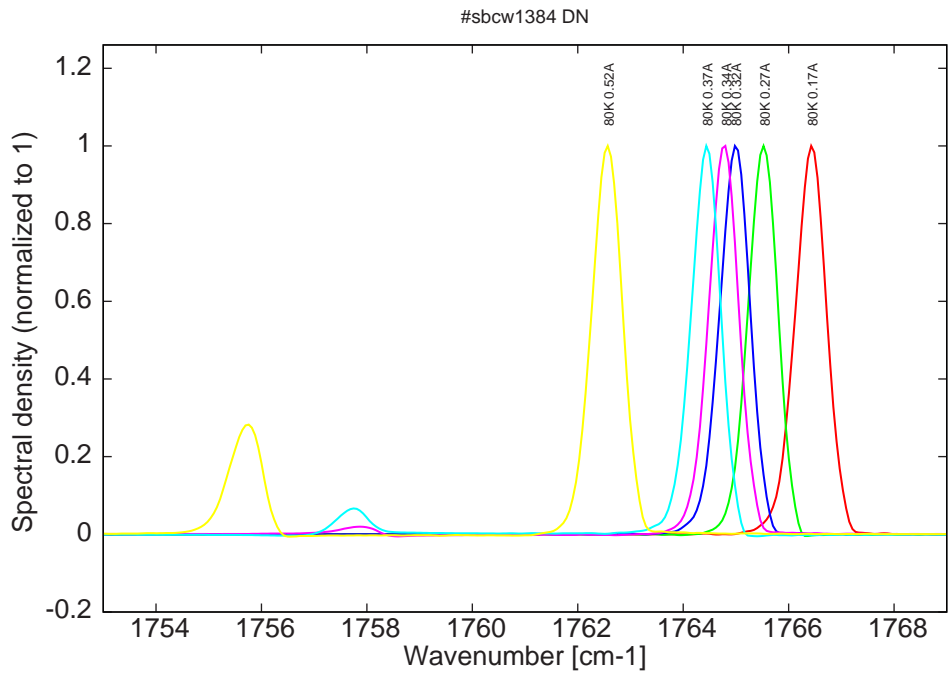
Figure 6: spectra at 80K for various DC currents (monomode up to 0.32A)
