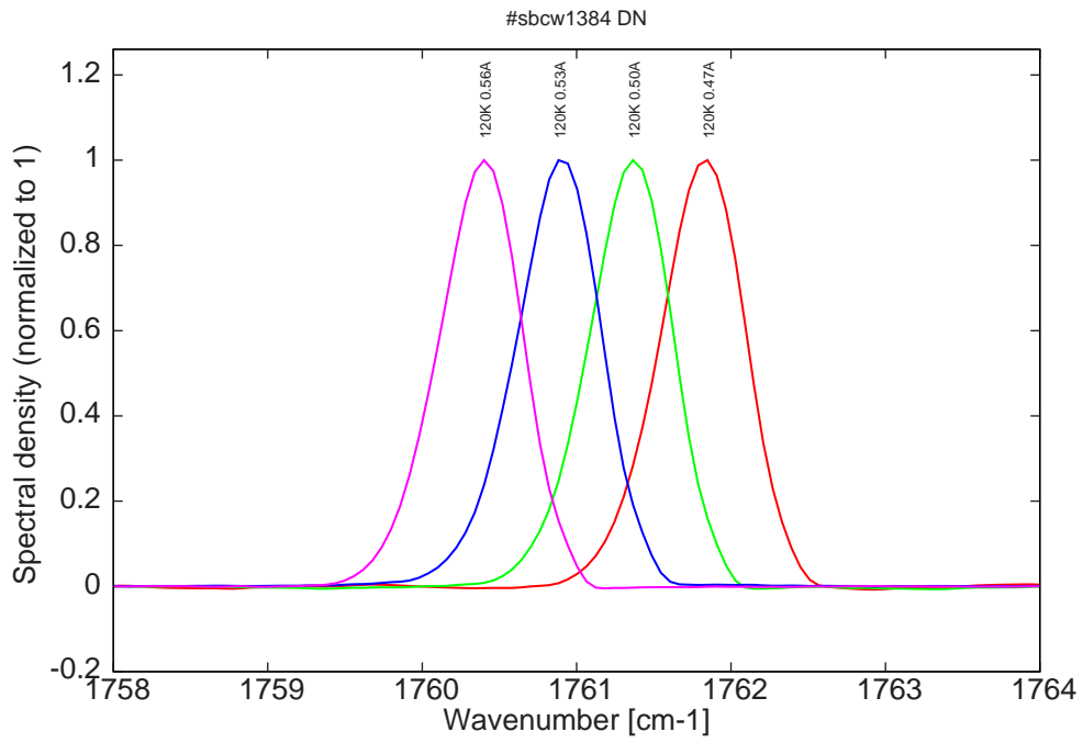
Figure 10: spectra at 120K for various DC currents (all monomode on a different mode compared to the other temperatures, see Fig. 1)
