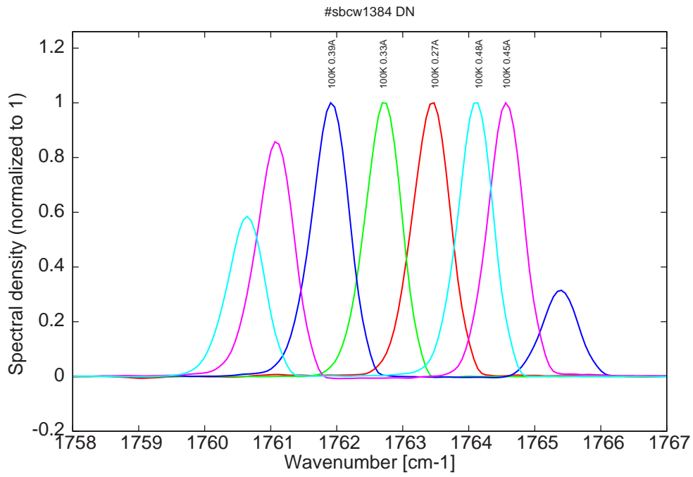
Figure 8: spectra at 100K for various DC currents (monomode up to 0.33A)
