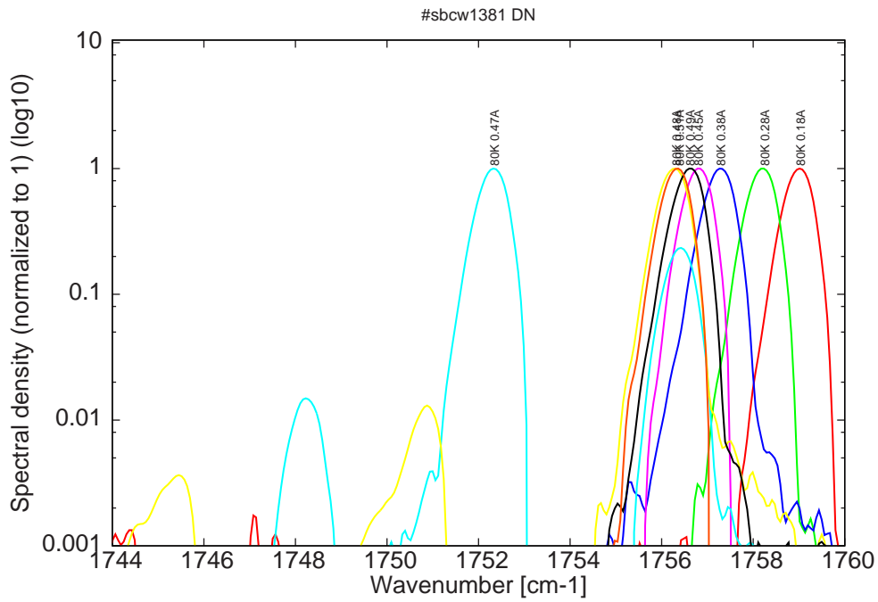
Figure 6: spectra at 80K for various DC currents (momomode for I < 0.45A and I > 0.49A , between trimode)
