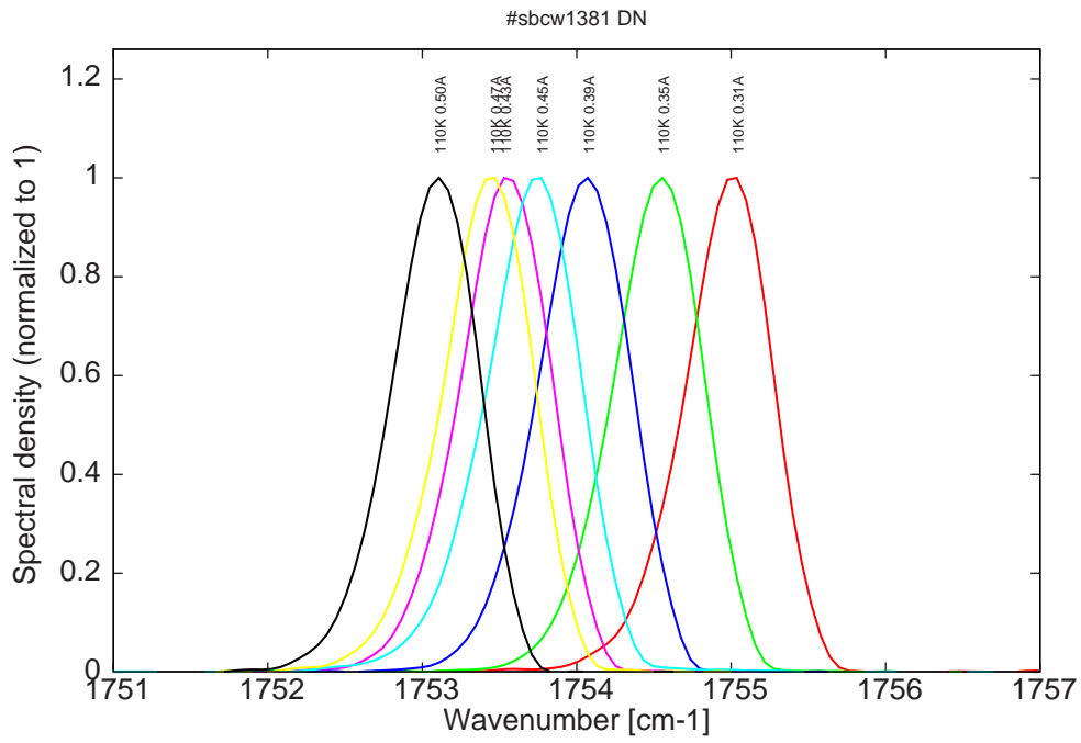
Figure 10: spectra at 110K for various DC currents (mode jumping for I > 0.43A , see Fig 1)
