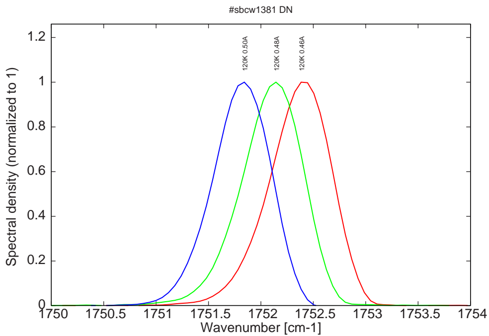
Figure 11: spectra at 120K for various DC currents (all monomode on the same mode as lower currents at lower temperatures, see Fig 1)
