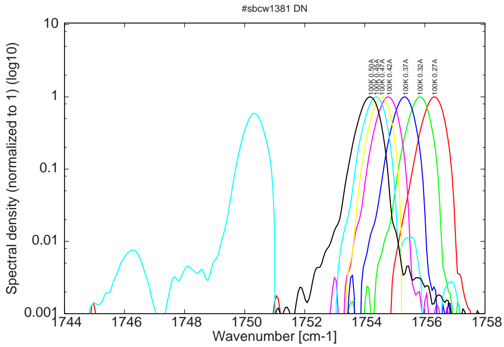
Figure 8: spectra at 100K for various DC currents (momomode for I < 0.42\text{A} and I > 0.47\text{A} , between trimode)
