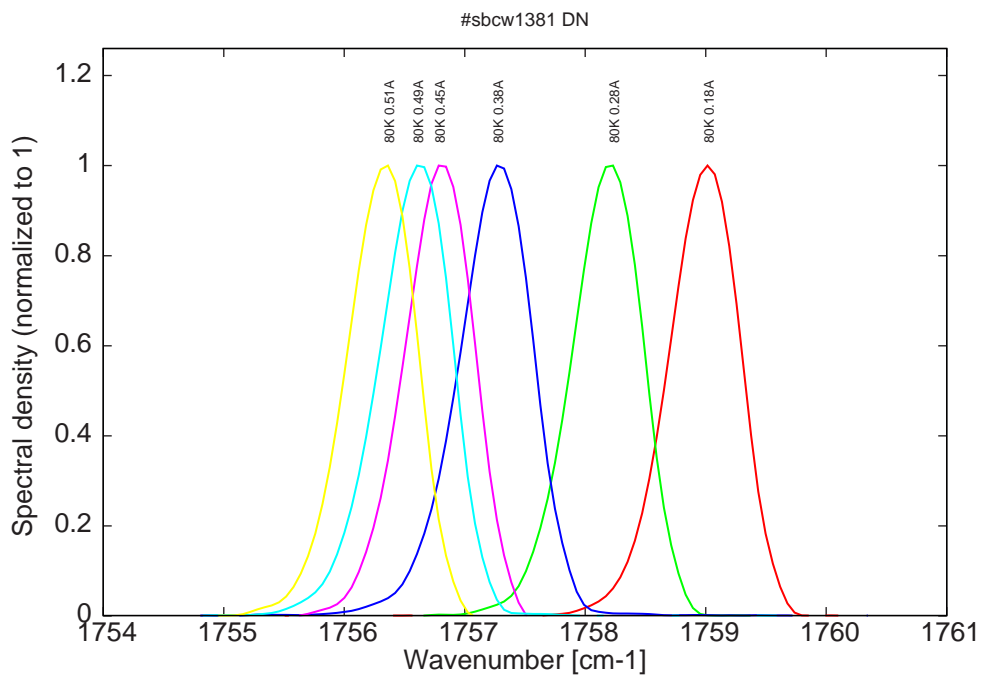
Figure 7: spectra at 80K for various DC currents (monomode range, mode jumping for I > 0.45A , see Fig 1)
