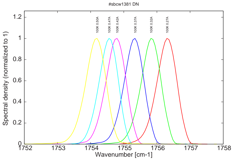
Figure 9: spectra at 100K for various DC currents (monomode range, mode jumping for I > 0.42\text{A} , see Fig 1)
