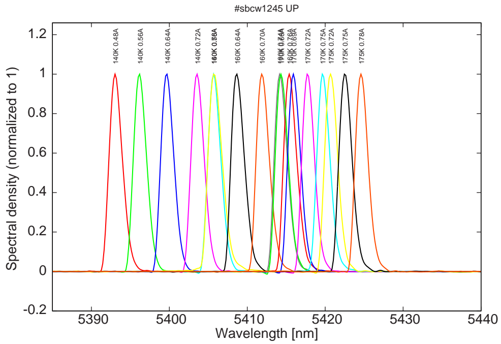
Figure 5: spectra at 140K, 160K, 170K and 175K
