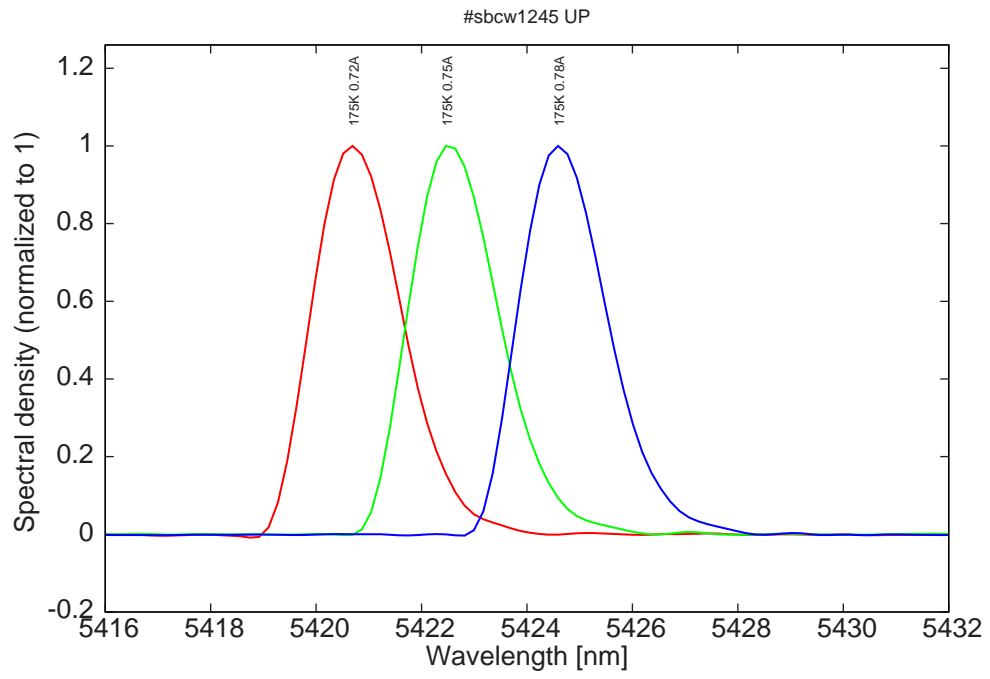
Figure 9: spectra at 175K
