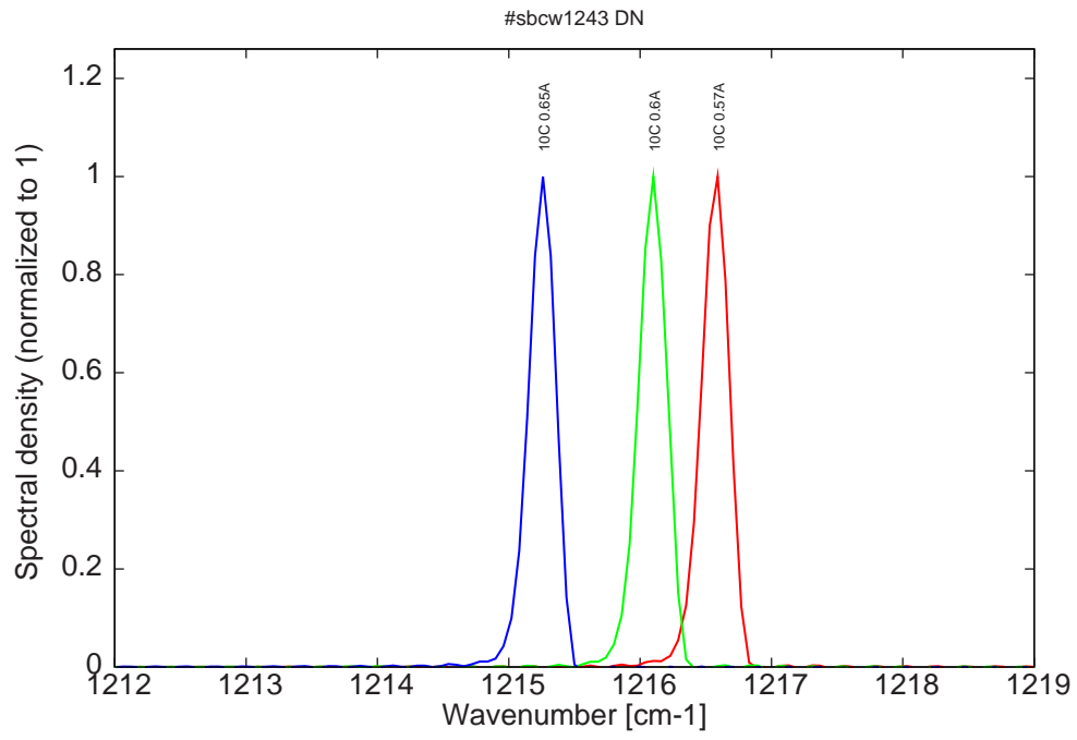
Figure 14: spectra at 10C for various DC currents (monomode up to I=0.65A )
