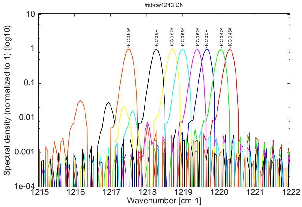
Figure 10: spectra at -10C for various DC currents (become bimode for I > 0.50A )
