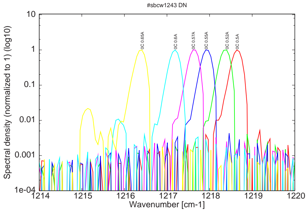
Figure 12: spectra at 0C for various DC currents (become bimode for I > 0.57A )
