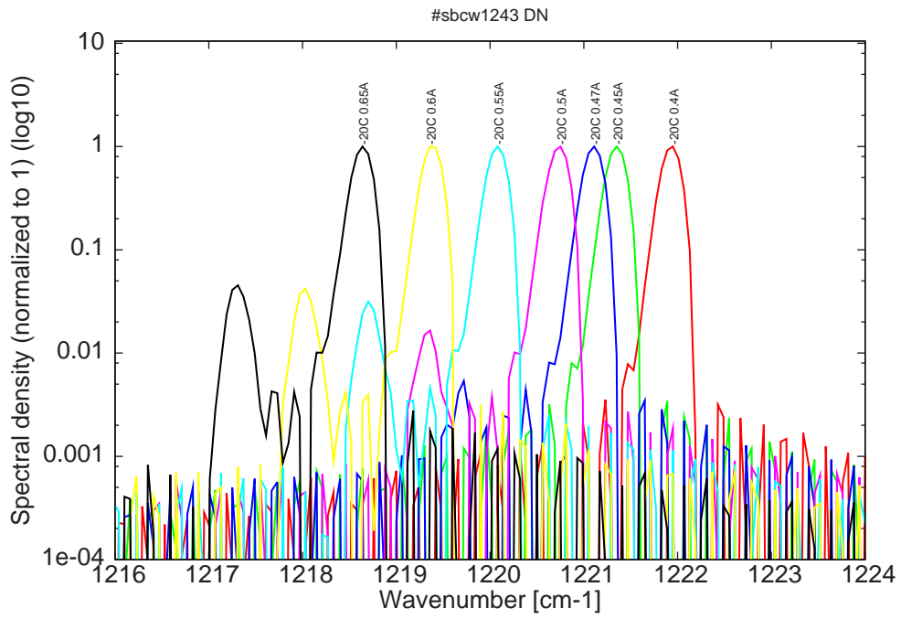
Figure 8: spectra at -20C for various DC currents (become bimode for I > 0.45A )
