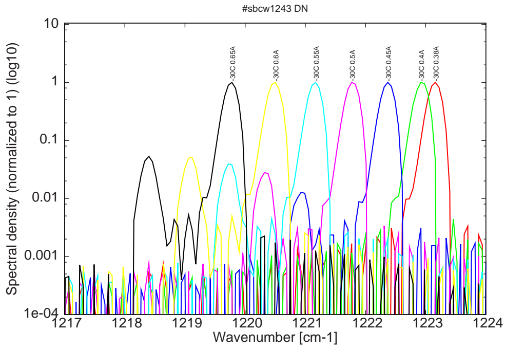
Figure 6: spectra at -30C for various DC currents (become bimode for I > 0.40A )
