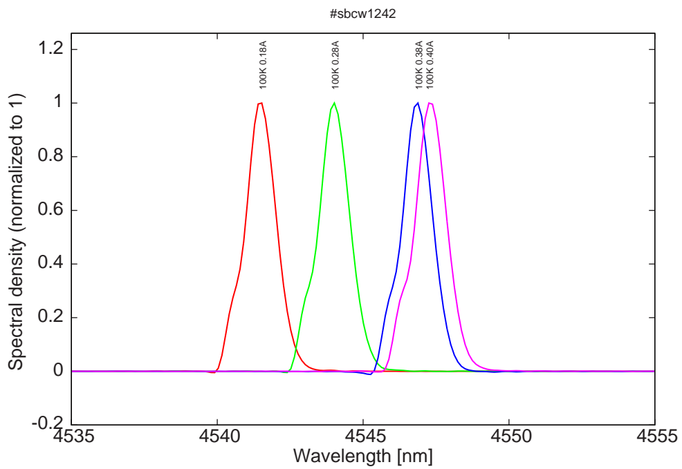
Figure 10: spectra at 100K (monomode range)
