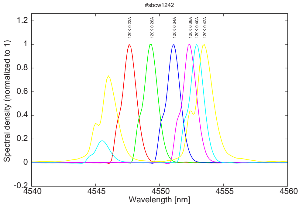
Figure 11: spectra at 120K
