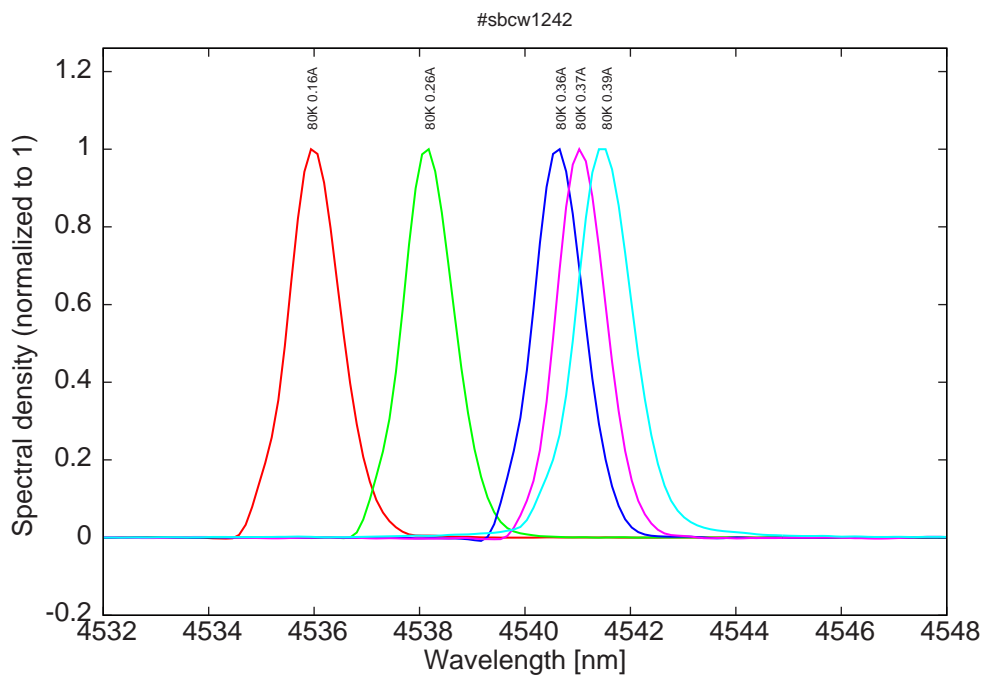
Figure 8: spectra at 80K (monomode range)
