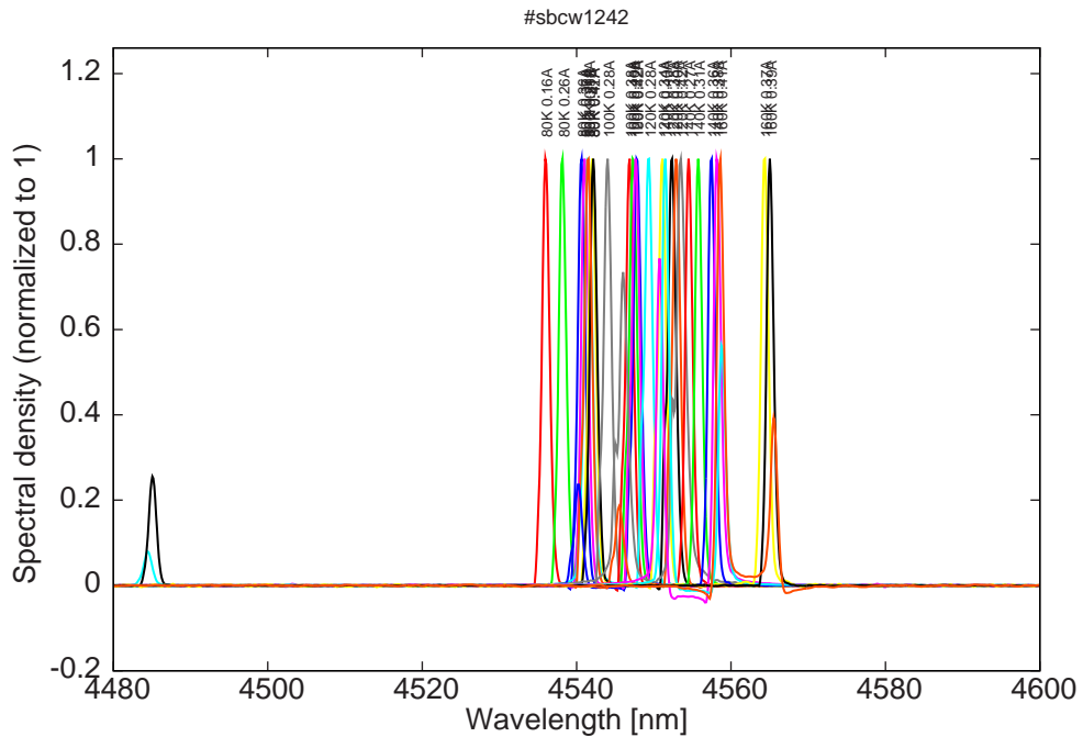
Figure 6: spectra at 80K, 90K, 100K, 120K and 140K
