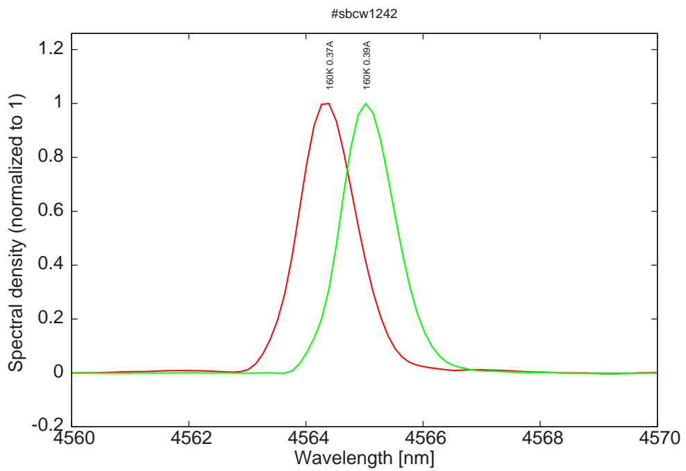
Figure 16: spectra at 160K (monomode range)
