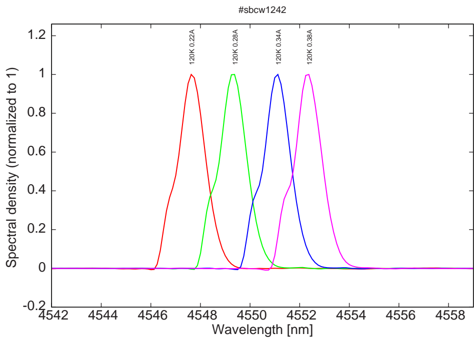
Figure 12: spectra at 120K (monomode range)
