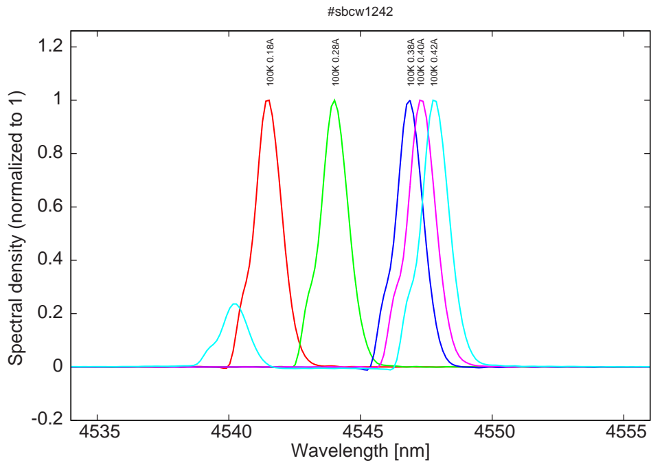
Figure 9: spectra at 100K
