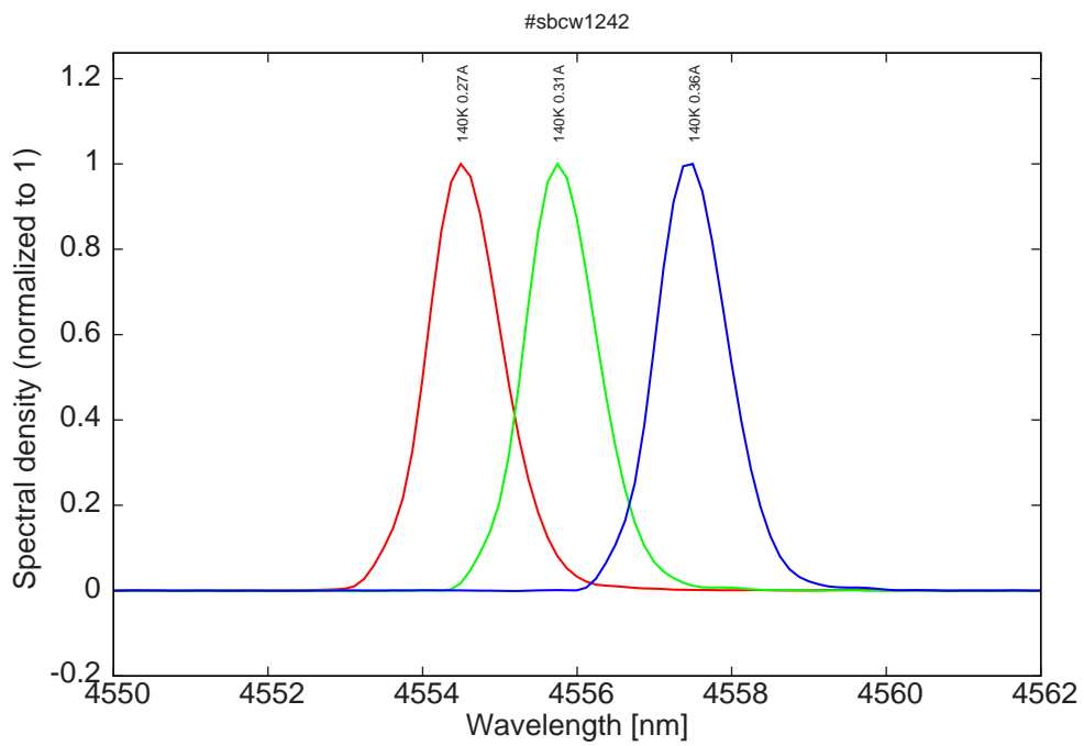
Figure 14: spectra at 140K (monomode range)
