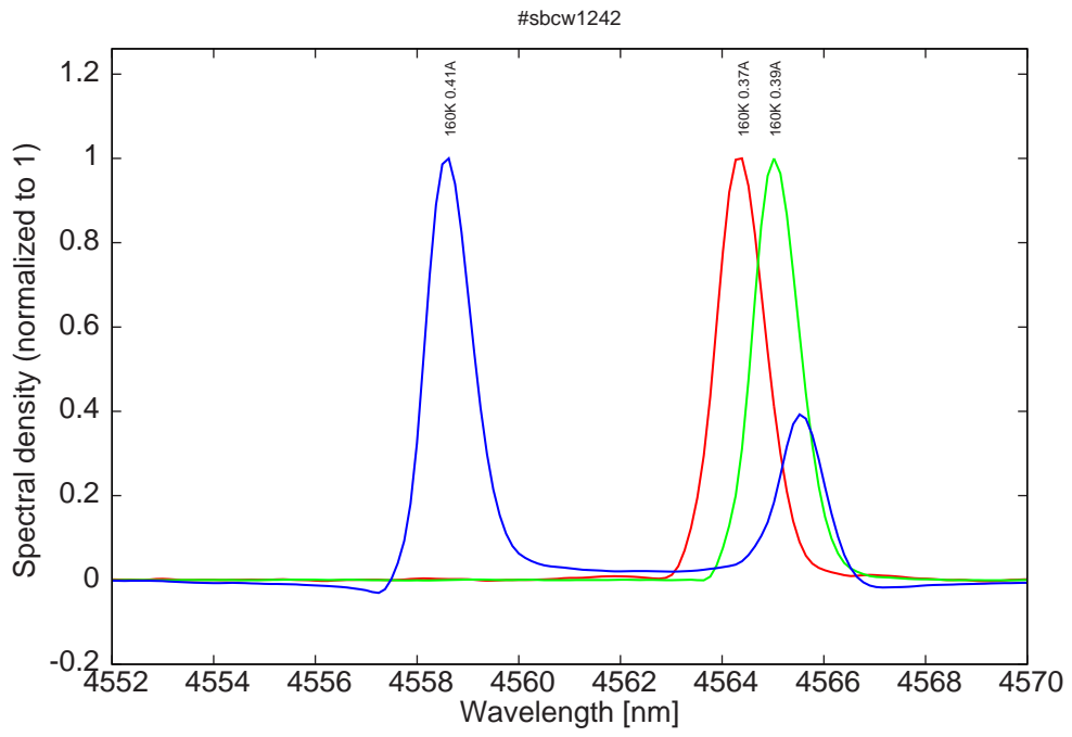
Figure 15: spectra at 160K
