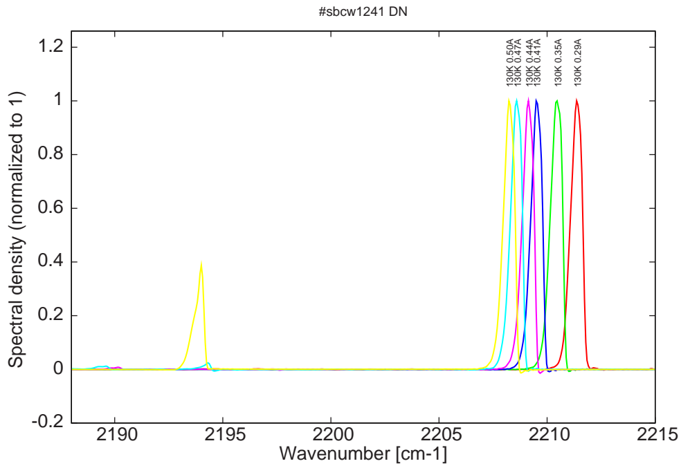
Figure 8: spectra at 130K
