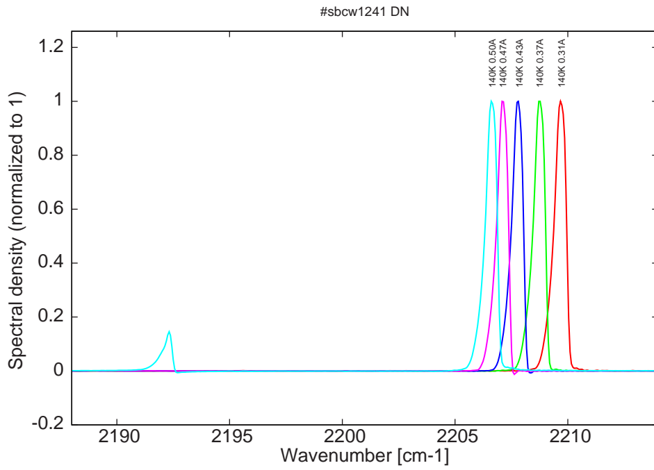
Figure 10: spectra at 140K
