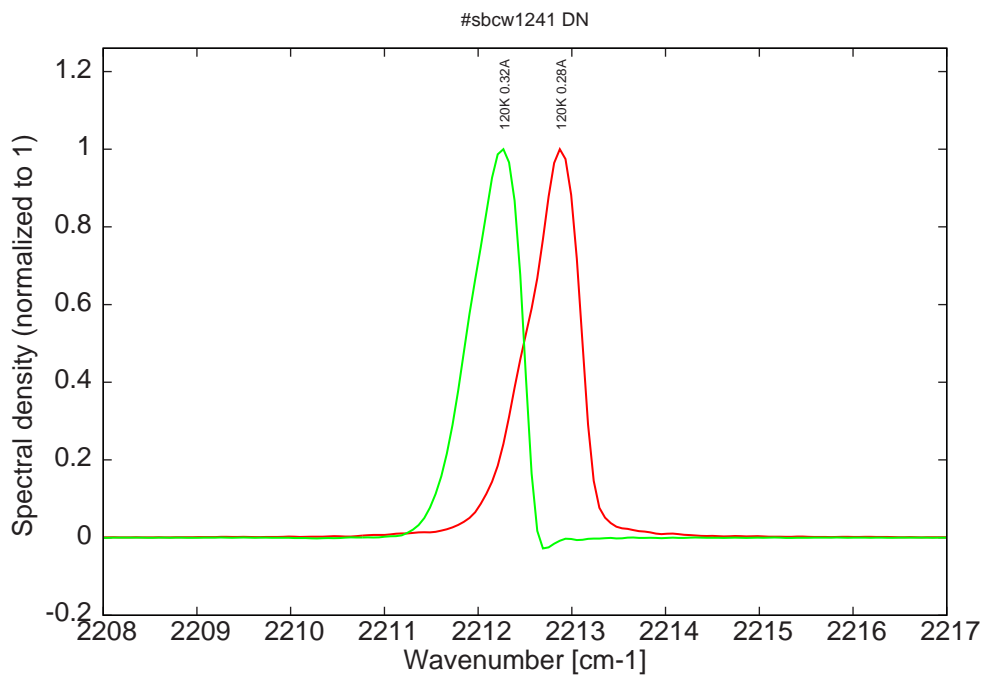
Figure 7: spectra at 120K (monomode range)
