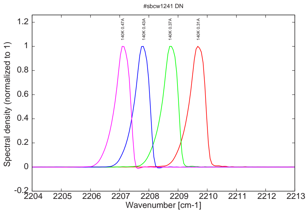
Figure 11: spectra at 140K (monomode range)
