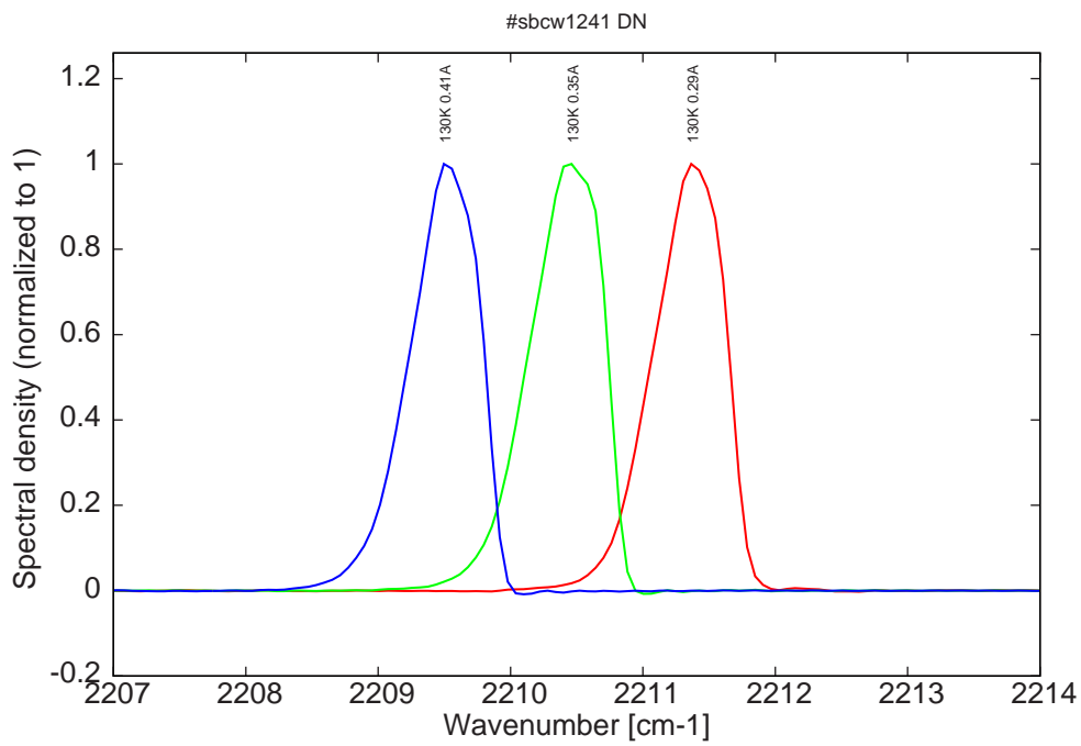
Figure 9: spectra at 130K (monomode range)
