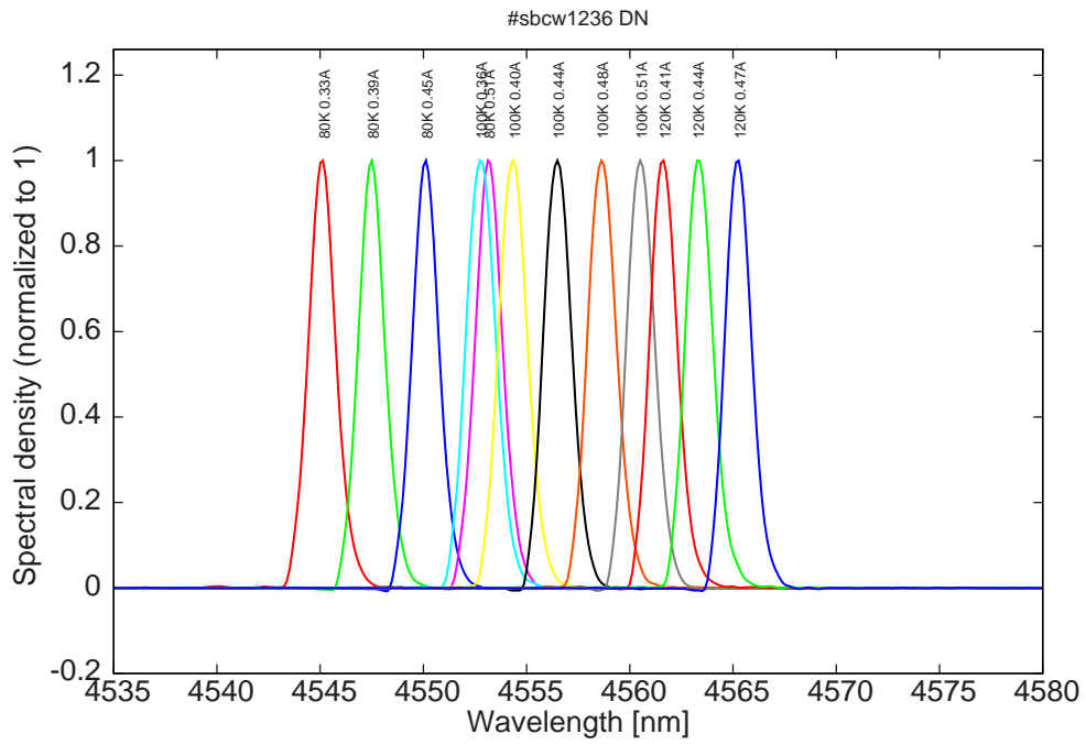
Figure 5: spectra at 80K, 100K, 120K, 140K, 160K and 180K
