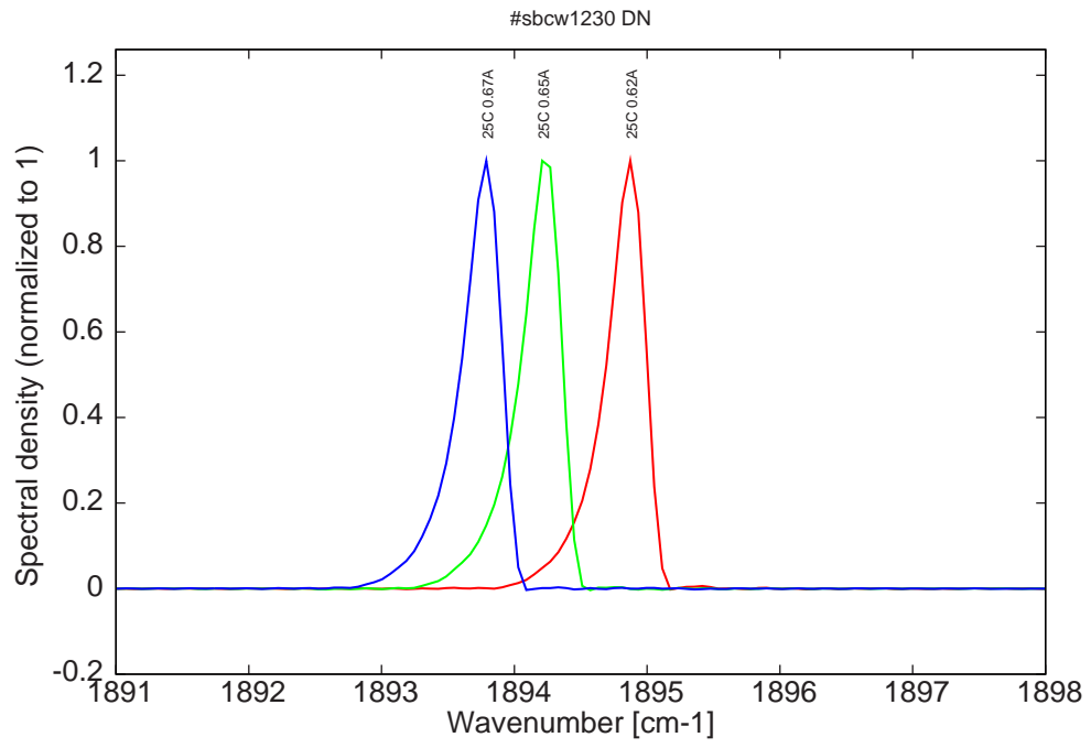
Figure 18: spectra at 25C for various DC currents (all monomode)
