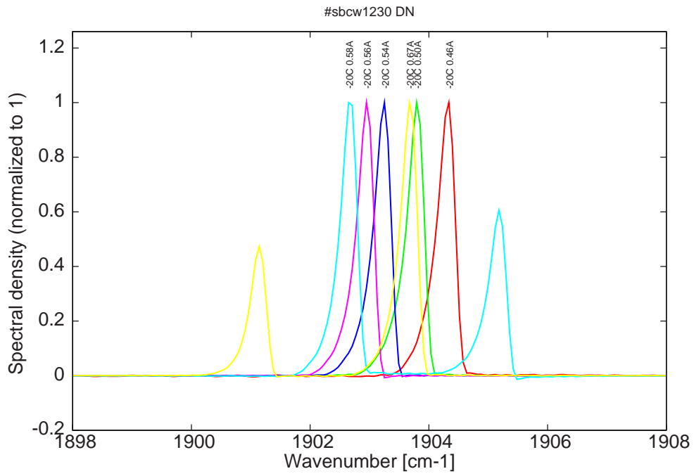
Figure 8: spectra at -20C for various DC currents (monomode up to 0.56A)
