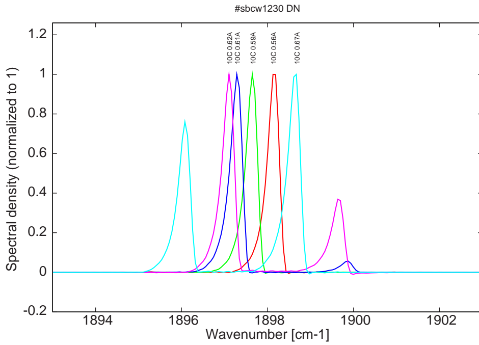
Figure 14: spectra at 10C for various DC currents (monomode up to 0.59A)
