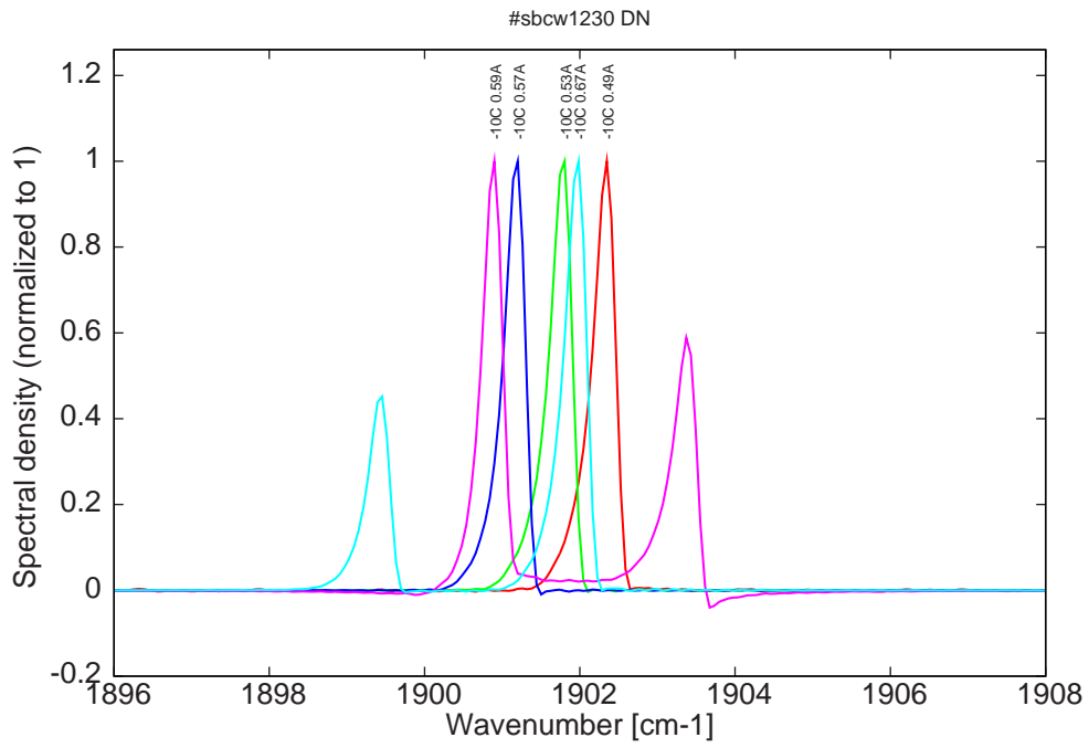
Figure 10: spectra at -10C for various DC currents (monomode up to 0.57A)
