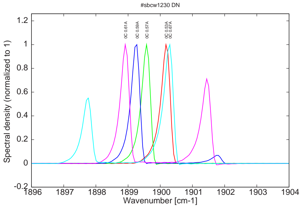
Figure 12: spectra at 0C for various DC currents (monomode up to 0.57A)
