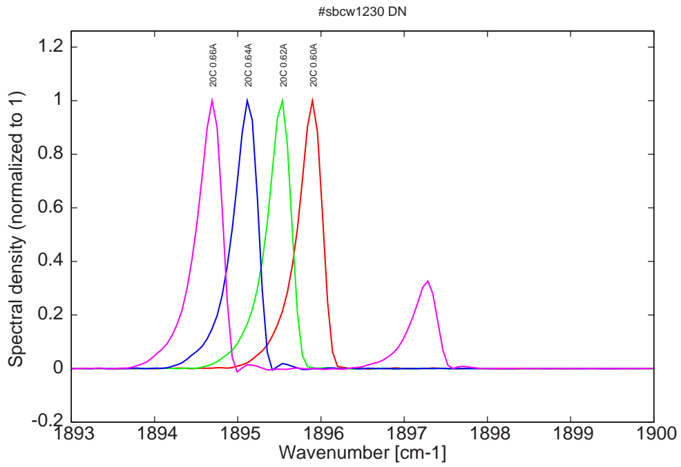
Figure 16: spectra at 20C for various DC currents (monomode up to 0.64A)
