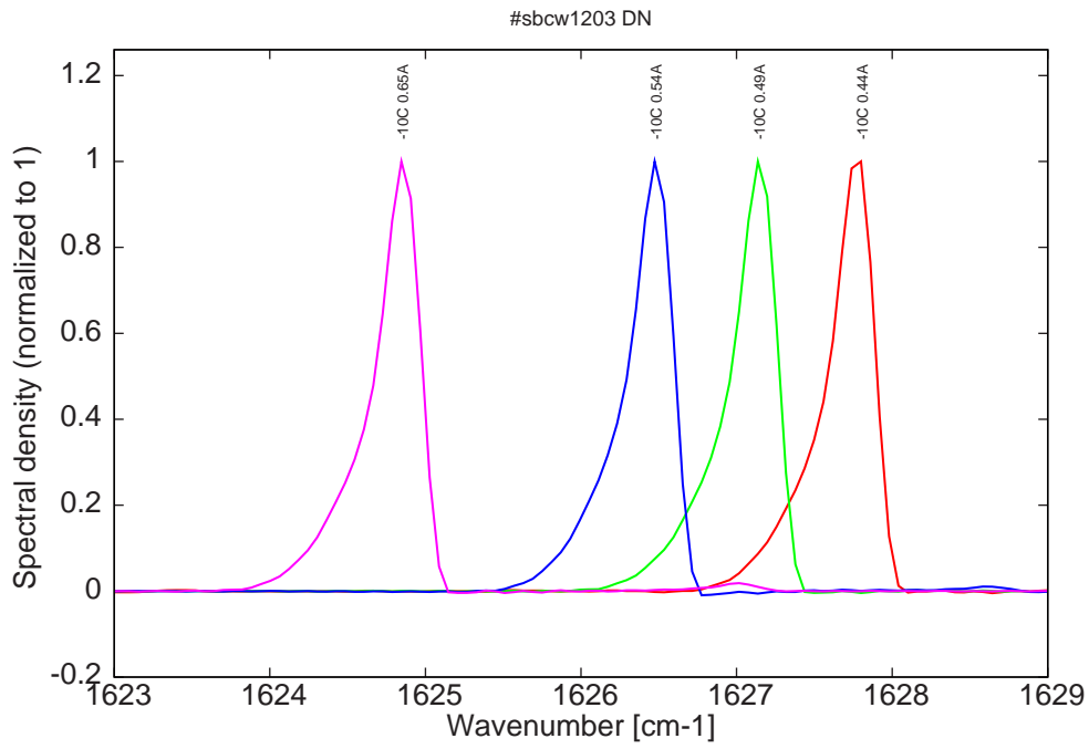
Figure 10: spectra at -10C for various DC currents (monomode up to 0.49A)
