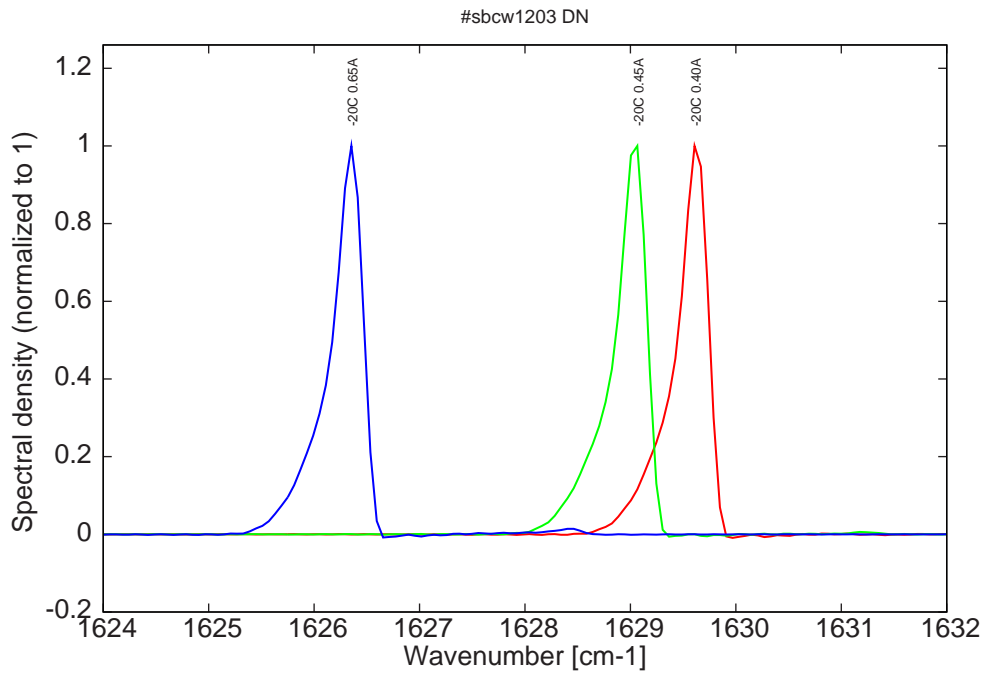
Figure 8: spectra at -20C for various DC currents (monomode only at threshold)
