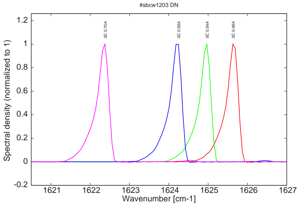
Figure 12: spectra at 0C for various DC currents (monomode up to 0.54A)
