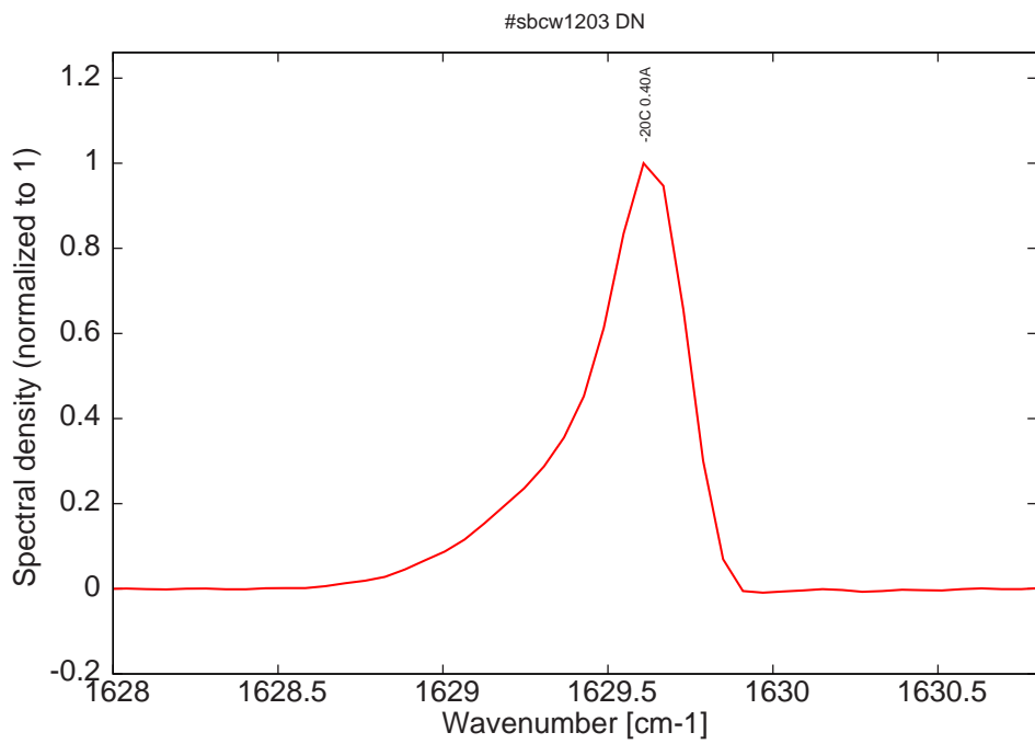
Figure 9: monomode spectrum at -20C and 0.40A
